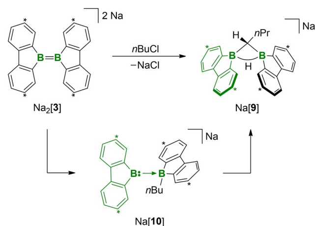
Scheme 8. The diborane(4)-dianion salt Na_2[3] and n BuCl generate Na[9] in a B-Cl substitution/C-H activation sequence. A borafluorenyl-anion adduct Na[10] is proposed as the intermediate (carbon atoms marked with asterisks bear t Bu substituents).
