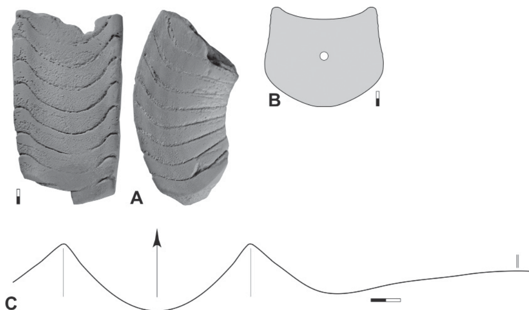
Fig. 8. Stroborinecerus felis gen. et sp. nov., holotype MB.C.30454 (Korn et al. 2002 Coll.) from Oued Temertasset. A. Ventral and lateral views. B. Whorl profile. C. Suture line, at ww=15.6 mm, wh=12.7 mm. Scale bar units=1 mm.
