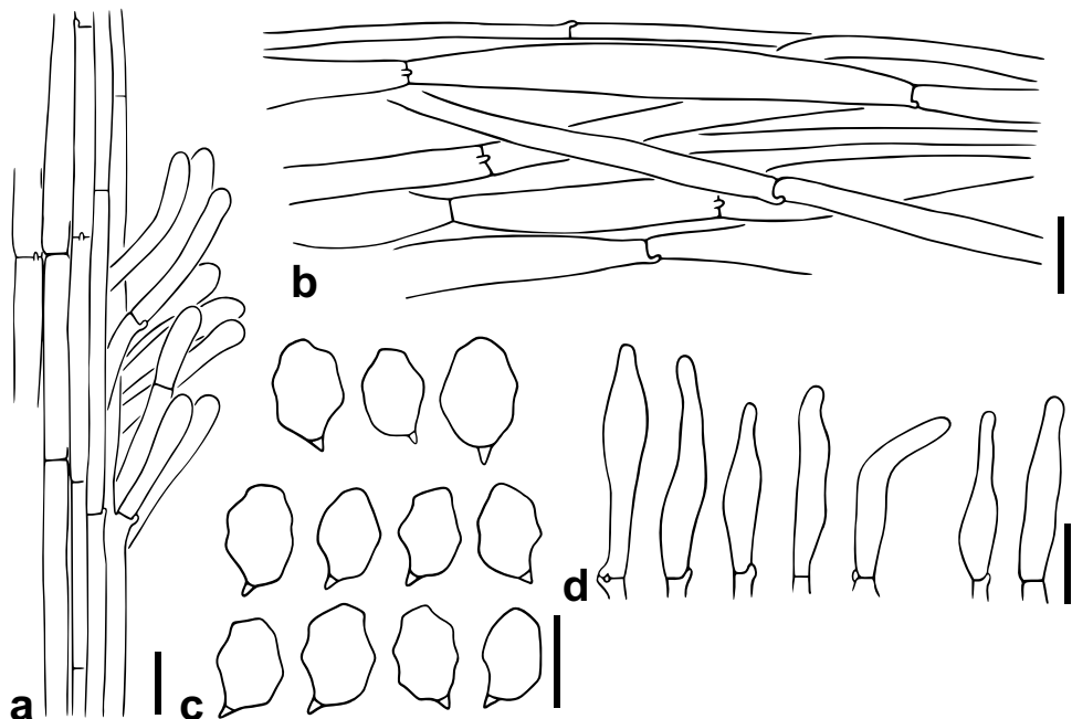
Fig. 27 Microscopic structures of Entoloma confusissimum (KaiR670, holotype): a stipitipellis with caulocystidia, bar = 20 \mu m; b pileipellis, bar = 20 \mu m; c basidiospores, bar = 10 \mu m; d cheilocystidia, bar = 20 \mu m
