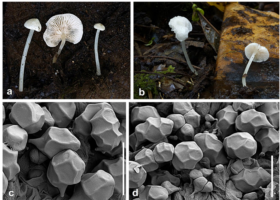
Fig. 26 Basidiocarps and basidiospores as seen by SEM of Entoloma confusissimum : a (KaiR489); b, c, d (KaiR670, holotype) bars = 10 \mu m
