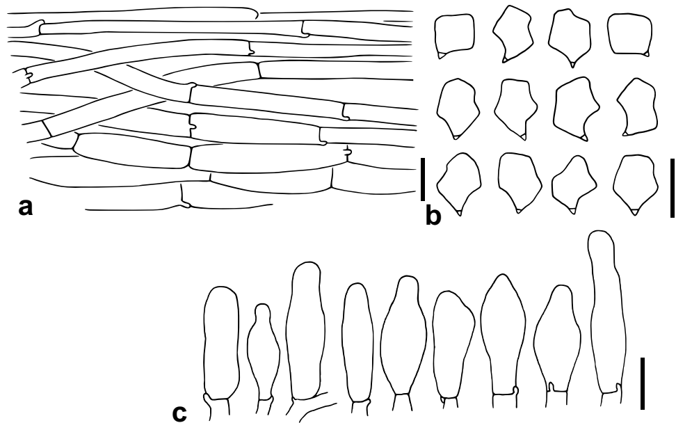
Fig. 25 Microscopic structures of Entoloma amistadosericulum (KaiR612, holotype): a pileipellis, bar = 20 \mu m; b basidiospores, bar = 10 \mu m; c cheilocystidia, bar = 20 \mu m
