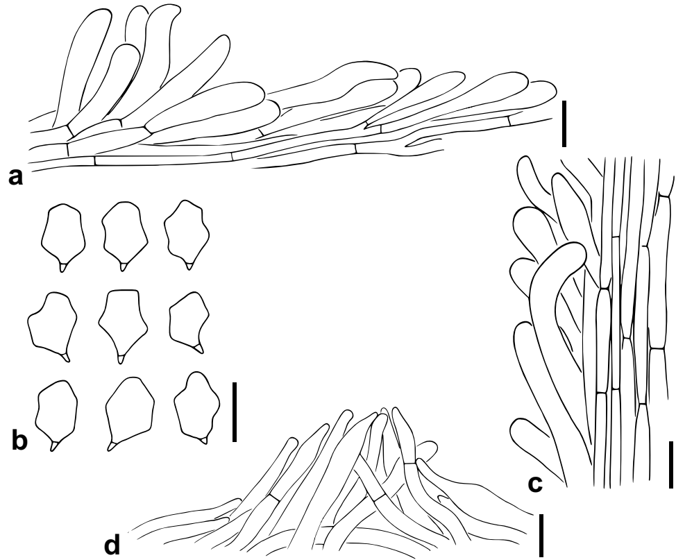
Fig. 34 Microscopic structures of Entoloma caeruleomarginatum (KaiR535, holotype): a pileipellis, bar = 20 \mu\text{m} ; b basidiospores, bar = 10 \mu\text{m} ; c stipitipellis, bar = 20 \mu\text{m} ; d cheilocystidia, bar = 20 \mu\text{m}
