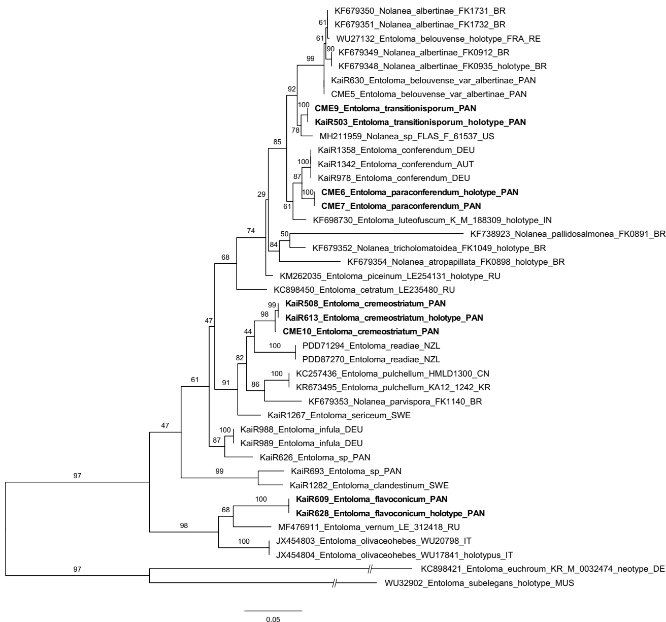
Fig. 12 Maximum Likelihood phylogram of species of subg. Nolanea based on ITS, rooted to E. subelegans and E. euchroum , bootstrap values above or below branches, bar = estimated changes/nucleotide
