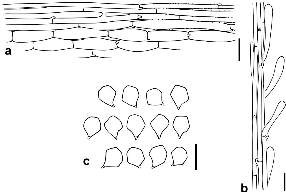
Fig. 11 Microscopic structures of Entoloma pruinosum (KaiR533, holotype): a pileipellis with incrusting pigment indicated at the right hand side, bar = 20 \mu m; b stipitipellis with caulocystidia, bar = 20 \mu m; c basidiospores, bar = 10 \mu m
