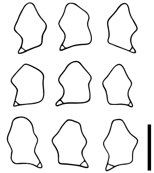
Fig. 14 Basidiospores of Entoloma belouvense var. albertinae (KaiR630), bar = 10\ \mu\text{m}
