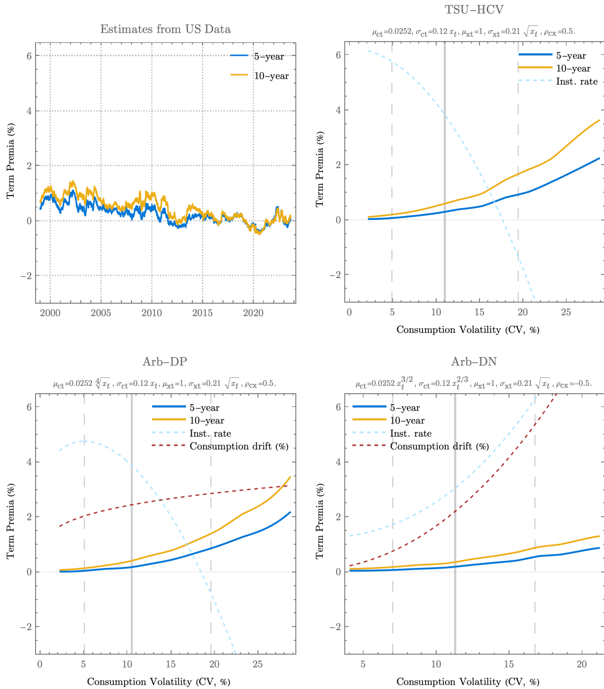
Figure 6: Term Premia in models with Time-Separable Utility and High consumption volatility
