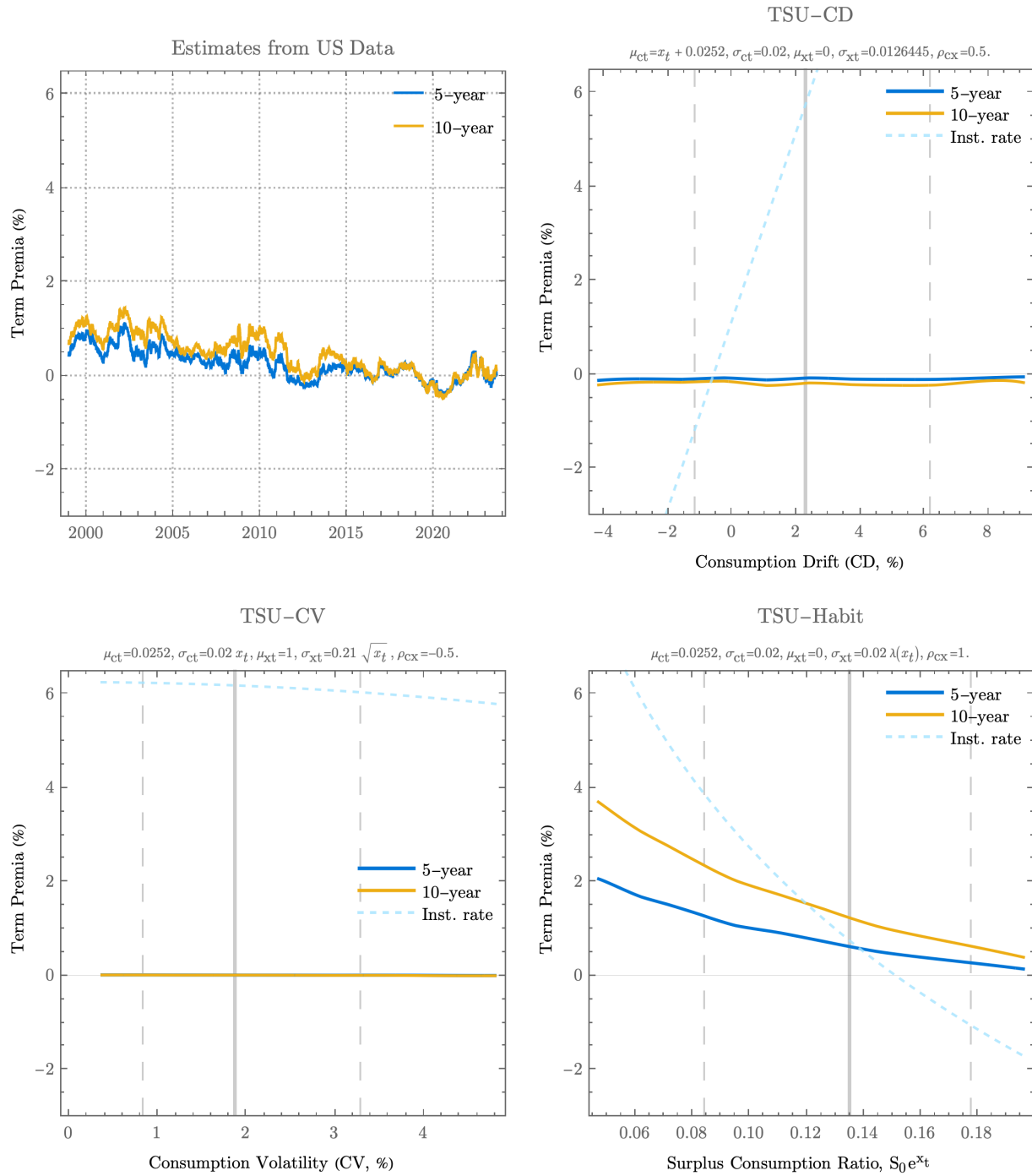
Figure 3: Term Premia in standard models with Time-Separable Utility The top left plot shows estimates of term premia according to d 'Amico et al. (2018). The remaining plots show state-dependent term premia for three standard variations, namely variations with a) time-varying CD, b) time-varying CV, and c) an external habit in the utility function respectively. The dashed line shows the short-term rate. The vertical dashed lines correspond to the typical values of the state variable based on simulations. The full range of the x -axis includes extreme values of the state variable, which are still possible (see Appendix D or Figure 16 for the exact definition of the ranges).
