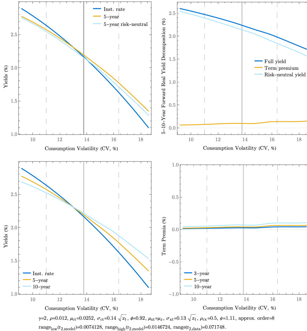
Figure 51: See Figure 16 for more details about the plots.
