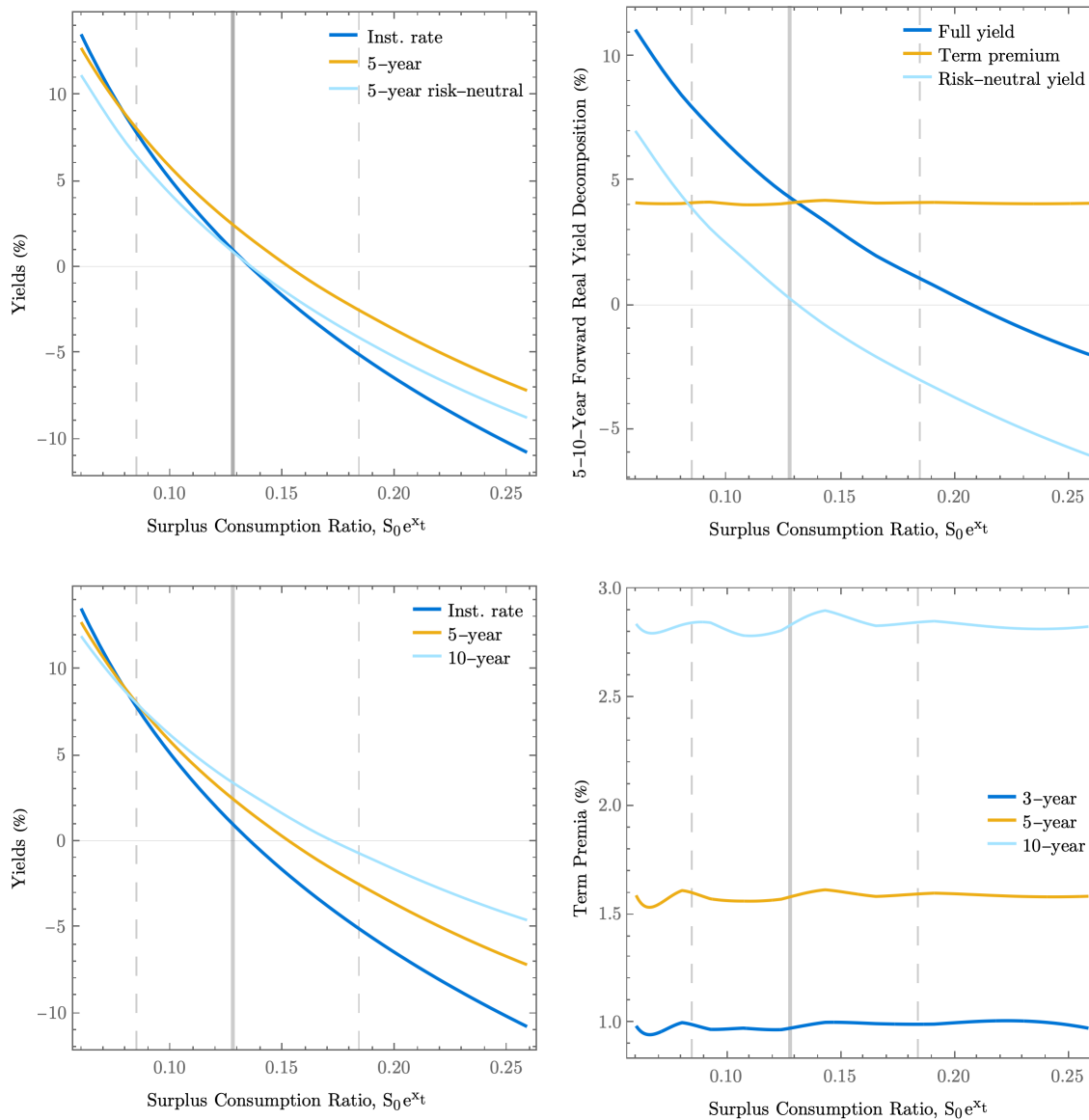
Figure 35: Time-varying extranl habit with time-separable utility and constant state variable volatility.
