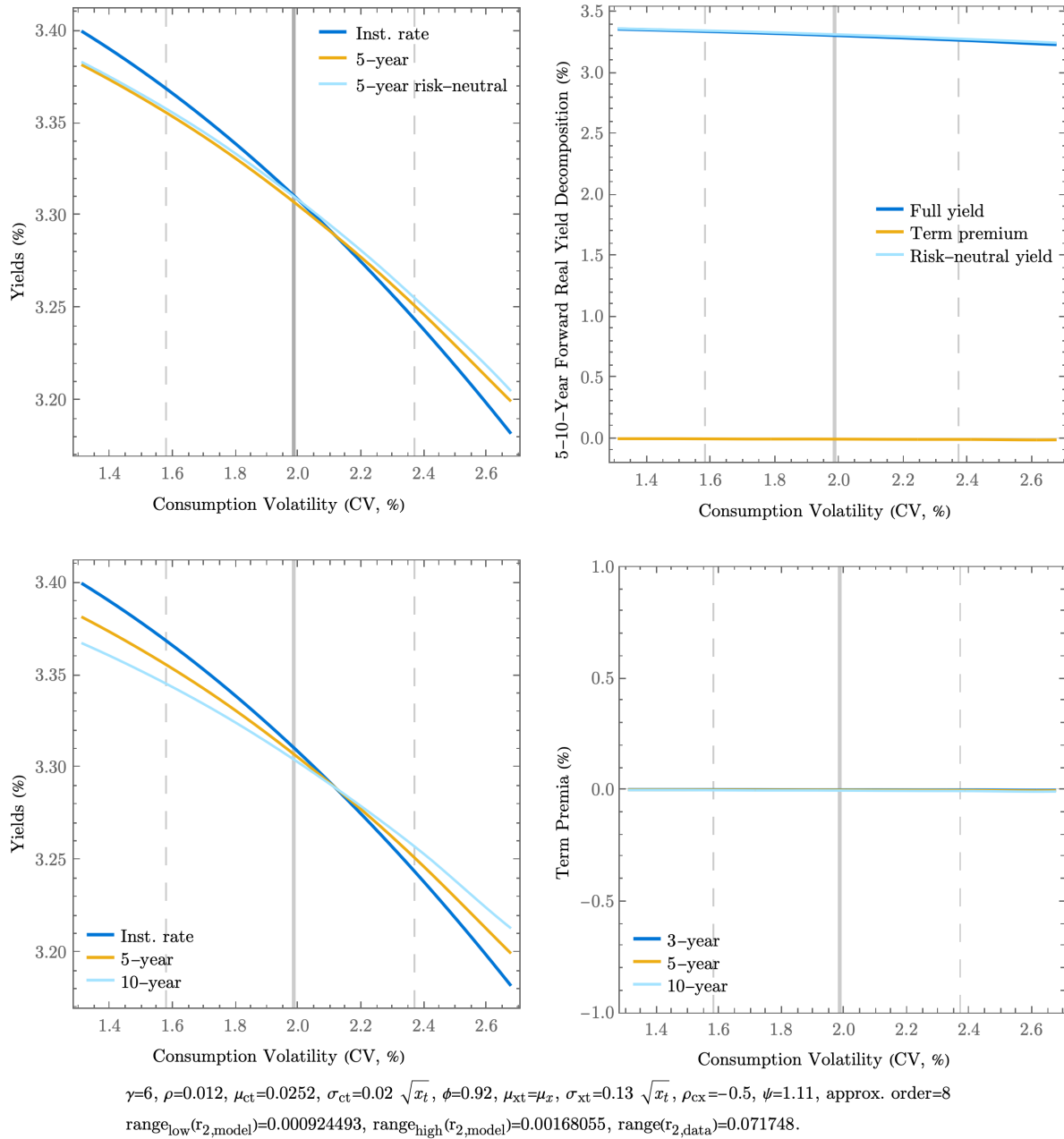
Figure 47: Time-varying consumption volatility with recursive utility and high risk aversion.
