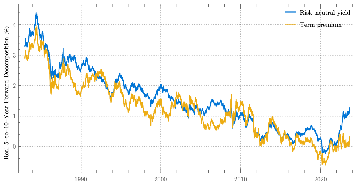
Figure 15: Time series of the forward 5-to-10 term premium for the US. ( back to text )
