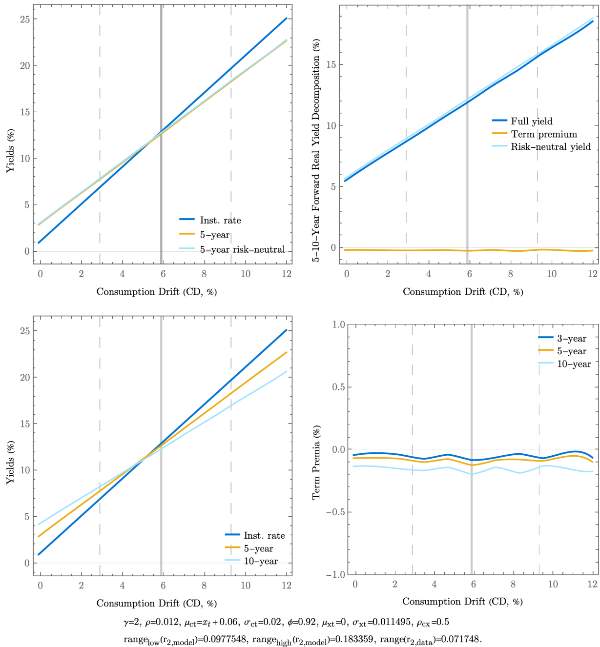
Figure 21: Time-varying and high consumption drift with time-separable utility. See Figure 16 for more details about the plots.
