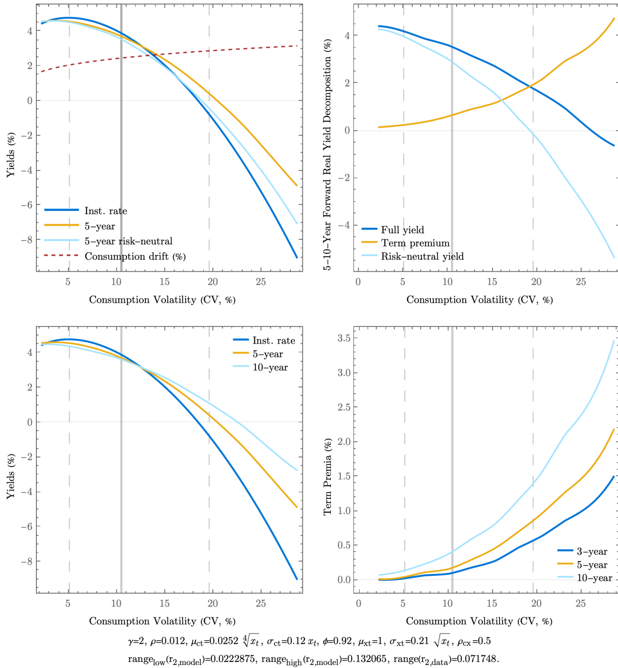
Figure 28: Both time-varying consumption drift and consumption volatility with time-separable utility, short-term rate decreasing in consumption volatility and positive \rho_{xc} . See Figure 6 for more details about the plots.
