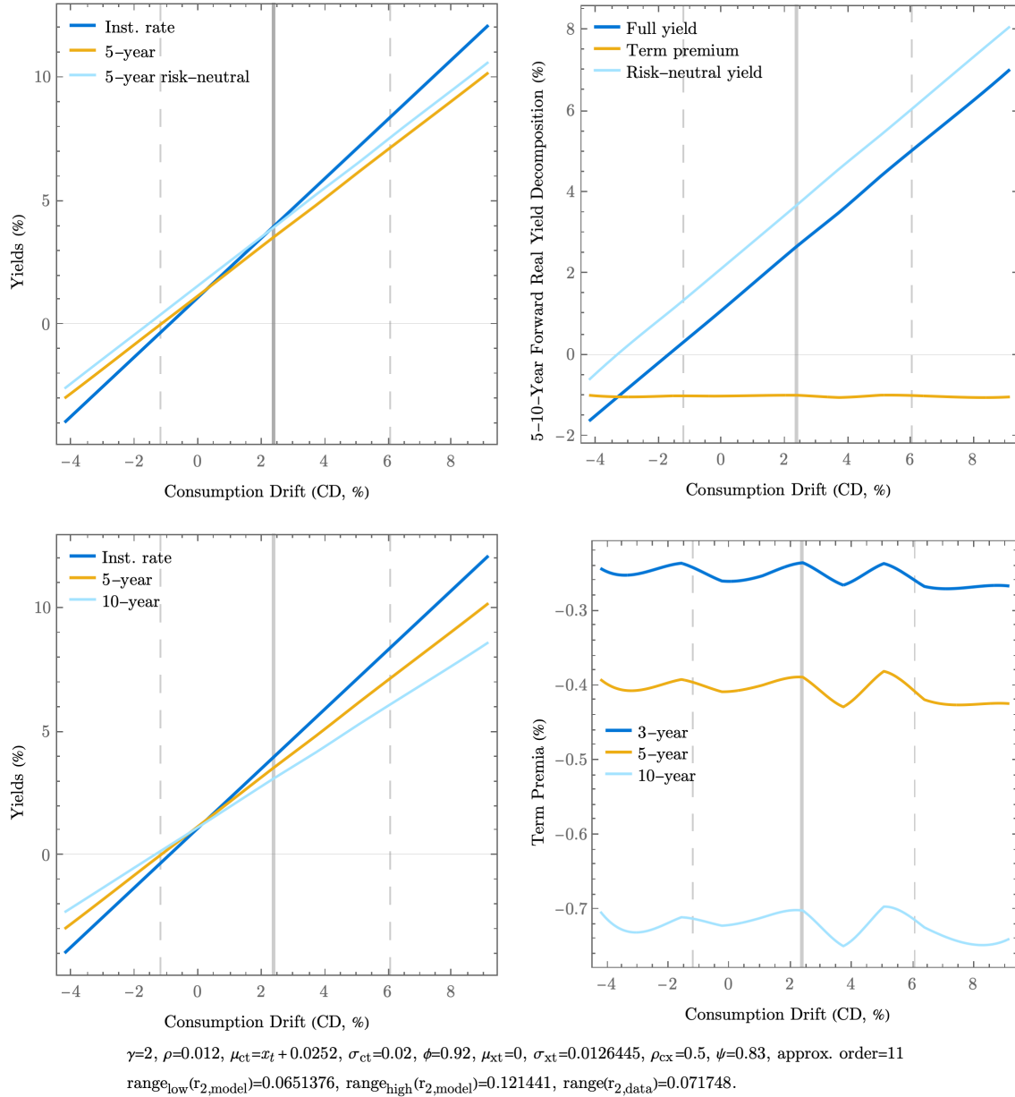
Figure 39: Time-varying consumption drift with recursive utility with low intertemporal elasticity of substitution.
