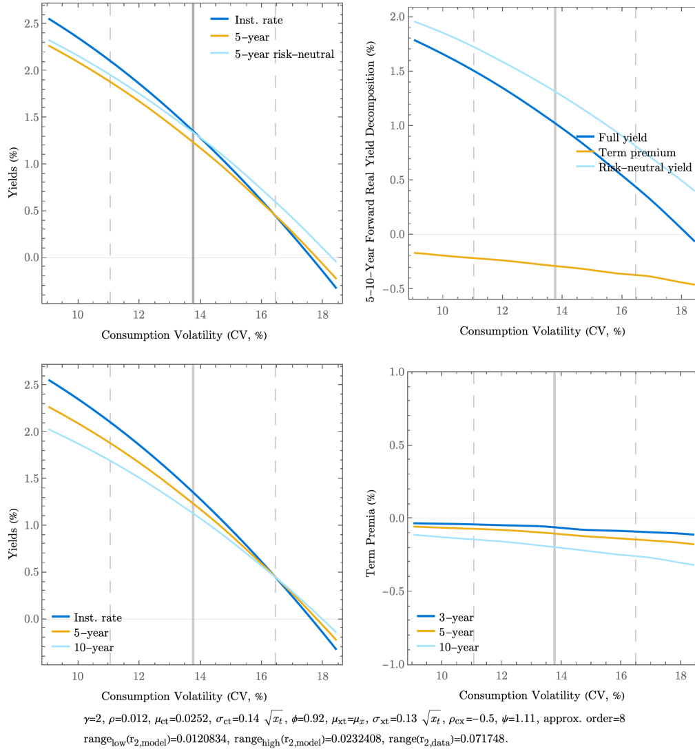
Figure 52: See Figure 16 for more details about the plots.
