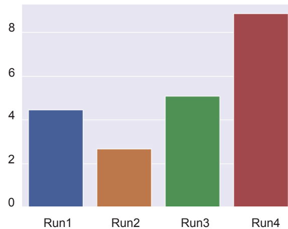
Total Gigabases
