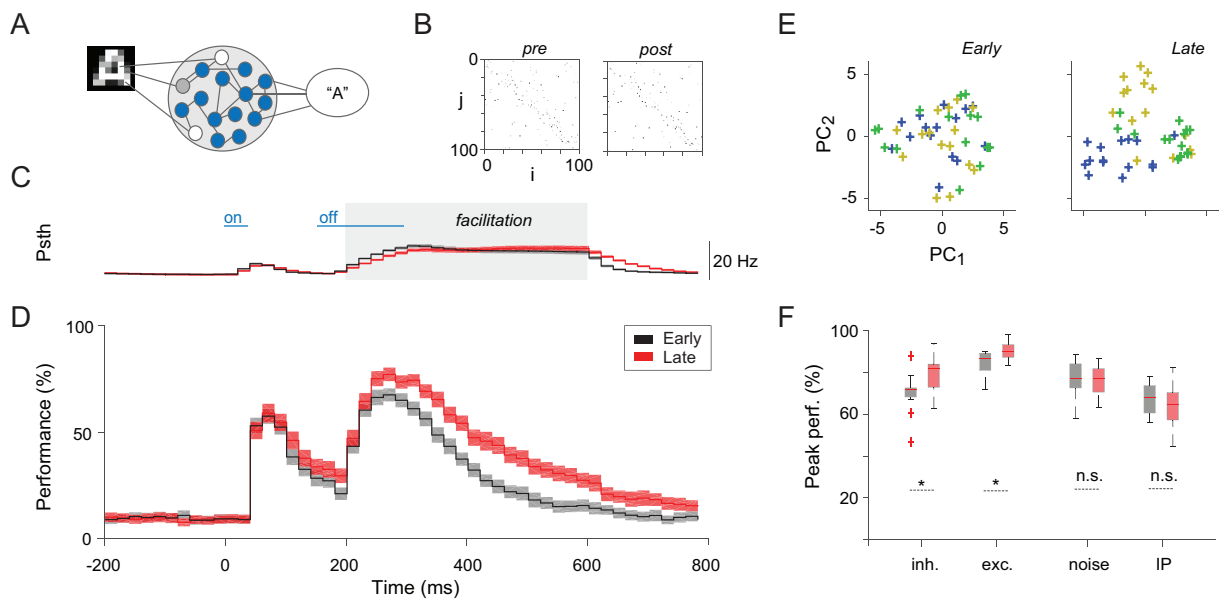
Fig. 6. Self-organizing recurrent network (SORN). A) Recurrent neural network with subset of neurons receiving pixel luminance inputs. B) Network topology: initial connections are sparse and random with nearby connections more likely to occur. Example of connections between 100 excitatory units out of the 200 total, before and after learning in one simulation. Visual exposure resulted in self-organized changes in synaptic gains. C) Example of network excitatory response to a brief stimulus. Response facilitation, implemented here through a decrease in synaptic inhibition, is marked by gray area. D) Example of classification performance improvement with stimulus exposure via unsupervised local plasticity rules (shaded areas indicate standard errors from the mean across 10 simulation). Note that here the firing rates are similar in early and late trials, due to the homeostatic nature of intrinsic plasticity, thus the enhancement in encoding comes from a reorganization of internal network dynamics. E) Exposure results in an enhanced clustering of trials belonging to different stimulus conditions in a low-dimensional projection space. F) Facilitation can boost or impede unsupervised learning depending on implementation. Facilitation via a decrease in synaptic inhibition or an increase in synaptic excitation leads to a boost in classification performance. Facilitation via non-structured excitatory input (noise) or threshold modulation via intrinsic plasticity interferes with learning.
