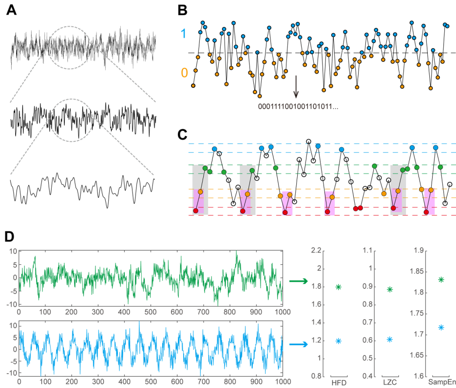
Figure 1. Illustration of the HFD, LZC and SampEn analysis. (A) The EEG time series reflect, to a certain degree, self-similarity, revealed at different timescales. The HFD is used to determine the fractal dimension of such data series. (B) In LZC analysis, a time series is binarised (by using the median value of each channel of each epoch). The values greater than the median are assigned ones (blue dots), and lower than the median are assigned zeros (orange dots). LZC can be defined as the number of unique subsequences in the binary sequence. This number can be normalized to eliminate the effects of signal length. This normalized value is the LZC used in this study. This panel was inspired by Leemburg and Bassetti (2018). (C) SampEn (here m = 2 ). Datapoints between dashed lines of the same color (red, orange, green and blue, respectively) are denoted for accepting matches (i.e., the tolerance: 20% of standard deviation). Matching points are indicated by the corresponding color. Starting from the first data point, the number of the same sequence patterns of consecutive data points are counted, also highlighted by color bars: 2-consecutive datapoints (6 pink bars): red \rightarrow orange; 3-consecutive datapoints (3 gray bars): red \rightarrow orange \rightarrow green. This procedure is repeated from the second data point, and so on. Then the total number of 2- and 3-consecutive datapoint sequence patterns are determined respectively, and the natural logarithm of their ratio is SampEn. Intuitively, the more non-repeated patterns, the larger the SampEn. This panel was inspired by Costa et al. (2005). (D) Snippets of simulated signals (1000 data points each): a more complex signal (green) and a more regular signal (blue). The latter shows a more pronounced oscillatory pattern. The HFD, LZC and SampEn values of these two signals are shown on the right (for HFD analysis of the simulated signals: we use the k_{max} value of 30). It can be noticed that the values of the blue signal are lower than the values of the green signal respectively, reflecting a lower complexity of the blue signal.
