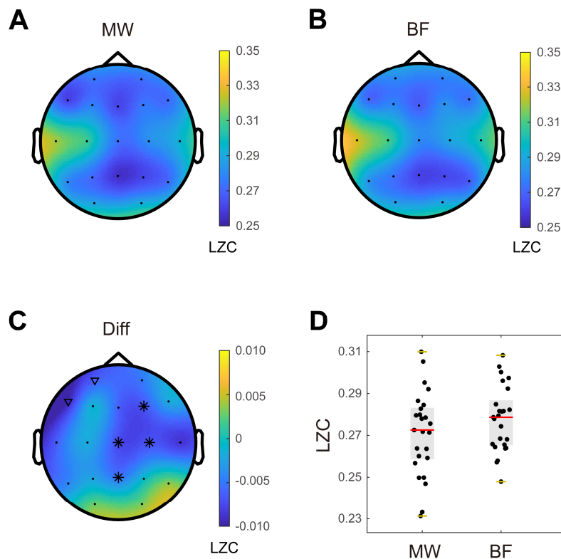
Figure 3. Differences in Lempel-Ziv complexity (LZC) between mind wandering (MW) and breath focus (BF) conditions. (A-B) Topographical plots depicting mean LZC values for MW and BF conditions in each electrode. (C) Topographical plot depicting the mean difference (Diff) between MW and BF conditions in each electrode. The black asterisks mark electrodes in which the LZC decrease (MW < BF) was significant ( p < 0.05 ). The black triangles represent the second identified cluster which shows a not significant trend ( p = 0.057 ) of LZC decrease (MW < BF) in the left frontal area. (D) Individual LZC values (averaged within the significant cluster, i.e., represented by black asterisks in Panel C) for MW and BF conditions. Each subject is represented by a dot. The gray boxes indicate the 25th and 75th percentiles. Centerlines show the median in each condition. When outliers are present, the whiskers indicate 1.5 times the interquartile range from the 25th and 75th percentiles. When no outliers are present, the whiskers lay on the most extreme data points.
