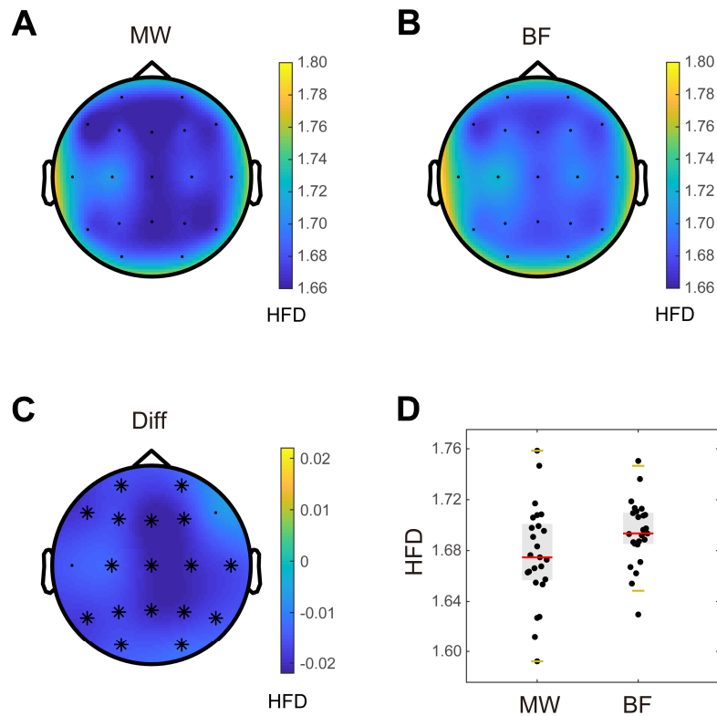
Figure 2. Differences in Higuchi's fractal dimension (HFD) between mind wandering (MW) and breath focus (BF) conditions. (A-B) Topographical plots depicting mean HFD values for MW and BF conditions in each electrode. (C) Topographical plot depicting the mean difference (Diff) between MW and BF conditions in each electrode. The black asterisks mark electrodes in which the HFD decrease (MW < BF) was significant ( p < 0.05 ). (D) Individual HFD values (averaged within the significant cluster) for MW and BF conditions. Each subject is represented by a dot. The gray boxes indicate the 25th and 75th percentiles. Centerlines show the median in each condition. When outliers are present, the whiskers indicate 1.5 times the interquartile range from the 25th and 75th percentiles. When no outliers are present, the whiskers lay on the most extreme data points.
