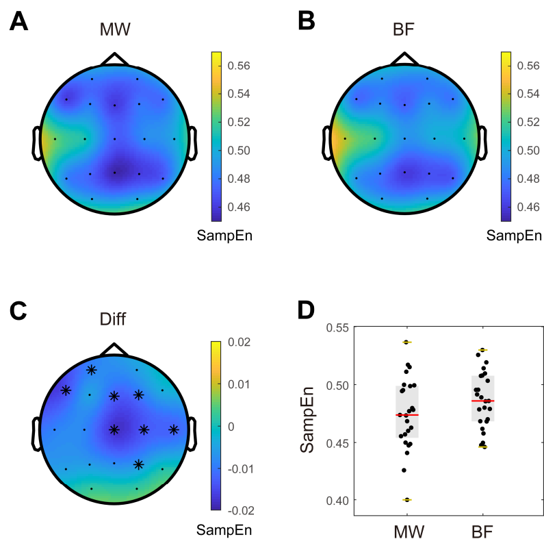
Figure 4. Differences in Sample entropy (SampEn) between mind wandering (MW) and breath focus (BF)
