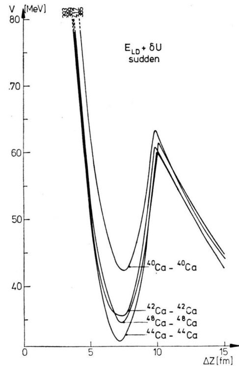
Fig. 28. The same as Fig. 24 for Ca-isotopes. The absolute heights of the Coulomb barrier and potential minimum are decreased compared with Fig. 11 (no curvature energy term). The relative depths of the potential minima are larger than in Figure 11.
