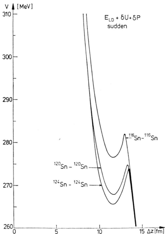
Fig. 18. The same as Fig. 6 for Sn-isotopes. The depths of the potential minima are already small compared with the potentials of the lighter nuclei (Fig. 6—Figure 17).
