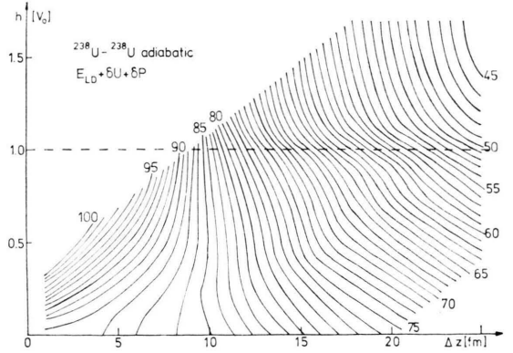
Fig. 35. The same as Fig. 31 for ^{238}\text{U}-^{238}\text{U} scattering. No minimum can be observed in this PES. The contour lines have 10 MeV equidistance and their value has to be multiplied by a factor 10.
