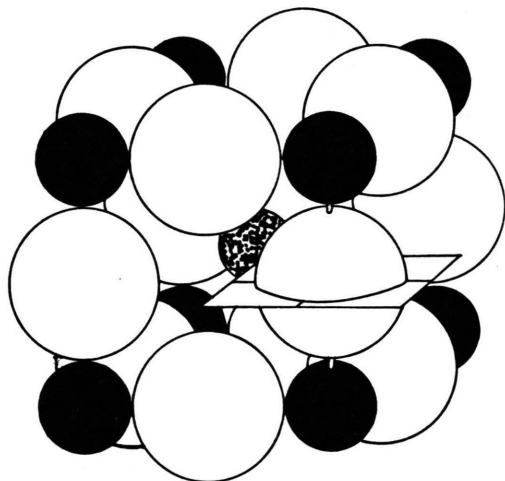
Fig. 1. Crystal structure of \text{KZnF}_3 , speckled sphere: \text{K}^+ ion, black spheres: \text{Zn}^{2+} ions, white spheres: \text{F}^- ions. The radii of the spheres do not correspond to the true radii of the ions. For one \text{F}^- the mirror plane and the fourfold symmetry axis are indicated.
