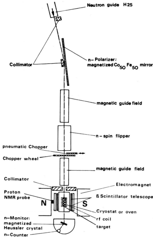
Fig. 2. Experimental set-up.
