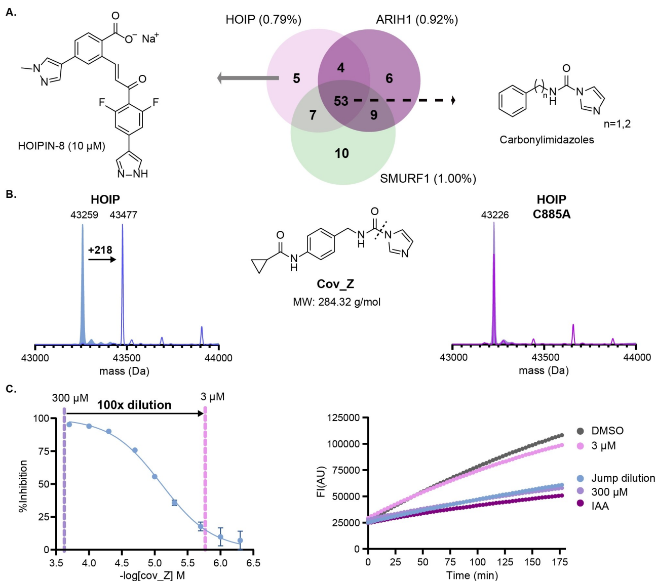
Figure 5. UbsRhodol in a fragment-based ligand HTS screening campaign. A) Venn diagram displaying the number of validated hits (> 60% inhibition) obtained in the three screening campaigns with UbsRhodol. Percentage indicated represents the hit rate for each E3 ligase. For a deeper characterization of compounds see Supporting Information Extended Table 1. B) MS-adduct formation experiments with carbonyl imidazole Cov_Z showed specific targeting of cysteine 885 of HOIP as confirmed by mutagenesis experiments and C) Jump dilution assays (100x dilution) against HOIP showed an irreversible covalent mode of action (showed for Cov_Z, see Supporting Information Figure 22–23 for X and Y) (stand. dev., n=3 ).
