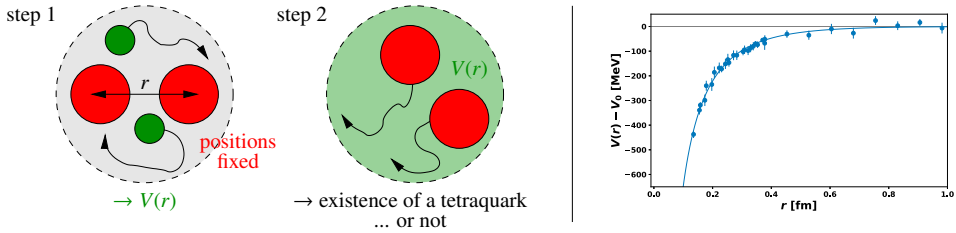
Figure 1. (left) Study of a \bar{b}\bar{b}qq tetraquark in the Born-Oppenheimer approximation (red circles represent the two heavy antiquarks \bar{b}\bar{b} , green circles the two light quarks qq ). Step 1: Lattice QCD computation of an antistatic-antistatic potential V(r) . Step 2: Solving the Schrödinger equation with the potential V(r) for the relative coordinate of the \bar{b} quarks provides information about the possible existence of a tetraquark. (right) The most attractive antistatic-antistatic potential [12].
