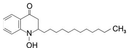
1-hydroxy-2-dodecyl-4(1H)quinolone
