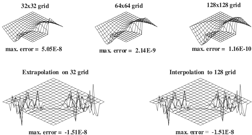
Fig. 2: potential errors for half of a spherical condenser by 9-point discretization. upper row : potential errors on 32×32, 64×64, and 128×128 grid. Lower row – left: potential errors by extrapolating the solutions on 32×32 grid – right: interpolation of extrapolated potentials on 128×128 grid
