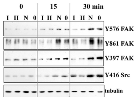
FIGURE 9. Enhanced phosphorylation of FAK and Src in osteoarthritic chondrocytes after apoptosis induction by camptothecin. Immunoblots of cell lysates of OA chondrocytes that were silenced using ADAM15-specific siRNAs I and II and a nonfunctional siRNA (N) or transfection agent alone (0) and treated with camptothecin, showing marked induction of phosphorylation of FAK at Tyr-576, Tyr-861, and Tyr-397 and Src at Tyr-416 by camptothecin after 15 and 30 min (N and 0), which is strongly reduced after silencing of ADAM15 (I and II). Shown are representative results of an analysis performed on primary chondrocytes derived from five OA cartilage samples.
