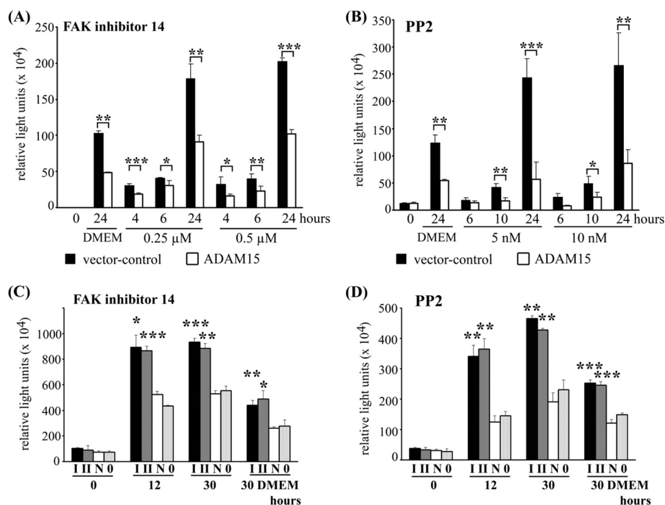
FIGURE 8. Inhibition of FAK and Src signaling by FAK 14 inhibitor and PP2 in the presence of ADAM15. Vector- (black bars) and ADAM15-transfected cells (open bars) were treated with 0.25 \mu M and 0.5 \mu M FAK 14 inhibitor (A) and 5 nM and 10 nM PP2 (B) for the time points shown, and caspase-3/7 activity was determined. A significantly increased caspase activity was detected in the control cells in contrast to ADAM15-transfected cells that exhibited higher apoptosis resistance to both inhibitors. Incubation with DMEM alone also displayed a significantly higher caspase activity in vector control cells. C and D, ADAM15 transfected cells were silenced using siRNA I and II for 40 h and treatment with 0.25 \mu M FAK 14 inhibitor (C) or 5 nM PP2 (D) resulted in a significantly higher caspase activity as compared with cells silenced with a nonfunctional siRNA (N) or with transfection agent alone (0). Incubation with DMEM alone served as control. Shown are representative results of least five repeated experiments. *, p < 0.05 ; **, p < 0.005 ; ***, p < 0.0005 .
