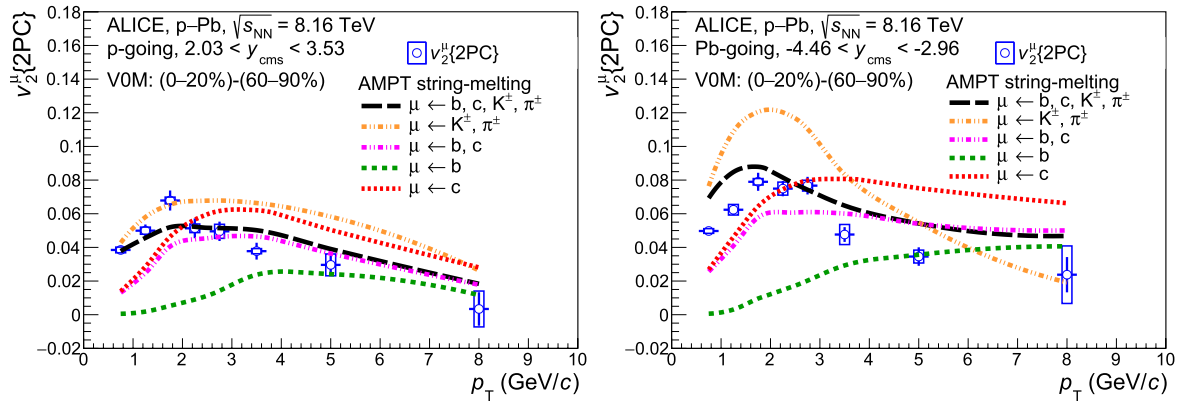
Fig. 6. Comparison of the p_T -differential v_2^\mu {2PC} of inclusive muons at forward (left) and backward (right) rapidities in high-multiplicity p-Pb collisions at \sqrt{s_{NN}} = 8.16 TeV with AMPT calculations [81–83]. The predictions are shown for muons from charm-hadron decays and beauty-hadron decays, separately, muons from charged-pion and kaon decays, and for muons from the combination of the various sources. The contribution of muons from both charm- and beauty-hadron decays is also displayed.
