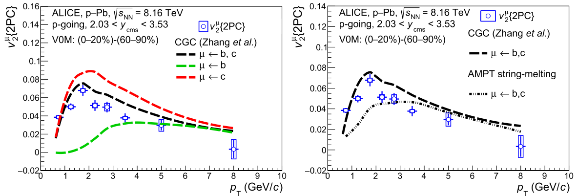
Fig. 7. Left: comparison of the p_T -differential v_2^\mu {2PC} of inclusive muons at forward rapidity in high-multiplicity p-Pb collisions at \sqrt{s_{NN}} = 8.16 TeV with CGC-based calculations [113,114]. The predictions are shown for muons from charm-hadron decays and beauty-hadron decays, separately, and for muons from the combination of the two sources. Right: comparison of the p_T -differential v_2 of muons from heavy-flavour hadron decays as obtained with CGC and AMPT calculations with the measured inclusive muon v_2 .
