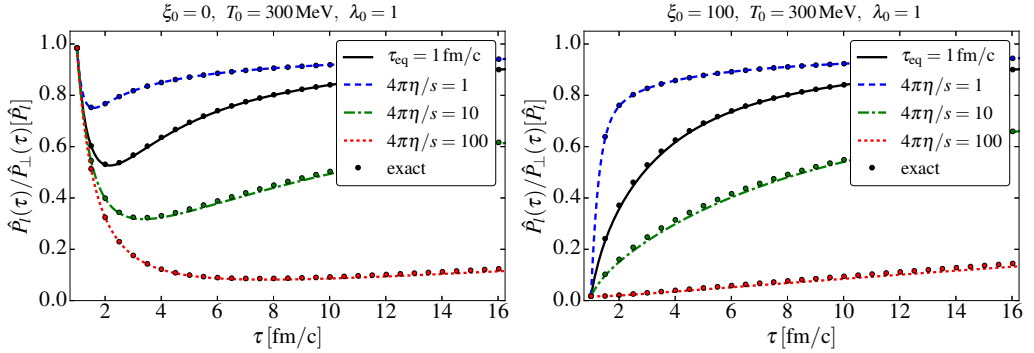
Fig. 2. (Color online) The evolution of \hat{P}_\parallel/\hat{P}_\perp as a function of proper time \tau . The lines are the solution of the conservation equations closed by the relaxation equation for \hat{P}_\parallel with \tau_{eq} = 1 fm and with three different choices for \eta/s . The corresponding solutions of the Boltzmann equation are shown by the large dots. The figure is taken from Ref. [12].
