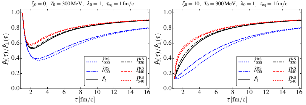
Fig. 1. The evolution of \hat{P}_l/\hat{P}_\perp as a function of proper time \tau for the different choices of \hat{I}_{nrq}^{RS} for closure. The figure is taken from Ref. [12].
