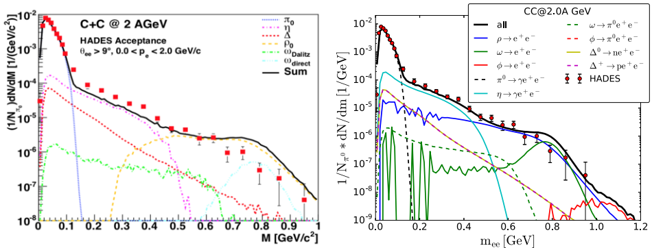
Fig. 3. Dilepton production as a function of the invariant mass in carbon-carbon collisions at E_{lab} = 2A GeV within the UrQMD transport approach (left, Fig. taken from [16]) and SMASH (right, Fig. taken from [14]).
