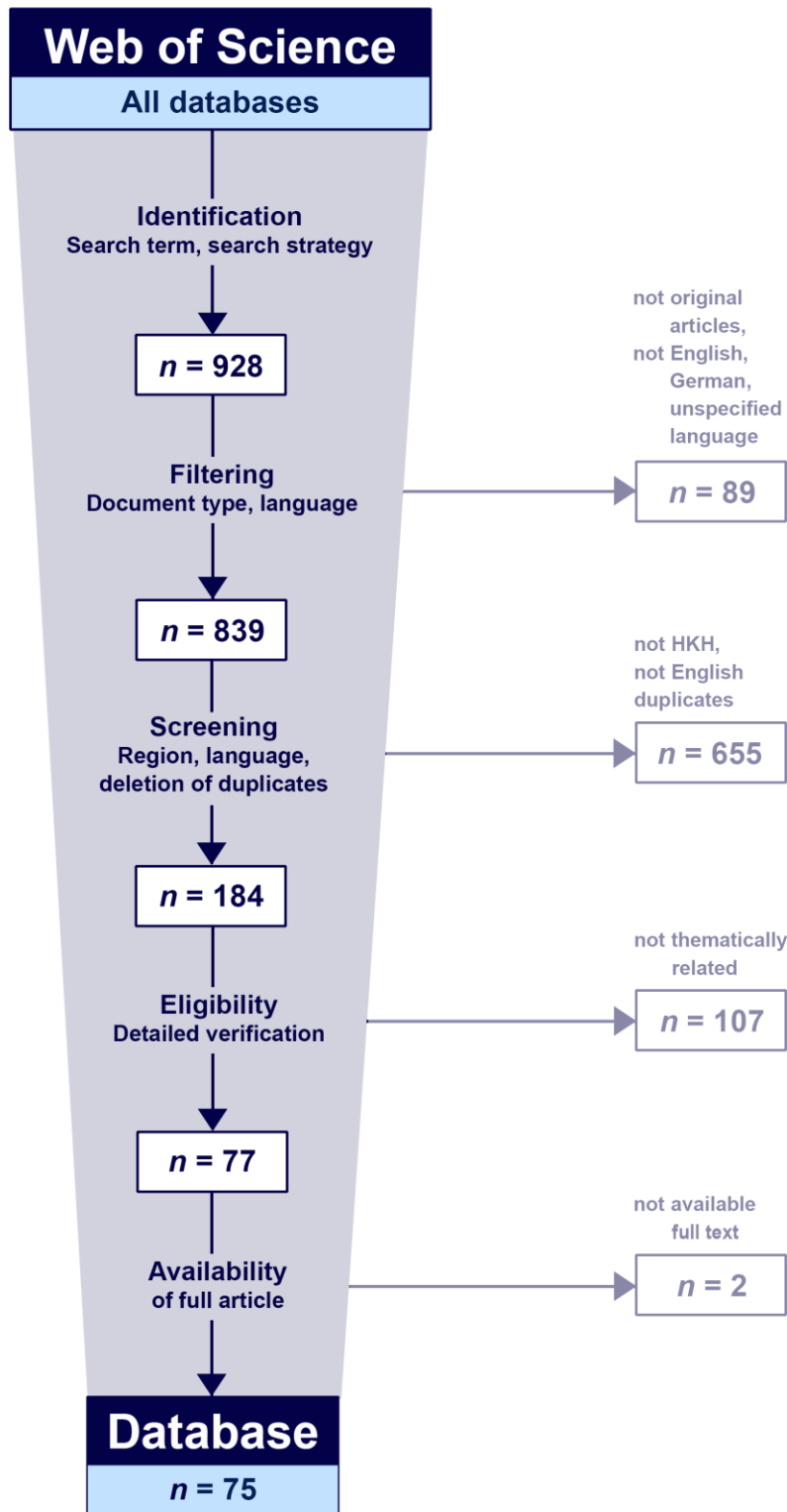
Fig. A1. Establishment of database following Preferred Reporting Items for Systematic Reviews and Meta-Analyses (PRISMA) guideline.
