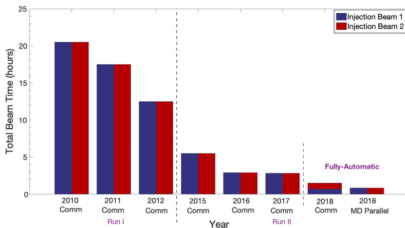
Fig. 5. The time to align the collimators at injection commissioning, compared to the 2018 parallel alignment MD, from [53].
