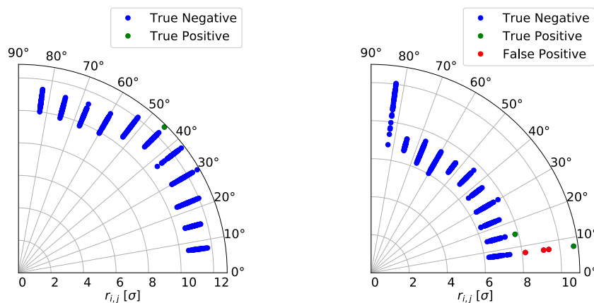
Fig. 16. DA simulations for two LHC configurations. The initial 4D co-ordinates are of the type (x, 0, y, 0) and a polar scan is performed on (x, y) . The various markers represent the results of the sixty seeds used. Left: Example of a DA computation where an outlier is correctly flagged (in green). Right: Examples of false positives (in red). The FP cases, are less worrisome as they refer to the determination of the maximum stable amplitude, which does not affect DA_{min} . (For interpretation of the references to colour in this figure legend, the reader is referred to the web version of this article.)
