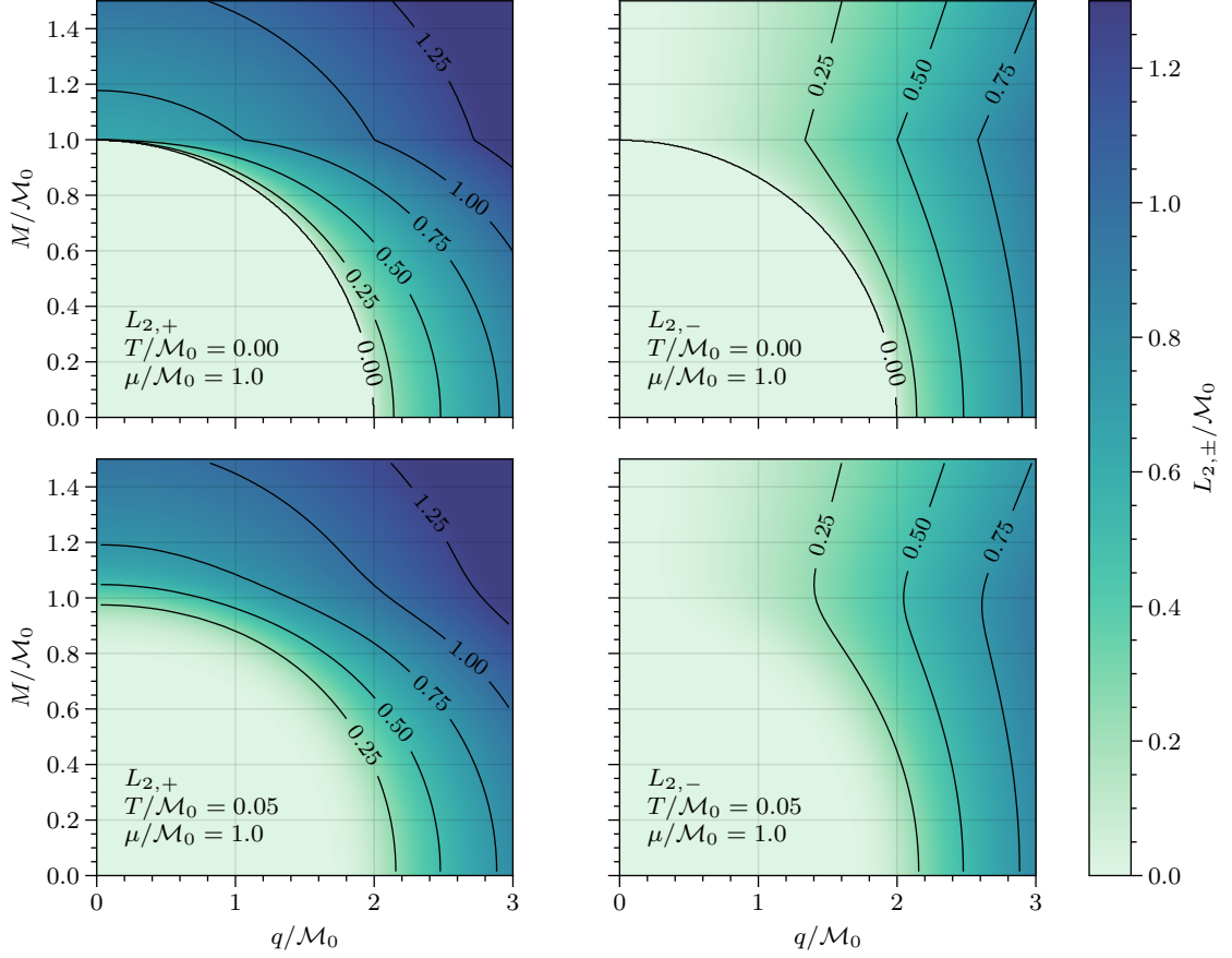
FIG. 1. L_{2,+} and L_{2,-} for T/\mathcal{M}_0 = 0, 0.05 and \mu/\mathcal{M}_0 = 1.0 as a function of q and M . Also at finite temperature L_{2,-}(M^2, \mu, T, q^2 = 0) = 0 . However, the 0.0 contour line and its label are not drawn, because they would be obscured by the axis. In the ancillary files to this paper, we provide a script, which allows to do the numerical computation of L_{2,\pm} for arbitrary values of (M^2, \mu, T, q^2) and that produces this figure. See Eqs. (13) and (15) for the definition of L_{2,\pm} .
