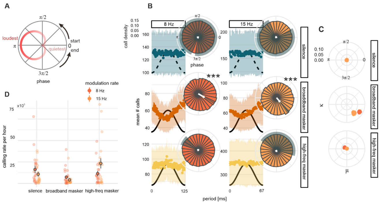
Fig. 2. Anti-phase preference for call onset timing in broadband noise. (A) Schematic representing the translation from the cartesian to polar coordinates. 0 phase (right) corresponds to the amplitude trough. Red trace represents amplitude change over a cycle. (B) Average call onset distributions within the modulation cycle track the inverse of the amplitude phase in broadband masker conditions, but not in silent and high-freq masker conditions (1 ms bins). Shaded areas indicate standard error of the mean (SEM). Black curves: schematic of amplitude envelope (not to scale) in playback conditions and simulated amplitude envelope in silent conditions. Insets: Circular density histograms of call onsets (30 bins). White arrows indicate resultant angular means; arrow lengths indicate resultant lengths (concentration of data at the angular mean). Shaded areas indicate maximum likelihood (MLE) 95% confidence intervals for angular means. Stars indicate significant p-values from Rayleigh's test of uniformity. *** p < 0.001 (C) Bootstrapped MLE von Mises mean ( \mu ) and concentration ( \kappa ) parameters indicating robust pattern of call onset clustering in the broadband masking condition for both modulation rates. (D) Data points (lightly colored dots) indicate number of calls observed per hour for each group for each recording day. Estimated mean calling rates (darkly colored dots with gray outline) from negative binomial models show a drop in calling between silent baseline and acoustic masking conditions (except for 15 Hz high-freq masker condition). Gray vertical lines indicate SE of model fit for predicted means.
