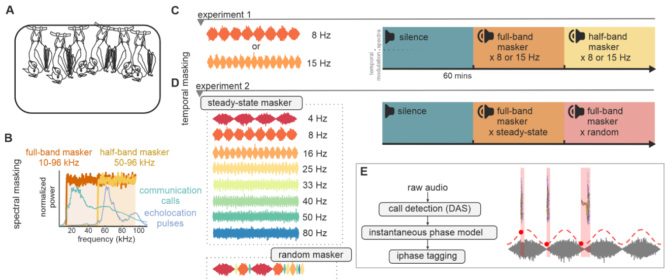
75 Fig. 1. Schematic of experiments. (A) Each group of bats consisted of 6 adults (4 male) that could flit and socialize freely in a cage placed within the recording chamber. (B) Stimuli were broadband white noise with 10-96 kHz (broadband masker) and 50-96 kHz (high-freq masker) carrier frequencies. Teal and violet traces indicate normalized power spectra of C. perspicillata communication and 80 echolocation calls, counterbalanced. (C) In experiment 1 , maskers were amplitude modulated at 8 or 15 Hz for each group. Procedure (right): Recording days (5) consisting of three one-hour blocks: a silent baseline, then playback of the broadband and high-freq 85 masking noise, counterbalanced. (D) In experiment 2 , broadband masking noise was amplitude modulated at eight amplitude modulation (AM) rates (4-80Hz). A random condition consisted of a randomly permuted sequence of the eight AM cycles. Procedure (right): Recording days (5) consisted of a silent baseline, then playback of the steady-state maskers (playback of each modulation rate for 7.5 minutes each in randomized order), and random masking noise, counterbalanced. (E) Data analysis: Call events (pink shaded areas) were detected using Deep Audio Segmenter (DAS). Calls were tagged with the instantaneous phase (red dots) of the amplitude envelope (red dashed line) at call onset time.
