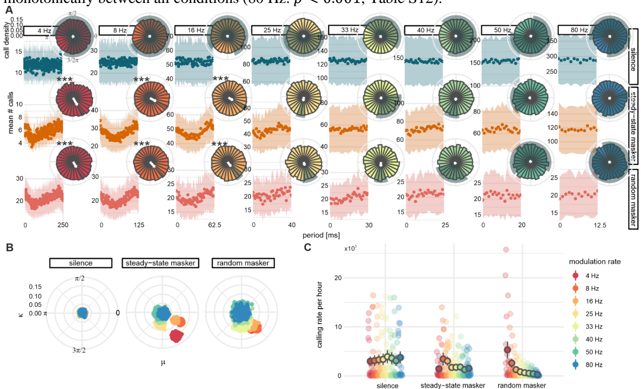
200 Fig. 3. Call timing adaptation to amplitude modulated noise is independent of predictability but sensitive to rate. (A) Average call onset distributions show call timings follow the inverse of the amplitude modulation cycle in both predictable (steady-state) and unpredictable (random) temporal contexts, but only do so reliably up to 16 Hz. *** p < 0.001 , Rayleigh’s test. (B) MLE von Mises mean and concentration parameters indicate that the call clustering pattern is robust but graded in playback conditions, with the
