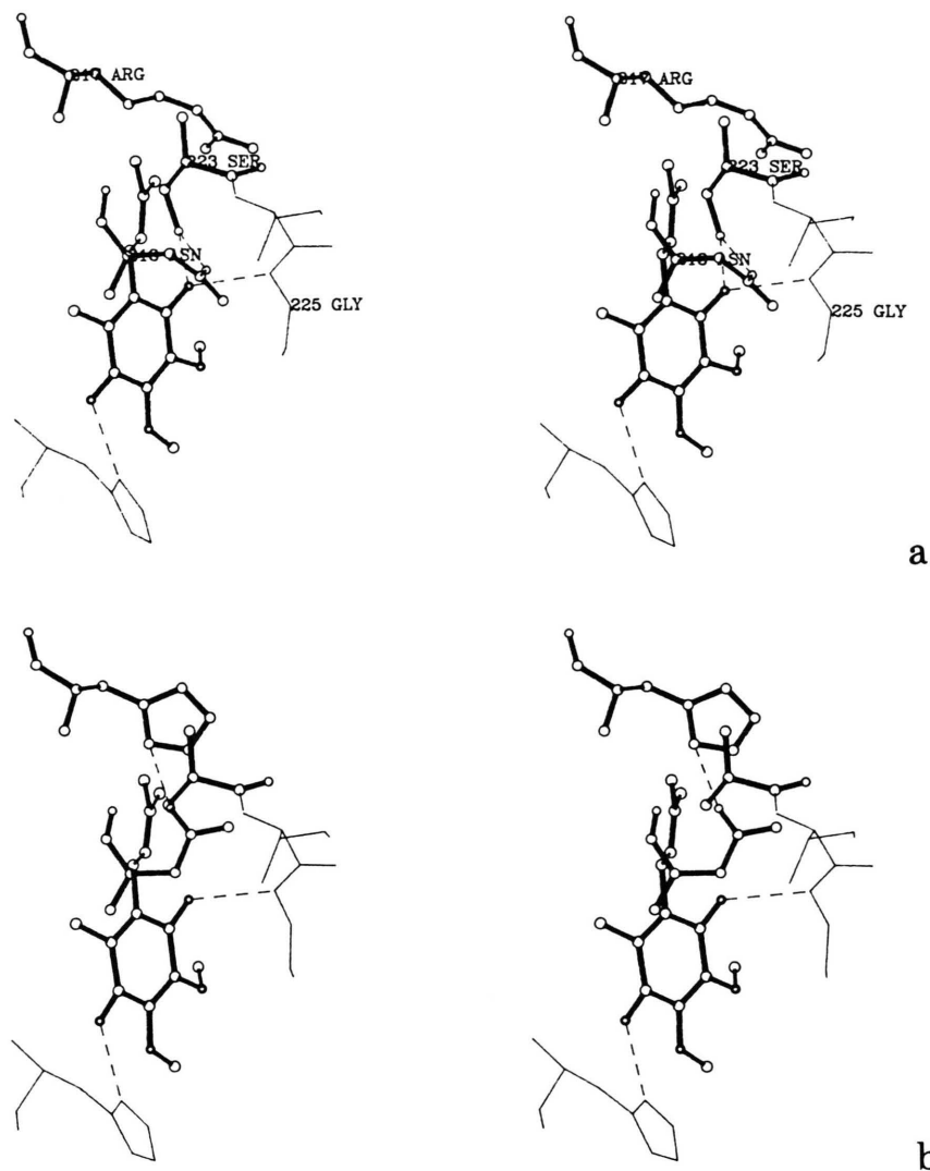
Fig. 1. Stereo plots of part of the Q_B site of a) Rps. viridis wild type; b) mutant T1 (SerL223 \rightarrow Ala, ArgL217 \rightarrow His). Possible hydrogen bonds are drawn as dashed lines. The quinone oxygen which is hydrogen bonded to serine L223 in the wild type will be referred to as oxygen-1 and that, which is hydrogen bonded to histidine L190 as oxygen-2. Ubiquinone, arginine L217, serine L223 and asparagine L213 are shown as atomic models. Histidine L190, isoleucine L224 and glycine L225 are drawn in a skeletal mode. Fig. 1 and 2 were produced by a computer program written by Lesk and Hardman [28].
