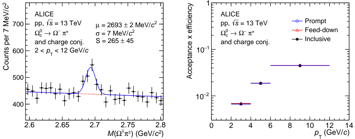
Figure 1: (Left panel): invariant-mass distribution of \Omega_c^0 \rightarrow \Omega^- \pi^+ candidates and their charge conjugates integrated over the whole p_T interval 2–12 GeV/c. The blue line shows the total fit function and the red line represents the combinatorial background fit. (Right panel): acceptance-times-efficiency for prompt, feed-down, and inclusive \Omega_c^0 baryons decaying into \Omega^- \pi^+ as a function of p_T in pp collisions at \sqrt{s} = 13 TeV.
