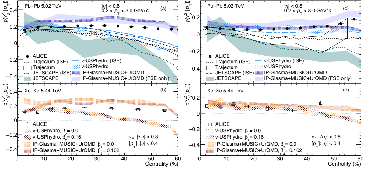
Figure 1: Centrality dependence of \rho(v_2^2, [p_T]) (left) and \rho(v_3^2, [p_T]) (right) in Pb–Pb at \sqrt{s_{NN}} = 5.02 TeV (a, c) and Xe–Xe collisions \sqrt{s_{NN}} = 5.44 TeV (b, d). The statistical (systematic) uncertainties are shown as vertical bars (filled boxes). The initial-state estimations (ISE) are represented by lines, while IP-Glasma+MUSIC+UrQMD [26], v-USPhydro [40], Trajectory [30], and JETSCAPE [31] hydrodynamic model calculations are shown with hatched bands.
