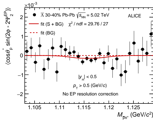
Figure 1: (color online) Fit to the invariant mass dependence of the \langle \cos \theta_p^* \sin(2\phi - 2\Psi_2^{\text{EP}}) \rangle for \bar{\Lambda} before event-plane resolution correction using Eq. 8 in the 30–40% centrality class. See text for details.
