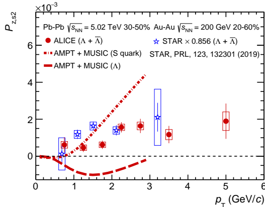
Figure 3: (color online) Transverse momentum dependence of P_{z,s2} averaged for \Lambda and \bar{\Lambda} in Pb–Pb collisions at \sqrt{s_{\text{NN}}} = 5.02 TeV in semi-central collisions and its comparison with the similar RHIC results for Au–Au collisions at \sqrt{s_{\text{NN}}} = 200 GeV. The model calculations [38] for \Lambda and strange quark for Pb–Pb collisions at \sqrt{s_{\text{NN}}} = 5.02 TeV in the 30–50% centrality interval using the approach described in Ref. [23] are shown by dash-dotted lines.
