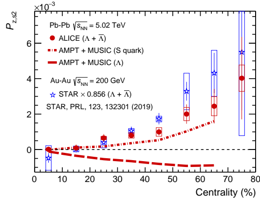
Figure 2: (color online) Centrality dependence of P_{z,s2} averaged for \Lambda and \bar{\Lambda} in Pb–Pb collisions at \sqrt{s_{\text{NN}}} = 5.02 TeV and its comparison with the RHIC results for Au–Au collisions at \sqrt{s_{\text{NN}}} = 200 GeV. The model calculations [38] for \Lambda and strange quark for Pb–Pb collisions at \sqrt{s_{\text{NN}}} = 5.02 TeV using the approach described in Ref. [23] are shown by dash-dotted lines.
