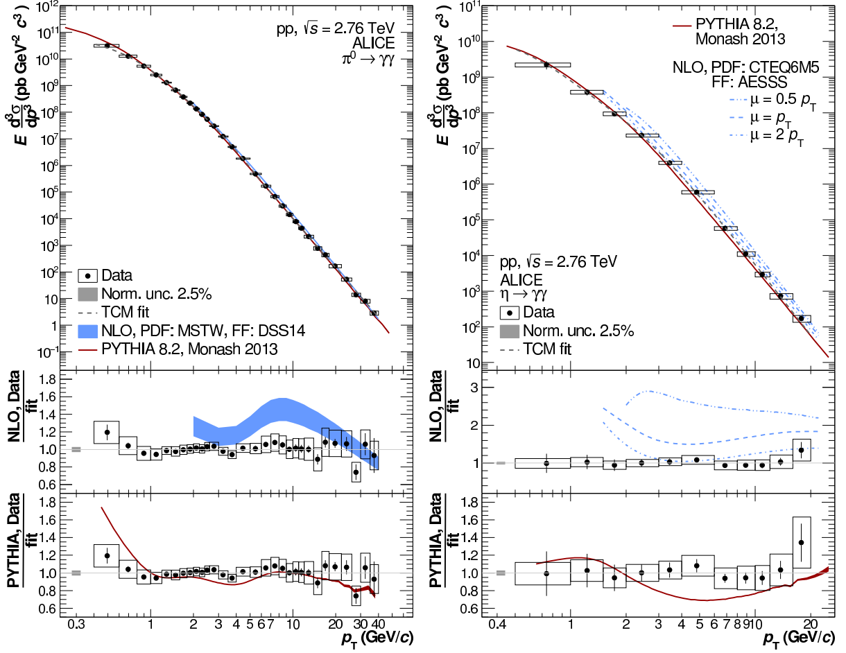
Fig. 9: Invariant differential cross section of the \pi^0 (left, top panel) and \eta meson (right, top panel) for pp collisions at \sqrt{s} = 2.76 TeV. The data are compared to PYTHIA 8.2 [30] generator-level simulations using the Monash 2013 tune as well as recent NLO pQCD calculations [3, 6]. The ratios of the data and the calculations to the respective two-component model fits [25, 26] to the data are shown in the lower panels. The horizontal error bars denote statistical, the boxes systematic uncertainties.
