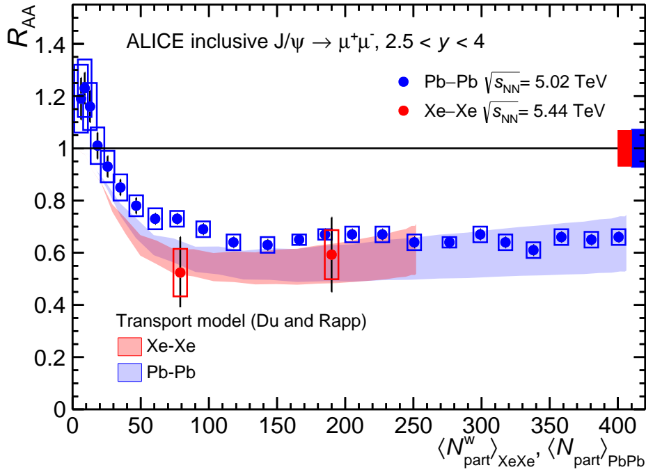
Fig. 2: The inclusive J/\psi nuclear modification factor for Xe–Xe collisions at \sqrt{s_{\text{NN}}} = 5.44 TeV. The results are plotted using as centrality variable \langle N_{\text{part}}^w \rangle , obtained by weighting, in each centrality interval, the N_{\text{part}} distribution with the corresponding distribution of the number of nucleon-nucleon collisions. The error bars represent the statistical uncertainties, the boxes around the points the uncorrelated systematic uncertainties. Correlated uncertainties are shown as a filled box around unity. The results are compared with the same quantity for Pb–Pb collisions at \sqrt{s_{\text{NN}}} = 5.02 TeV [10] and to the results of the calculation of a transport model [13, 14]. For Pb–Pb, the weighting of N_{\text{part}} with the number of nucleon-nucleon collisions was not performed, since it leads to a negligible effect when the centrality intervals are narrow.
