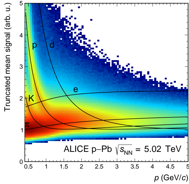
Fig. 38: Truncated mean signal as a function of momentum for p–Pb collisions at \sqrt{s_{\text{NN}}} = 5.02 TeV. The solid lines represent the expected signals for various particle species.
