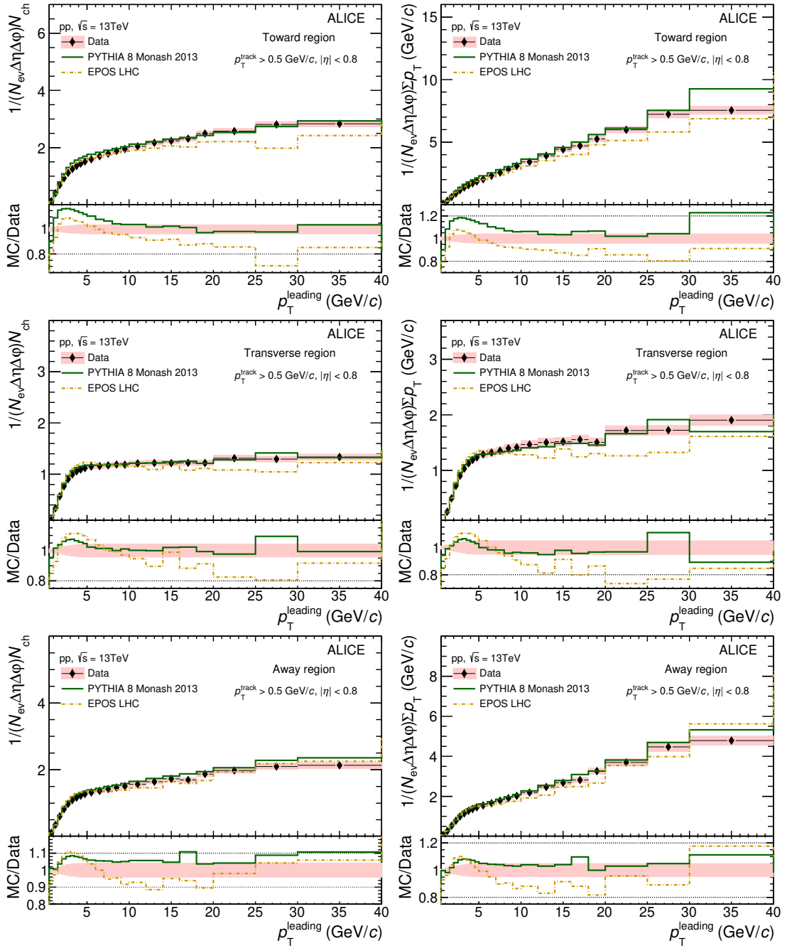
Figure A.1: Number density N_{\text{ch}} (left) and \sum p_{\text{T}} (right) distributions as a function of p_{\text{T}}^{\text{leading}} compared to MC predictions in Toward (top), Transverse (middle), and Away (bottom) regions for p_{\text{T}}^{\text{track}} > 0.5 GeV/c. The shaded areas in the upper panels represent the systematic uncertainties and vertical error bars indicate statistical uncertainties. In the lower panels, the shaded areas are the sum in quadrature of statistical and systematic uncertainties from the upper panels. No uncertainties are given for the MC calculations.
