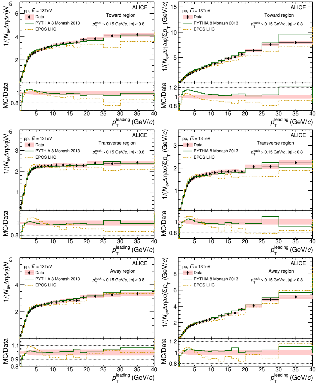
Figure 4: Number density N_{ch} (left) and \Sigma p_T (right) distributions as a function of p_T^{leading} along with the MC predictions in Toward (top), Transverse (middle), and Away (bottom) regions for the threshold of p_T^{track} > 0.15 GeV/c. The shaded areas in the upper panels represent the systematic uncertainties and vertical error bars indicate statistical uncertainties. In the lower panels, the shaded areas are the sum in quadrature of statistical and systematic uncertainties from upper panels. No uncertainties are shown for the MC calculations.
