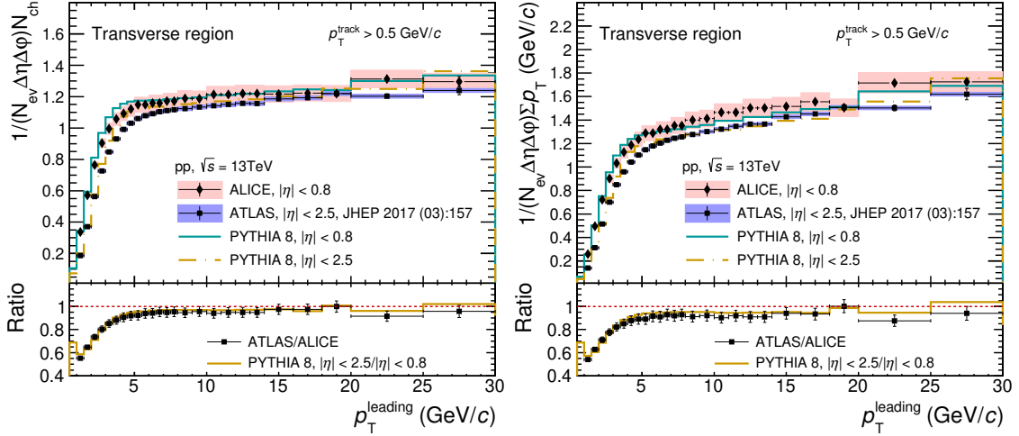
Figure 8: Number density N_{\text{ch}} (left) and \sum p_T density (right) in the Transverse region for p_T^{\text{track}} > 0.5 GeV/c at \sqrt{s} = 13 TeV from ALICE ( |\eta| < 0.8 ) and ATLAS ( |\eta| < 2.5 ) measurements [14]. The results are compared to PYTHIA 8 Monash-2013 calculations. The shaded areas represent the systematic uncertainties and vertical error bars indicate statistical uncertainties. No uncertainties are shown for the MC calculations.
