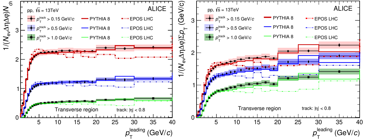
Figure 5: Number density N_{ch} (left) and \Sigma p_T (right) distributions as a function of p_T^{\text{leading}} along with the MC predictions in Transverse region for three transverse momentum thresholds of p_T^{\text{track}} > 0.15, 0.5, and 1.0 GeV/c. The shaded areas represent the systematic uncertainties and vertical error bars indicate statistical uncertainties.
