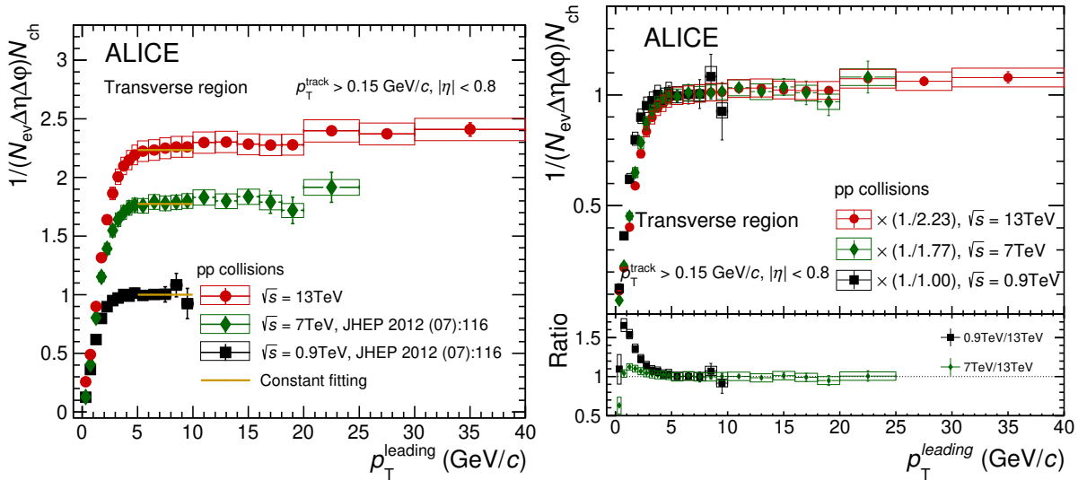
Figure 6: Left: Number density N_{ch} in the Transverse region as a function of p_T^{\text{leading}} ( p_T^{\text{track}} > 0.15 GeV/c threshold) for \sqrt{s} = 0.9, 7 and 13 TeV. A constant function is used to fit the data in the range 5 < p_T^{\text{leading}} < 10 GeV/c and the results are shown as solid lines. Right: Number densities N_{ch} scaled by the pedestal values obtained from the fit in order to compare the shapes. The open boxes represent the systematic uncertainties and vertical error bars indicate statistical uncertainties.
