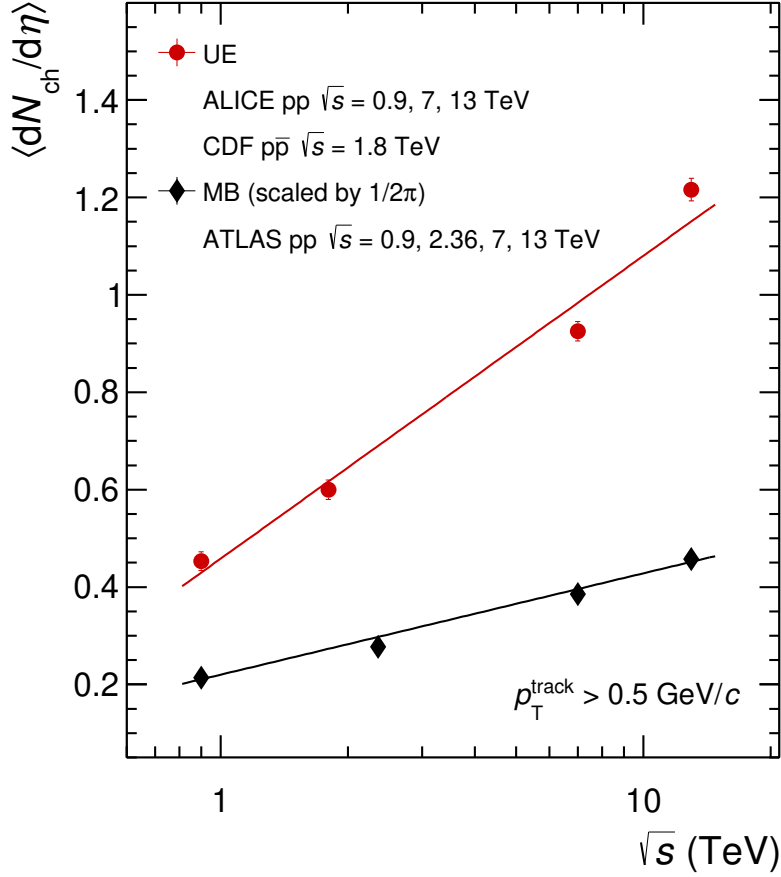
Figure 7: Comparison of number density in the plateau of the Transverse region with lower energy data taken from [5, 12] and dN_{\text{ch}}/d\eta in minimum-bias events (scaled by 1/2\pi ) [48]. Both are for charged-particles with p_{\text{T}} > 0.5 GeV/c. Error bars represent statistical and systematic uncertainties summed in quadrature. The straight lines show the results of fitting data points with the functional form a + b \ln s .
