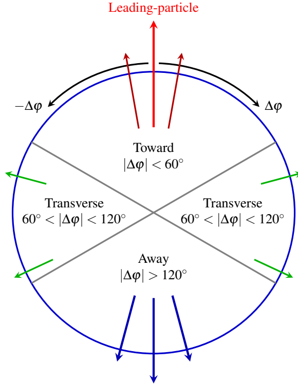
Figure 1: Illustration of the Toward, Transverse, and Away regions in the azimuthal plane with respect to the leading track direction.
