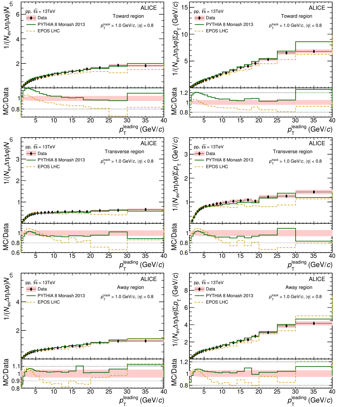
Figure A.2: Number density N_{ch} (left) and \sum p_T (right) distributions as a function of p_T^{\text{leading}} and the comparisons to MC predictions in Toward (top), Transverse (middle), and Away (bottom) regions for p_T^{\text{track}} > 1.0 GeV/c. The shaded areas in the upper panels represent the systematic uncertainties and vertical error bars indicate statistical uncertainties. In the lower panels, the shaded areas are the sum in quadrature of statistical and systematic uncertainties from the upper panels. No uncertainties are given for the MC calculations.
