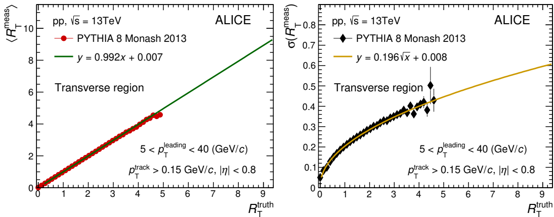
Figure 2: Mean R_T^{\text{meas}} and standard deviation \sigma of the R_T^{\text{meas}} distribution as a function of R_T^{\text{truth}} . The solid lines represent the fits to the points and the extrapolation to higher R_T^{\text{truth}} , resulting in the parameterized response matrix used for unfolding.
