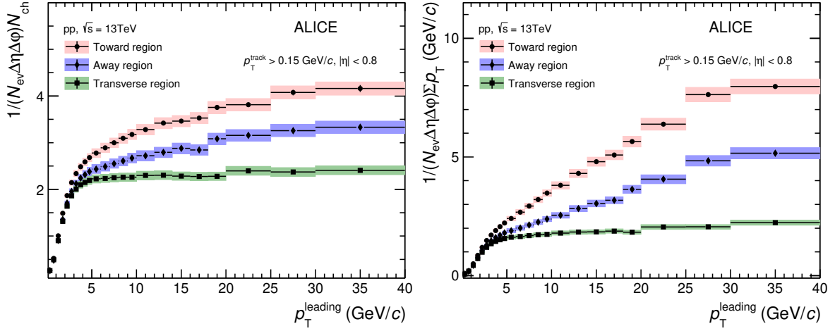
Figure 3: Number density N_{\text{ch}} (left) and \sum p_T (right) distributions as a function of p_T^{\text{leading}} in Toward, Transverse, and Away regions for p_T^{\text{track}} > 0.15 GeV/c. The shaded areas represent the systematic uncertainties and vertical error bars indicate statistical uncertainties.
