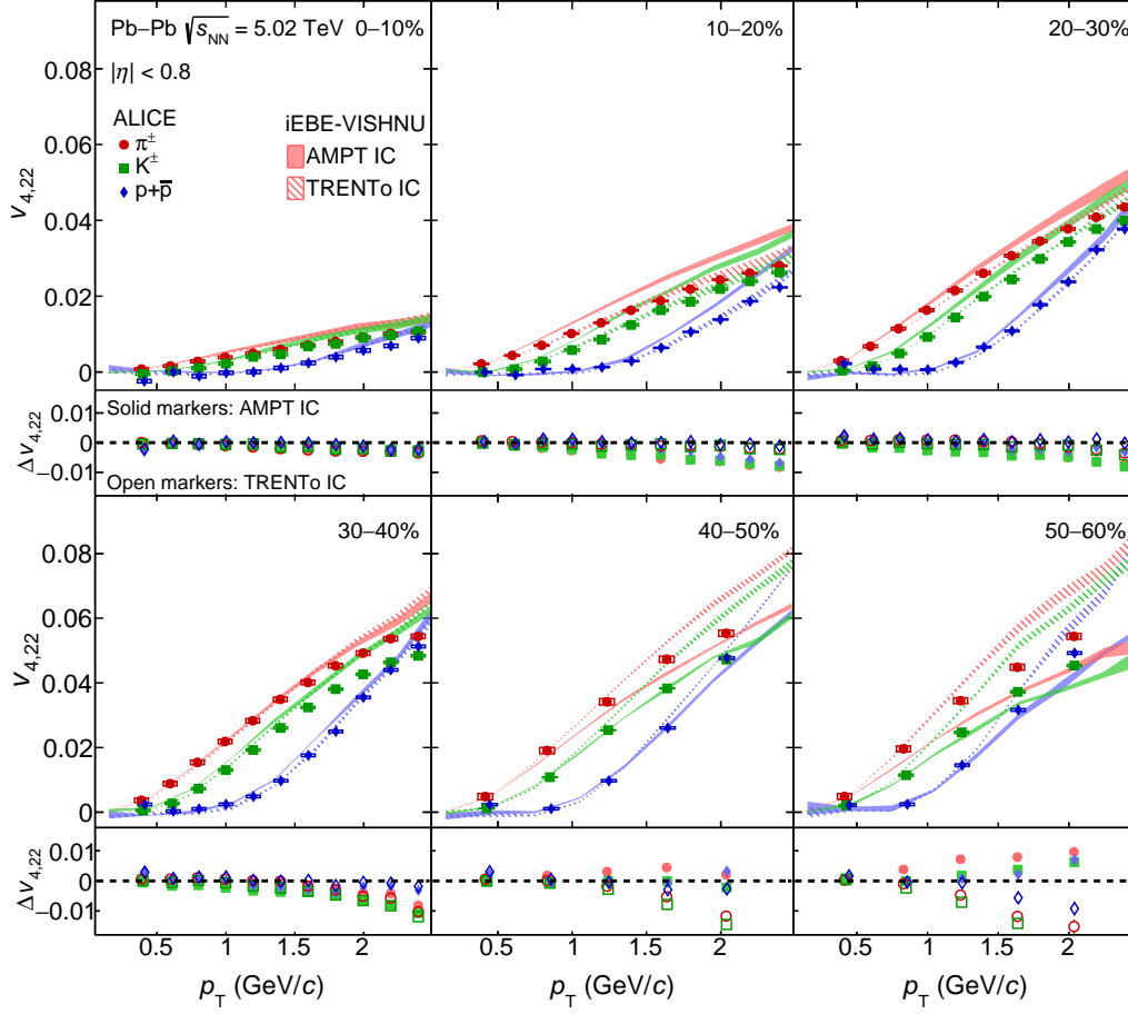
Figure 15: The p_T -differential v_{4,22} of \pi^\pm , K^\pm and p + \bar{p} in the 0–10% up to 50–60% centrality intervals of Pb–Pb collisions at \sqrt{s_{\text{NN}}} = 5.02 TeV compared with iEBE-VISHNU hybrid models with two different sets of initial parameters: AMPT initial conditions ( \eta/s = 0.08 and \zeta/s = 0 ) shown as solid bands and TRENTo initial conditions ( \eta/s(T) and \zeta/s(T) ) as hatched bands. The bottom panels show the difference between the measurements and each model. Statistical and systematic uncertainties are shown as bars and boxes, respectively.
