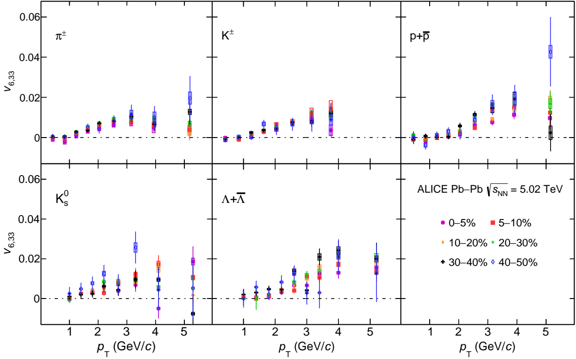
Figure 4: The p_T -differential v_{6,33} for different centrality intervals of Pb–Pb collisions at \sqrt{s_{\text{NN}}} = 5.02 TeV grouped by particle species. Statistical and systematic uncertainties are shown as bars and boxes, respectively.
