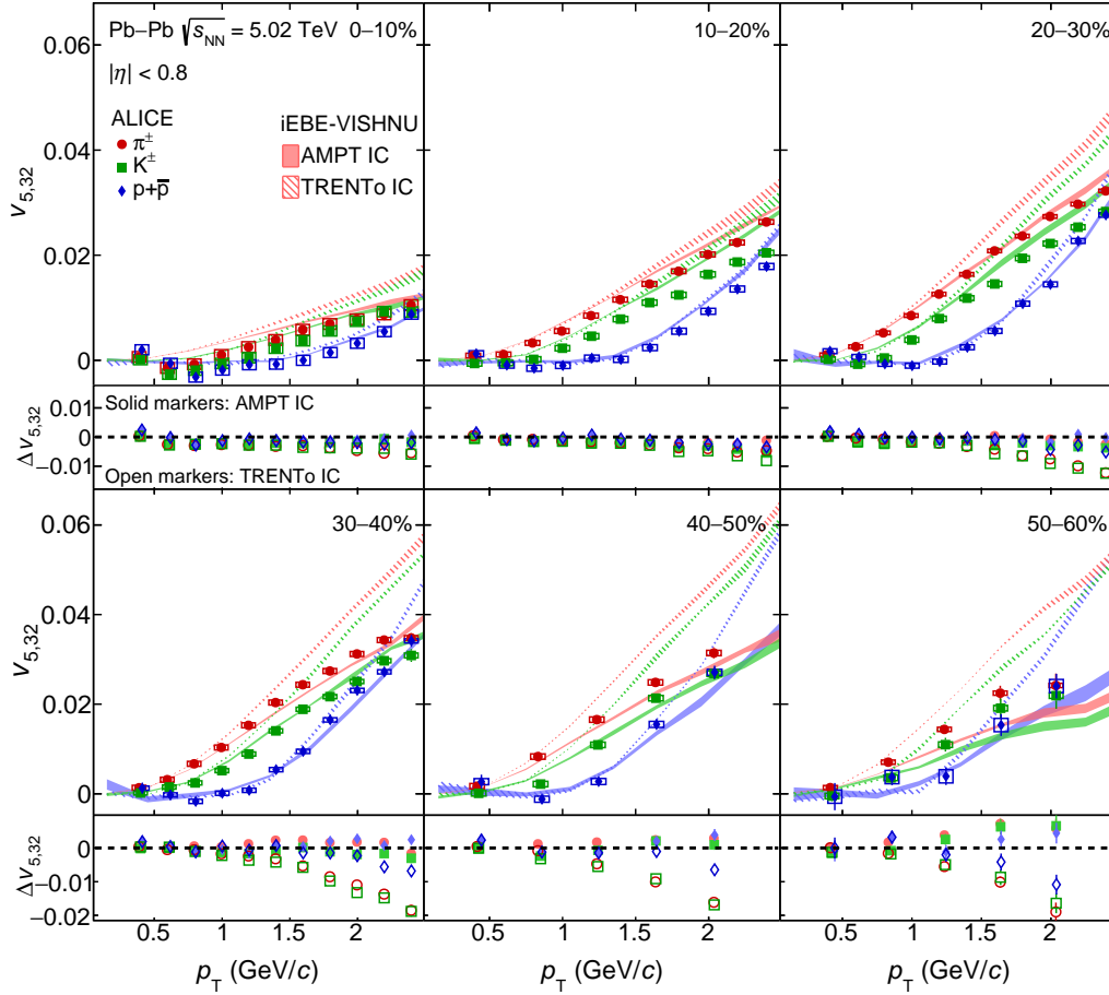
Figure 16: The p_T -differential v_{5,32} of \pi^\pm , K^\pm and p + \bar{p} in the 0–10% up to 50–60% centrality intervals of Pb–Pb collisions at \sqrt{s_{\text{NN}}} = 5.02 TeV compared with iEBE-VISHNU hybrid models with two different sets of initial parameters: AMPT initial conditions ( \eta/s = 0.08 and \zeta/s = 0 ) shown as solid bands and TRENTo initial conditions ( \eta/s(T) and \zeta/s(T) ) as hatched bands. The bottom panels show the difference between the measurements and each model. Statistical and systematic uncertainties are shown as bars and boxes, respectively.
