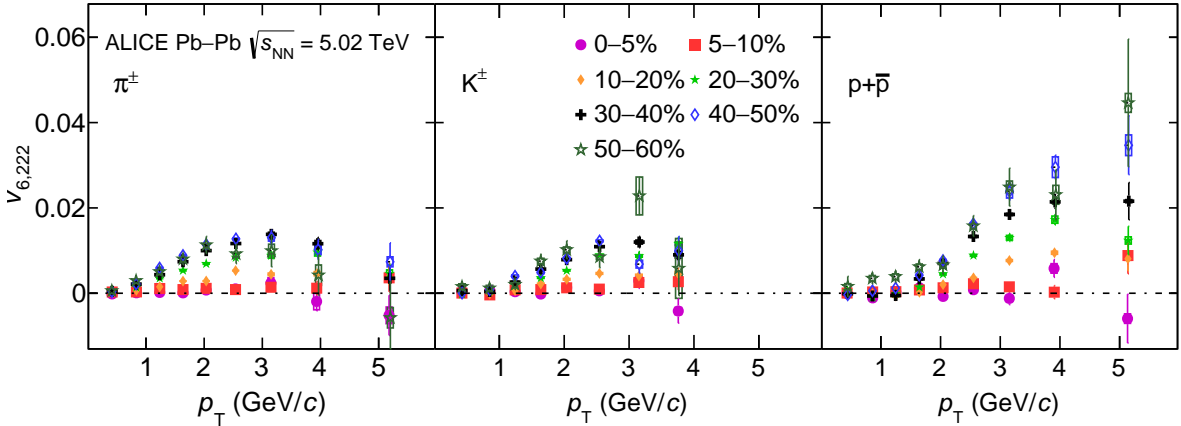
Figure 5: The p_T -differential v_{6,222} for different centrality intervals of Pb–Pb collisions at \sqrt{s_{\text{NN}}} = 5.02 TeV grouped by particle species. Statistical and systematic uncertainties are shown as bars and boxes, respectively.
