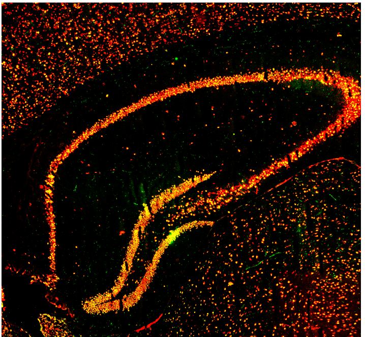
Figure S2: High resolution images of LPPR5 Immuno-histochemical staining in the hippocampus
