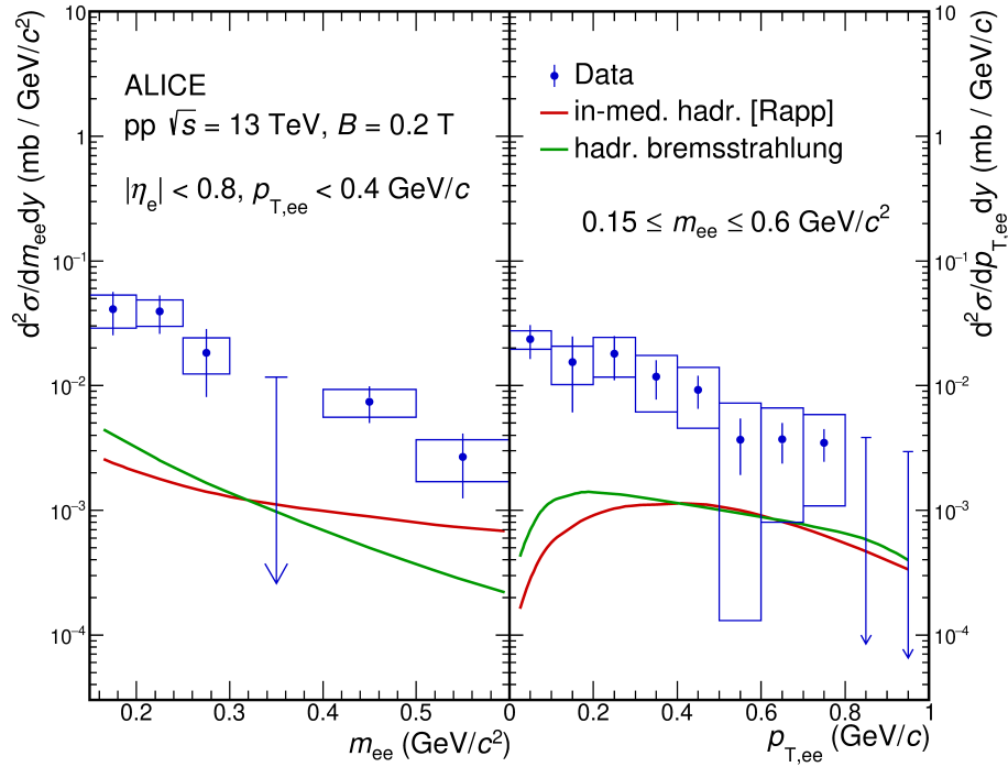
Figure 4: Dielectron excess spectra as a function of m_{ee} (left) and p_{T,ee} (right) after subtraction of the hadronic decay cocktail. The error bars and boxes represent statistical and combined systematic uncertainties from data and cocktail. Arrows indicate upper limits at 90% confidence level. Also shown as lines are calculations of bremsstrahlung from initial- and final-state hadrons [72], and thermal dielectron production [73–75].
