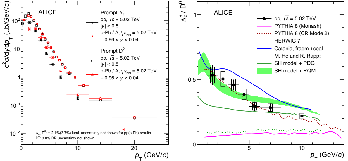
Fig. 1: Left: Prompt \Lambda_c^+ and D^0 p_T -differential cross section in pp collisions and in p–Pb collisions at \sqrt{s_{NN}} = 5.02 TeV. The results in p–Pb collisions are scaled with the atomic mass number A of the Pb nucleus. Right: the \Lambda_c^+/D^0 ratio as a function of p_T measured in pp collisions at \sqrt{s} = 5.02 TeV compared with theoretical predictions (see text for details). Statistical uncertainties are shown as vertical bars, while systematic uncertainties are shown as boxes, and the bin widths are shown as horizontal bars.
