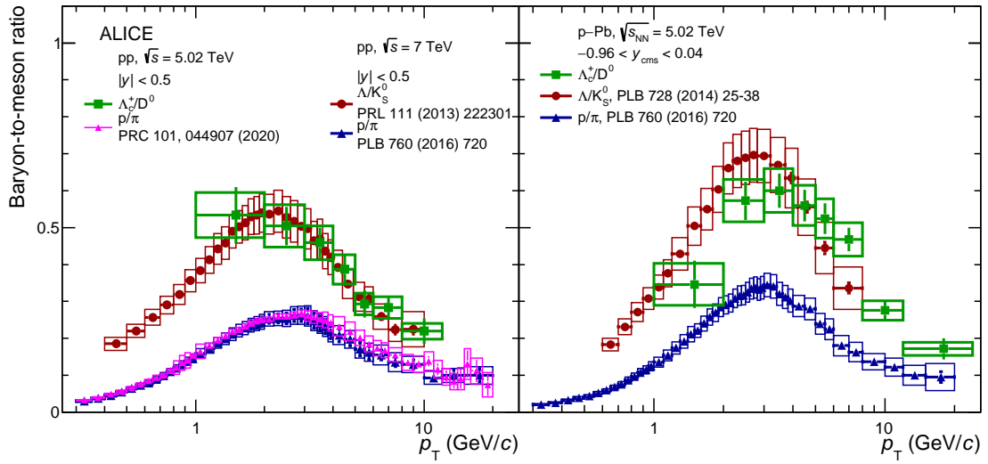
Fig. 2: The charm baryon-to-meson ratio \Lambda_c^+/D^0 in pp collisions (left), and p–Pb collisions (right) at \sqrt{s_{NN}} = 5.02 TeV, compared to the light-flavour baryon-to-meson ratios \Lambda/K_S^0 and p/\pi . Statistical uncertainties are shown as vertical bars, while systematic uncertainties are shown as boxes, and the bin widths are shown as horizontal bars.
