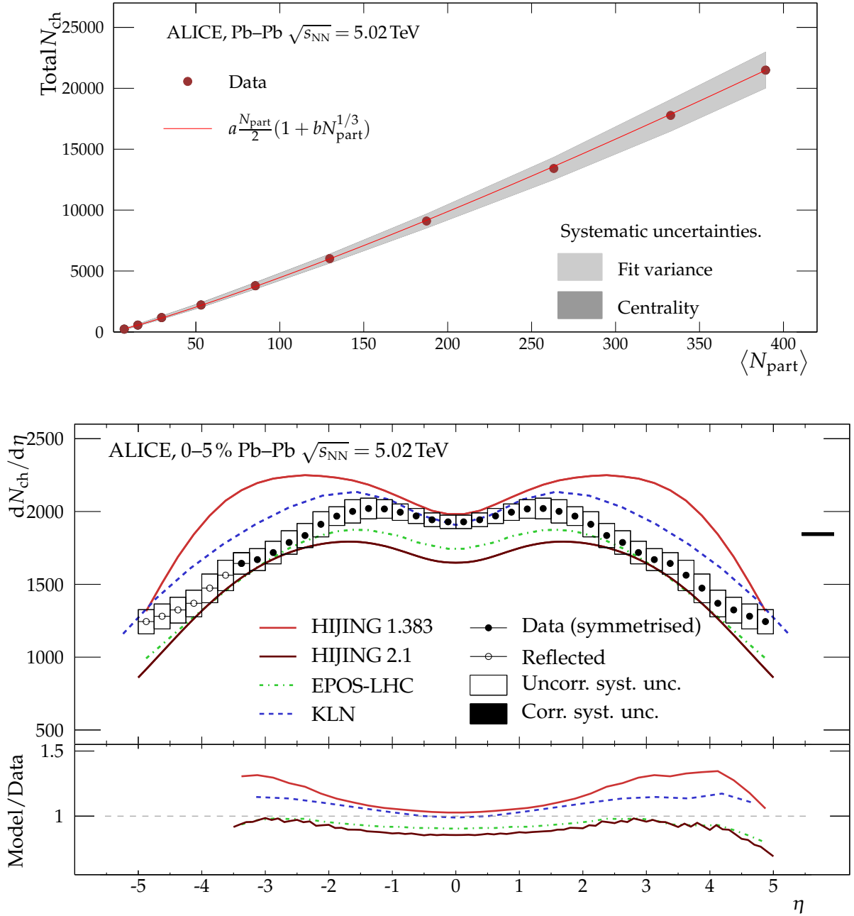
Figure 2: [Colour online] Comparison of dN_{\text{ch}}/d\eta in the 0–5% (0–6% for KLN) most central collisions of two versions of HIJING, KLN, and EPOS-LHC model calculations to the measured distribution.
