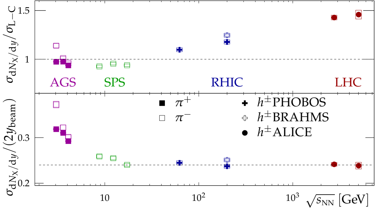
Figure 5: [Colour behaviour as a function \sqrt{s_{\text{NN}}} of the width of the charged-particle or -pion rapidity-density distribution with respect to the Landau–Carruthers width (top) and rapidity range (bottom). Charged-pion points from AGS and SPS up to RHIC are adapted from the literature [32], while the PHOBOS (filled crosses) [33] and BRAHMS (open crosses) [29] charged-hadron points are translated from the corresponding dN_{\text{ch}}/d\eta results.
