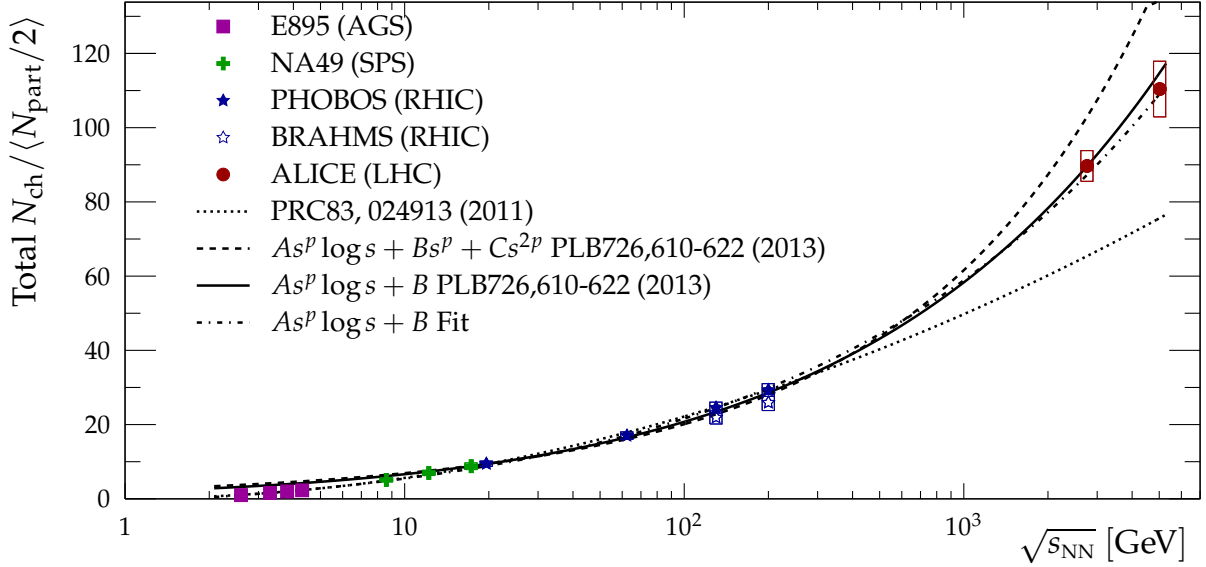
Figure 3: [Colour a function of \sqrt{s_{\text{NN}}} for the most central collisions at AGS (0–5 % Au–Au) [24, 25], SPS (0–5 % Pb–Pb) [26, 27], RHIC (0–5 % and 0–6 % Au–Au) [17, 28, 29], and LHC (0–5 % Pb–Pb) [13]. The dotted, dashed, and full lines are extrapolations from fits to lower energy results [13], while the dash-dotted line is a fit over all energies, including \sqrt{s_{\text{NN}}} = 5.02 TeV.
