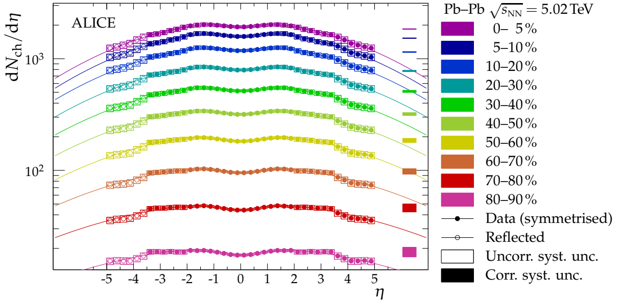
Figure 1: [Colour Charged-particle pseudorapidity density for ten centrality classes over a broad \eta range in Pb–Pb collisions at \sqrt{s_{\text{NN}}} = 5.02 TeV. Boxes around the points reflect the total uncorrelated systematic uncertainties and statistical errors, while the filled squares on the right reflect the correlated systematic uncertainty (evaluated at \eta = 0 ). Statistical errors are generally insignificant. Also shown is the reflection of the 3.5 < \eta < 5 values around \eta = 0 (open circles). The line corresponds to fits of the difference between two Gaussians centred at \eta = 0 ( f_{\text{GG}} ) [7] to the data.
