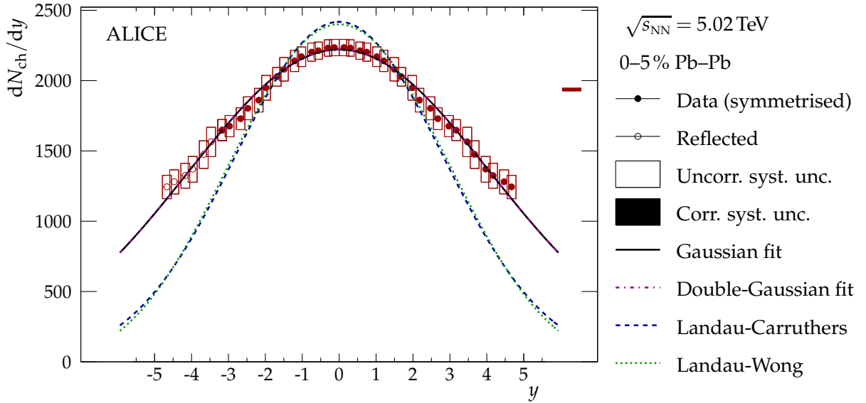
Figure 4: [Colour most central (0–5%) Pb–Pb collisions at \sqrt{s_{\text{NN}}} = 5.02 TeV. Also shown are the Landau–Wong [30], Landau–Carruthers [31], Gaussian, and double–Gaussian distributions.
