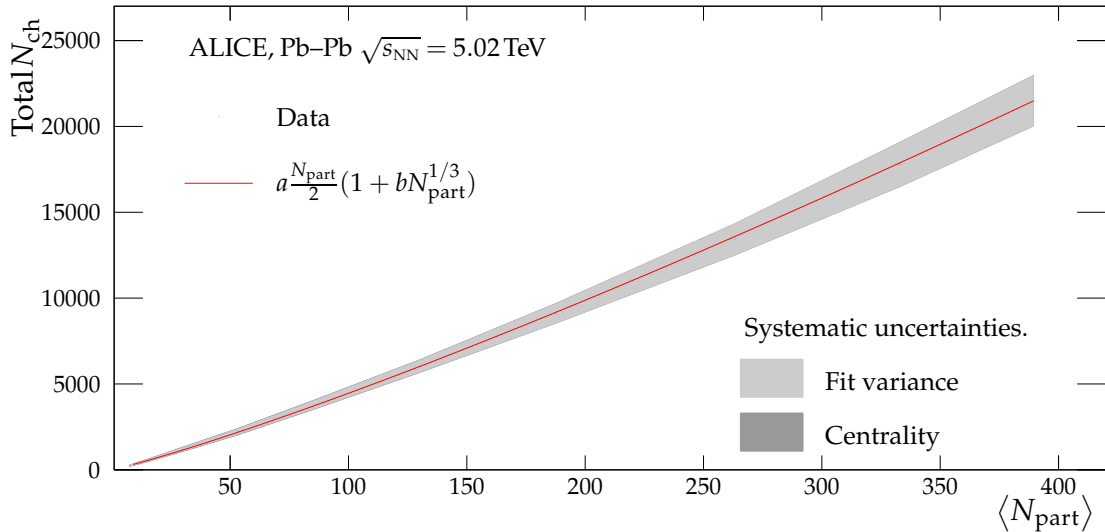
Figure 2: [Colour online] Total number of charged particles as a function of the mean number of participating nucleons [10]. The total charged-particle multiplicity is given as the integral over dN_{\text{ch}}/d\eta over the measured region ( -3.5 < \eta < 5 ) and extrapolations from fitted functions in the unmeasured regions. The contribution from unmeasured \eta regions amounts to \approx 30\% of the total number of charged particles. The uncertainty on the extrapolation to the unmeasured pseudorapidity region is smaller than the size of the markers. The contribution to the systematic uncertainties from the centrality determination and electromagnetic processes are vanishing compared to the contribution from the largest differences between the fitted functions. A function inspired by factorisation [17] is fitted to the data, and the best fit yields a = 51.5 \pm 7.3 , b = 0.16 \pm 0.05 .
