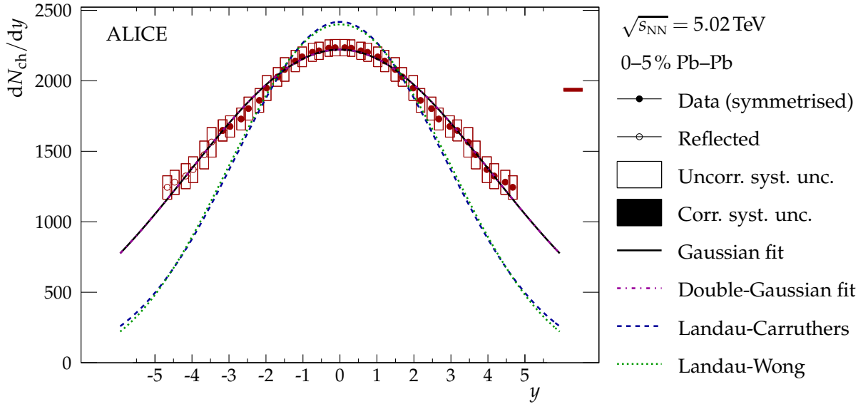
Figure 5: [Colour online] Estimate of dN_{\text{ch}}/dy in the most central (0–5%) Pb–Pb collisions at \sqrt{s_{\text{NN}}} = 5.02 TeV. Also shown are the Landau–Wong [30], Landau–Carruthers [31], Gaussian, and double–Gaussian distributions.
