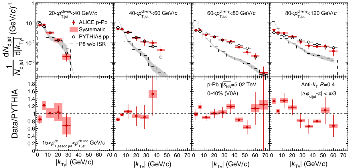
Fig. 1: Dijet |k_{Ty}| distributions in p–Pb collisions in the 0–40% V0A multiplicity event class for several kinematic intervals of the full jet ( p_{T,\text{jet}}^{\text{ch+ne}} ). The measurement is compared to PYTHIA8 (tune 4C, K = 0.7 ) with and without initial state radiation. The lower panels show the ratio between the measurement and PYTHIA8 including initial state radiation.
