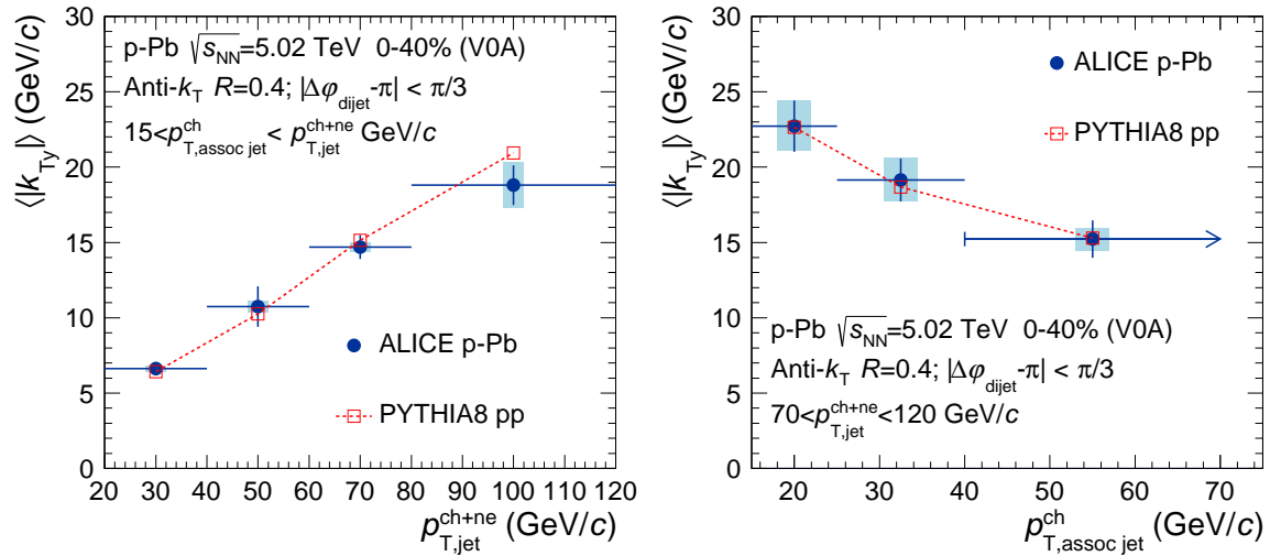
Fig. 3: Mean of the |k_{Ty}| distributions as a function of the full jet transverse momentum p_{T,\text{jet}}^{\text{ch+ne}} (left) and the associated charged jet transverse momentum p_{T,\text{assoc jet}}^{\text{ch}} (right) compared to PYTHIA8.
