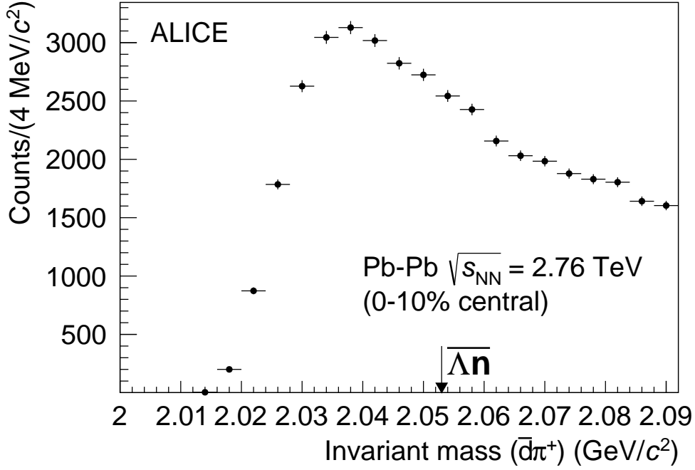
Fig. 2: Invariant mass distribution for \bar{d}\pi^+ for the Pb–Pb data corresponding to 19.3 \times 10^6 central events. The arrow indicates the sum of the mass of the constituents ( \bar{\Lambda}n ) of the assumed bound state. A signal for the bound state is expected in the region below this sum.
