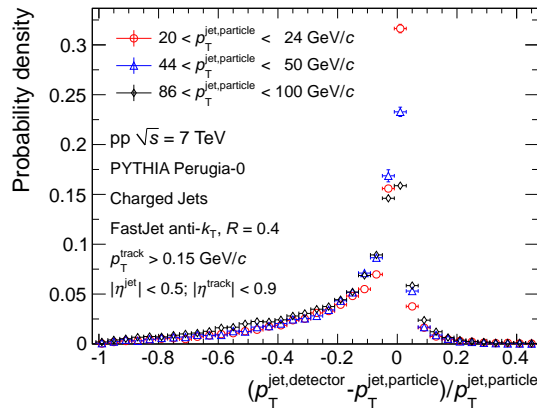
Fig. 1: (Color online) Probability distribution of the relative momentum difference of simulated ALICE detector response to charged jets in pp collisions at \sqrt{s} = 7 TeV for three different p_{\text{T}}^{\text{jet, particle}} intervals. Charged jets are simulated using PYTHIA Perugia-0 and reconstructed with the anti- k_{\text{T}} jet finding algorithm with R = 0.4 .
