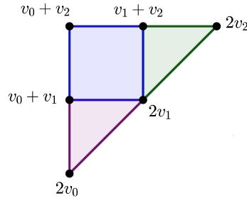
FIGURE 8. The space G_2 in Example 1.14
