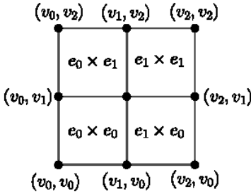
FIGURE 7. The space G^2 in Example 1.14
