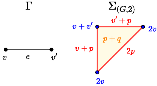
FIGURE 5. The graph \Gamma and the associated colored polysimplicial complex when d = 2
