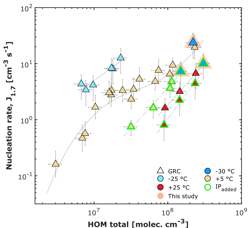
750 Figure 8. Pure biogenic nucleation rates at 1.7 nm diameter against total HOM concentration at different temperatures for \alpha -pinene and \alpha -pinene + isoprene systems. HOM total is defined as the sum of C5, C10, C15 and C20 carbon classes. Triangles represent Galactic Cosmic Rays (GCR) conditions. Data points at +5 °C and +25 °C are from Kirkby et al. (2016) and Heinritzi et al., (2020). Data points at -25 °C are from Simon et al., (2020). The value of isoprene-to-monoterpene carbon ratio (R) varies from 1.5 to 6.5 for Heinritzi et al., (2020), and R equals to 14.4 and 6.1 for this study. The points with orange marker on the background indicate the contribution of this work. Solid lines represent power-law fits to GCR conditions of the systems with \alpha -pinene only and dashed lines are the power-law fits of the systems with isoprene added. Bars indicate 1 \sigma run-to-run uncertainty. The overall systematic scale uncertainty of HOM of +78 % and -68 % and is not shown.
