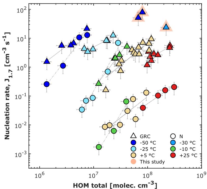
715 Figure 6. Pure biogenic nucleation rates of pure \alpha -pinene at 1.7 nm diameter against total HOM concentration at different 720 temperatures. HOM total is defined as the sum of C 5 , C 10 , C 15 and C 20 carbon classes. Triangles represent galactic cosmic rays (GCR) conditions and circles represent Neutral conditions. Data points at -50 °C, -25 °C, -10 °C, +5 °C and +25 °C are from Simon et al. (2020). The points with orange marker on the background are the contribution of this study (experiments \alpha -30,20, \alpha -50,20 and \alpha - 50,60-100). Solid and dashed lines represent power-law fits to GCR and Neutral conditions. Bars indicate 1 \sigma run-to-run uncertainty. The overall systematic scale uncertainty of HOM of +78 % and -68 % and is not shown.
