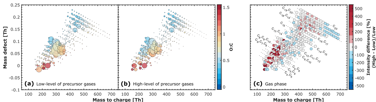
735 Figure 7. Mass defect plots of gas phase for two different systems and the normalized difference between them. Gas phase is measured with a Nitrate CI-APi-TOF Mass Spectrometer, (a) \alpha -pinene oxidation products at -10\text{ }^{\circ}\text{C} and 90 % RH at low-level of precursor gases, (b) \alpha -pinene oxidation products at -10\text{ }^{\circ}\text{C} and 80 % RH at high-level of precursor gases. \alpha -pinene was 0.2 - 0.8 ppbv and Ozone \sim 40 - 50 ppbv in (a), and \alpha -pinene was 2 - 3 ppbv and Ozone \sim 100 ppbv in (b). The symbol sizes and colors in (a) and (b) represent the intensities normalized by the total signal in each system. (c) The difference between the normalized signals shown in (a) and (b) is represented by the color scale.
