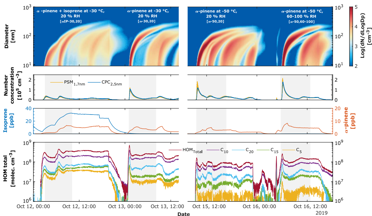
655 Figure 1. Experimental overview for pure biogenic new particle formation. First panel: particle size distribution for four different experiments: \alpha -pinene + isoprene at -30\text{ }^{\circ}\text{C} and 20\text{ }\% RH ( \alpha IP-30,20); \alpha -pinene at -30\text{ }^{\circ}\text{C} and 20\text{ }\% RH ( \alpha -30,20); \alpha -pinene at -50 ^{\circ}\text{C} and 20\text{ }\% RH ( \alpha -50,20) and \alpha -pinene at -50\text{ }^{\circ}\text{C} and 60\text{-}100\text{ }\% RH ( \alpha -50,60-100). The color scale represents the log 10 of the normalized particle concentration in \text{cm}^{-3} . Second panel: Particle number concentration in \text{cm}^{-3} measured by the PSM with a cut- 660 off diameter of 1.7\text{ nm} and CPC 2.5\text{ nm} . Third panel: Mixing ratio in ppbv for the biogenic precursor gases, isoprene and \alpha -pinene. Fourth panel: Evolution of total HOM concentration in \text{molec. cm}^{-3} , measured in the gas phase by the Nitrate CI-API-TOF mass spectrometer. HOM total is defined as the sum of \text{C}_5 , \text{C}_{10} , \text{C}_{15} and \text{C}_{20} carbon classes which are shown as well. Ozone level is not shown, though remains stable over the whole period \sim 100\text{ ppbv} . The shaded areas refer to the time where the particles were collected using the TD-DMA.
