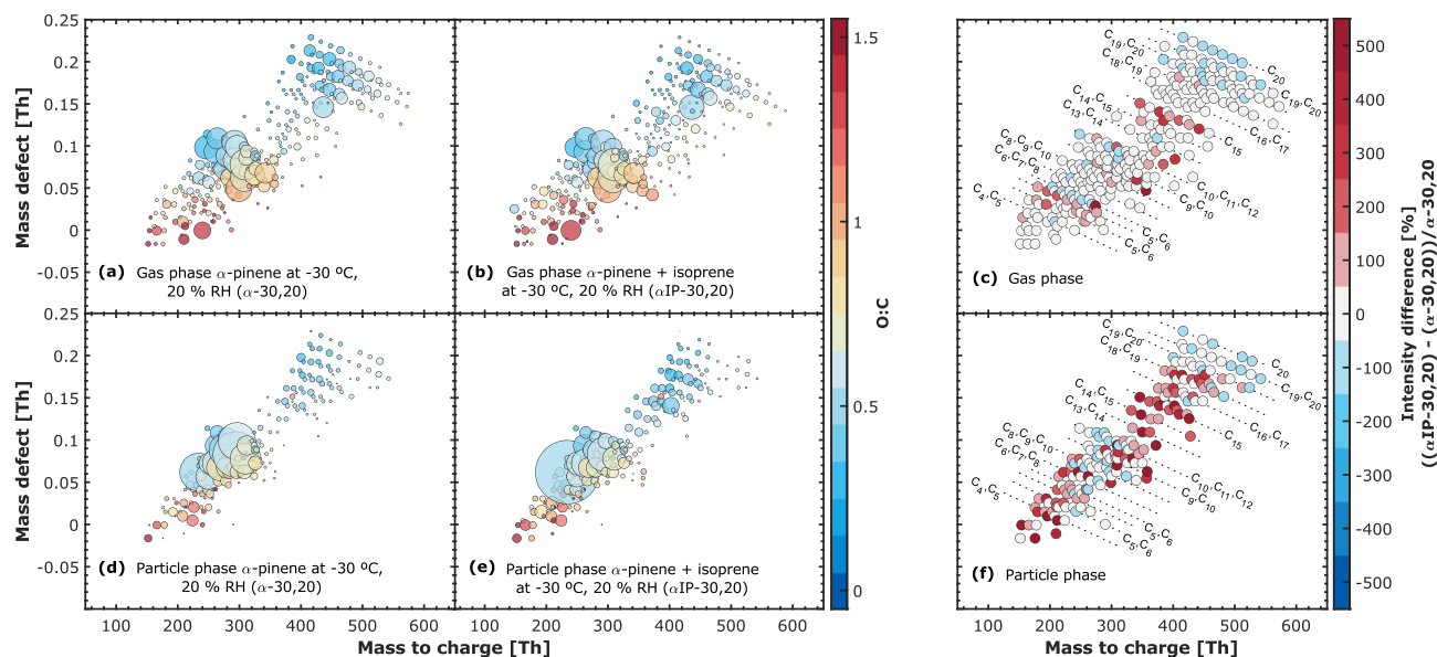
Figure 3. Mass defect plots of gas and particle phase and the intensity difference between them. Both phases are measured with a Nitrate CI-API-TOF Mass Spectrometer, while the TD-DMA is coupled to it for particle phase measurements. (a) gas and (d) particle for \alpha -pinene oxidation products at -30\text{ }^{\circ}\text{C} and 20\text{ }\% RH ( \alpha -30,20). (b) gas and (e) particle for \alpha -pinene + isoprene oxidation products at -30\text{ }^{\circ}\text{C} and 20\text{ }\% RH ( \alpha IP-30,20). The level of \alpha -pinene was between 1 and 8 ppbv in both experiments, while isoprene was present only in experiment \alpha IP-30,20 reaching up to 30 ppbv. Ozone levels were \sim 100 ppbv in both experiments. The symbol sizes in (a), (b), (d) and (e) are the intensities normalized by the total signal in each system. The intensity difference in gas (c) and in particle (f) is indicated as ((\alpha IP-30,20) - ( \alpha -30,20)) / \alpha -30,20. The color scale represents the difference in percent.
