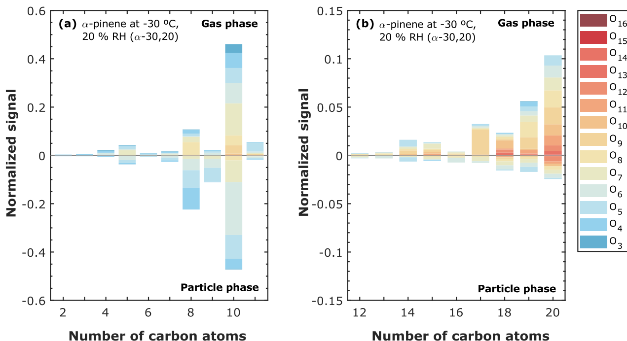
670 Figure 2. Carbon atom distribution and oxygen atom content in gas and particle phase molecules for \alpha -pinene oxidation products at -30 °C and 20 % RH ( \alpha -30,20). Both phases are measured with a Nitrate CI-APi-TOF Mass Spectrometer, while the TD-DMA is coupled to it for particle phase measurements. (a) carbon atom distribution C 2-11 and (b) carbon atom distribution C 12-20 . The level of \alpha -pinene was between 1 and 8 ppbv and Ozone level was stable at ~ 100 ppbv. The intensities are normalized by the total signal in each system. Each color represents a specific number of oxygen atoms in the range of 3 to 16.
