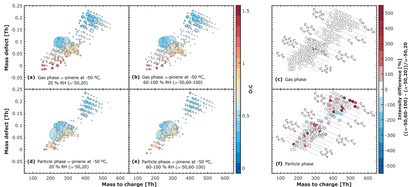
685 Figure 4. Mass defect plots of gas and particle phase and the intensity difference between them. Both phases are measured with a Nitrate CI-API-TOF Mass Spectrometer, while the TD-DMA is coupled to it for particle phase measurements. (a) gas and (d) particle for \alpha -pinene oxidation products at -50 °C and 20 % RH ( \alpha -50,20). (b) gas and (e) particle for \alpha -pinene oxidation products at -50 °C and 60 to 100 % RH ( \alpha -50,60-100). The level of \alpha -pinene was between 1 and 8 ppbv and Ozone levels were ~ 100 ppbv in both 690 experiments. The symbol sizes in (a), (b), (d) and (e) are the intensities normalized by the total signal in each system. The intensity difference in gas (c) and in particle (f) is indicated as ((\alpha -50,60-100) - ( \alpha -50,20)) / \alpha -50,20. The color scale represents the difference in percent.
