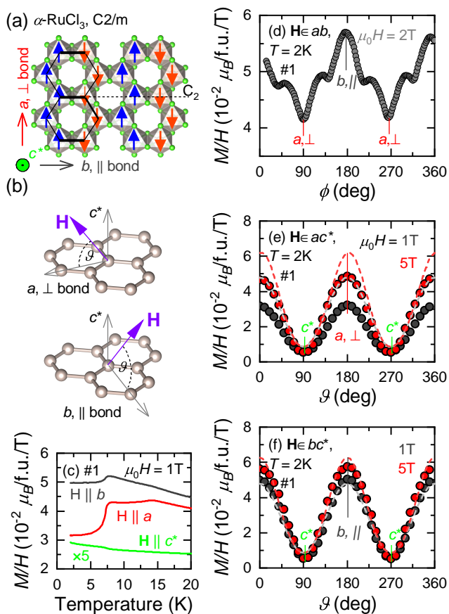
FIG. 1. (Color online) (a) Single honeycomb layer of \alpha -RuCl 3 and the crystallographic axes ( a , b , and c^* ). We highlight two directions within the ab plane; the a axis is perpendicular ( \perp bond) and the b axis is parallel ( \parallel bond) to one of the Ru-Ru bonds, respectively. Red and blue arrows at the honeycomb sites indicate the zigzag domain with ordering wave vector \mathbf{Q} \parallel b . Dashed line indicates a C_2 rotation symmetry around an axis parallel to the b axis. (b) During the magnetization and magnetostriction measurements, the magnetic field ( \mathbf{H} ) was canted out of the ab plane by an angle of \vartheta , while the planar projection of the applied field was either along the a or b axis. (c) Temperature dependence of the magnetization for fields along the main crystallographic axes in the field cooling runs ( \mu_0 H = 1 T). Note, that the data for \mathbf{H} \parallel c^* is multiplied by a factor of 5 for better visibility. (d-e) Angular dependence of the magnetization at T = 2 K for fields rotated within the ab , ac^* , and bc^* planes, respectively. Measurement data is plotted with symbols (full circles) for \mu_0 H = 1 T and 5 T. In case of \mathbf{H} \in ab , the measurements are plotted for \mu_0 H = 2 T. Dashed curves in panels (e,f) correspond to the theoretical calculations.
