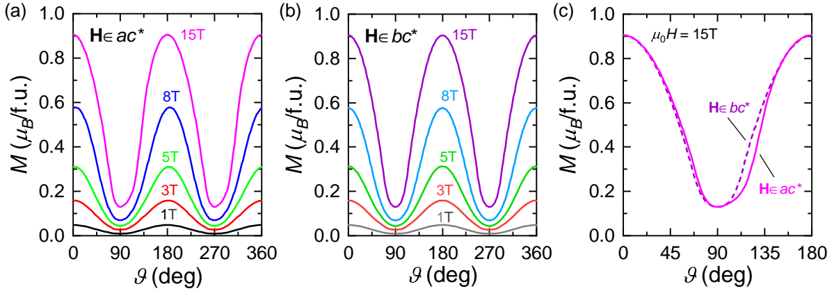
FIG. S4. (Color online) Theoretical calculations for the angular dependence of the magnetization for (a) \mathbf{H} \in ac^* and for (b) \mathbf{H} \in bc^* . In panel (c), we compare the angular dependency for \mathbf{H} \in ac^* and \mathbf{H} \in bc^* at \mu_0 H = 15 T.
