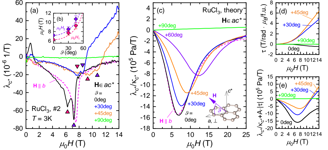
FIG. 3. (Color online) (a) Field dependence of the linear magnetostriction coefficient \lambda_{c^*} at T=3\text{K} . The magnetic field was applied along the main crystallographic axes, as well as canted out of the ab plane with projection perpendicular to the bond ( \mathbf{H} \in ac^* ). The \vartheta=0\text{deg} and 90\text{deg} angles correspond to the a and c^* axes, respectively. The two peaks in the \lambda_{c^*} data correspond to (\mu_0H_1) a phase transition between different zigzag interplane orderings and (\mu_0H_2) a transition into the field-induced quantum paramagnetic phase. The \mu_0H_1 and \mu_0H_2 phase boundaries are indicated by triangles, respectively. (b) Angular dependence of the \mu_0H_1 and \mu_0H_2 phase transition fields. The dashed lines indicate the \sim 1/\cos\vartheta field dependence. (c) The field dependence of the \lambda_{c^*}/\kappa_{c^*} magnetostriction calculated for H field canted out of the ab plane with \vartheta angle, \mathbf{H} \in ac^* . The inset defines the field angle \vartheta . Note, that panels (a) and (c) are shown for different field scales. (d) Magnetic field dependence of the calculated \tau magnetic torque for selected \vartheta canting angles, \mathbf{H} \in ac^* . (e) The effect of magnetic torque on the field-dependence of the magnetostriction is modelled with the \lambda_{c^*}/\kappa_{c^*} + A \cdot |\tau| relation with the same A=2.2 \cdot 10^5 \text{ Pa} \cdot \text{Rad} / (\text{T}^2 \cdot \mu_B/\text{f.u.}) parameter fitted for each curve.
