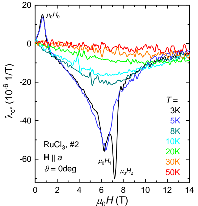
FIG. 2. (Color online) Magnetic field dependence of the \lambda_{c^*} linear magnetostriction coefficient at selected temperatures. The \Delta L length change was measured along the c^* axis and \mathbf{H} \parallel a magnetic field was applied, perpendicular to one of the Ru-Ru bonds.
