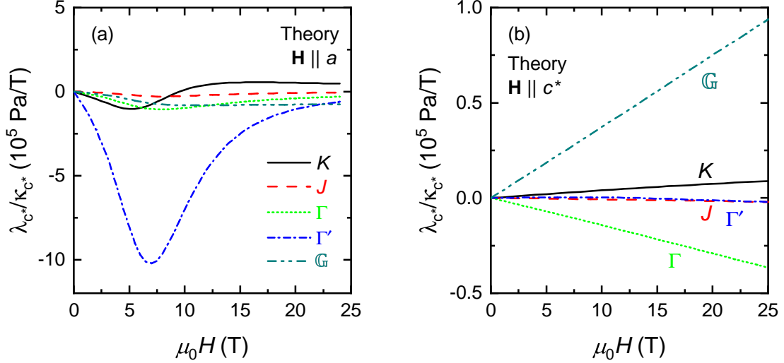
FIG. 4. (Color online) Dissection of the largest contributions to theoretical magnetostriction through Eq. (5). Each curve correspond to a component of Eq. (5) with different \mathcal{J} . The notation K , J , \Gamma , \Gamma' , and \mathbb{G} corresponds to the summand components of \frac{1}{V}\tilde{K}(\frac{\partial M}{\partial K}) , \frac{1}{V}\tilde{J}(\frac{\partial M}{\partial J}) , \frac{1}{V}\tilde{\Gamma}(\frac{\partial M}{\partial \Gamma}) , \frac{1}{V}\tilde{\Gamma}'(\frac{\partial M}{\partial \Gamma'}) , and \frac{1}{V}\tilde{\mathbb{G}}(\frac{\partial M}{\partial \mathbb{G}}) , respectively. The line with \mathcal{J} = \mathbb{G} corresponds to magnetoelastic coupling with the g -tensor. (a) In-plane field \mathbf{H} \parallel a ( \vartheta = 0 deg), (b) Out-of-plane field \mathbf{H} \parallel c^* ( \vartheta = 90 deg).
