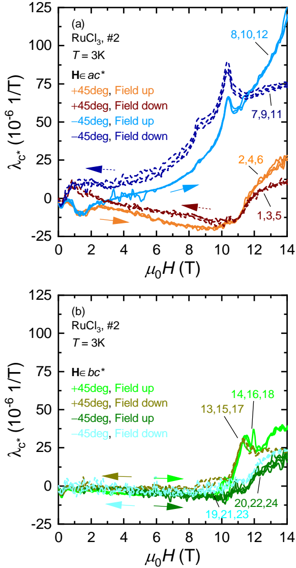
FIG. S1. (Color online) Magnetic field dependence of the \lambda_{c^*} linear magnetostriction coefficient at T=3K for the field-increasing and decreasing runs for field canted within the ac^* and bc^* planes ( \mathbf{H} \in ac^* and \mathbf{H} \in bc^* , respectively). For each setting, three measurements are shown, the numerals indicate the order of the measurements. The ab -plane projection of the canted magnetic field was set perpendicular and parallel to the Ru-Ru bonds, respectively in panels (a) and (b). The magnetic field was canted out of the ab plane in \vartheta = \pm 45^\circ angles.
