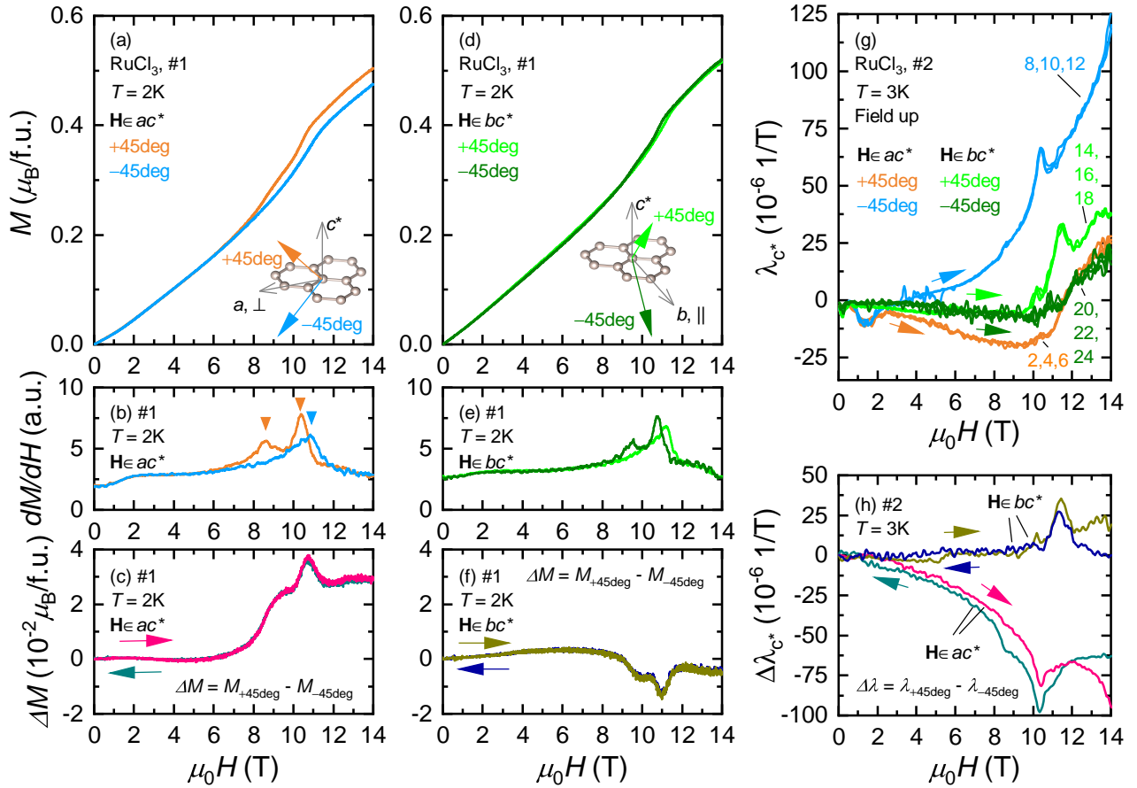
FIG. 5. (Color online) (a) Magnetic field dependence of the magnetization at T=2\text{K} for \mathbf{H} \in ac^* with \vartheta=\pm 45\text{deg} canting out of the ab plane. (b) Magnetic field dependence of the field-derivative, and (c) the field dependence of the \Delta M magnetization difference for the \vartheta=+45\text{deg} and -45\text{deg} measurements ( \Delta M=M_{+45\text{deg}} - M_{-45\text{deg}} ). The phase transitions for \mathbf{H} \in ac^* are indicated by triangles as peaks in dM/dH . (d-f) Magnetic field dependence of the magnetization, field derivative, and \Delta M at T=2\text{K} for \mathbf{H} \in bc^* , \vartheta=\pm 45\text{deg} . (g) Magnetic field dependence of the \lambda_{c^*} magnetostriction coefficient at T=3\text{K} for \mathbf{H} \in ac^* and \mathbf{H} \in bc^* measured in the field-increasing runs with \vartheta=\pm 45\text{deg} canting angles. Three \lambda_{c^*} - H curves are shown for each configuration, with numerals indicating the order of the measurements (complete list is shown in the supplementary material [75], Fig. S1). The experimental conditions are illustrated as an inset in panels (a) and (d). While panels (a,b,d,e,g) show measurements for the field-increasing runs, panels (c,f,h) show the measurements for the field increasing and decreasing runs.
