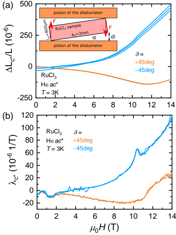
FIG. S2. (Color online) Magnetic field dependence of the \Delta L_{c^*}/L relative length change and the corresponding \lambda_{c^*} linear magnetostriction coefficient at T=3.0\text{K} for the field increasing runs. The magnetic field was canted out from the ab plane in \vartheta=\pm 45\text{deg} angles, perpendicular to the Ru-Ru bonds, \mathbf{H} \in ac^* . The inset of panel (a) illustrates the rotation of the sample within the dilatometer, where the rotation angle is \alpha \approx 0.08\text{deg} .
