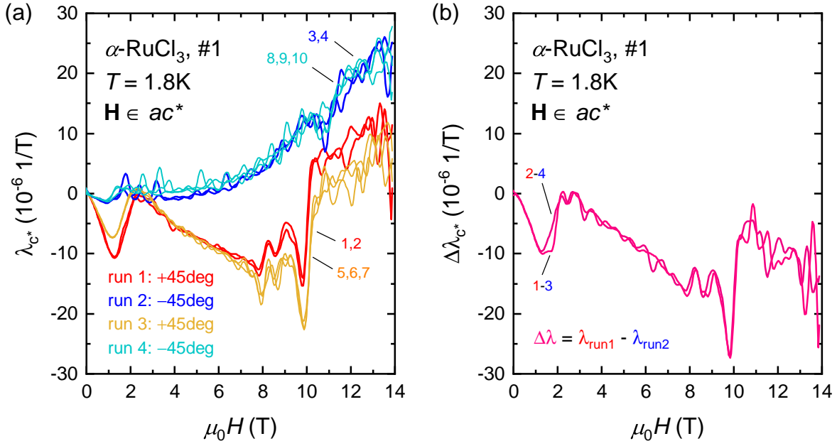
FIG. S3. (Color online) (a) Magnetic field dependence of the \lambda_{c^*} linear magnetostriction coefficient at T=1.8 K for sample #1. The magnetic field was canted out of the ab plane in \vartheta = \pm 45 deg angles, \mathbf{H} \in ac^* . During the measurement we changed the \vartheta canting angle in a +45 deg \rightarrow -45 deg \rightarrow +45 deg \rightarrow -45 deg sequence. Numerals indicate the order of the measurements. (b) Magnetic field dependence of the \Delta\lambda_{c^*} magnetostriction difference calculated from the measurements runs 1 and 2.
