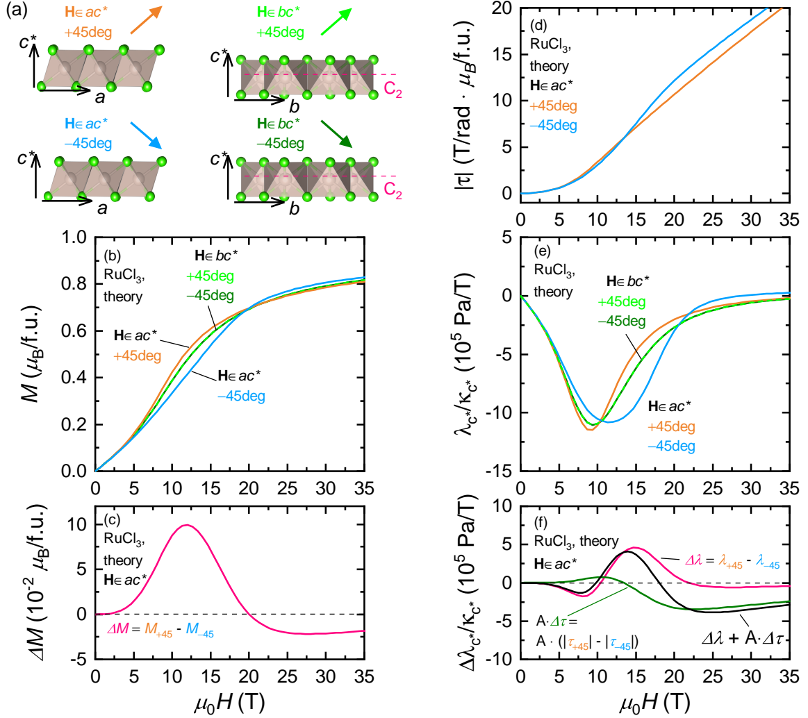
FIG. 6. (Color online) (a) Schematic illustration of the measurement configurations for each experiment. For \mathbf{H} \in ac^* , \vartheta = +45^\circ and \vartheta = -45^\circ , the net magnetization points along the vertexes and the edges of the \text{Cl}_6 octahedra, respectively. In both cases of \mathbf{H} \in bc^* , \vartheta = \pm 45^\circ , the net magnetization points along the side of the \text{RuCl}_6 octahedra, which configurations are connected by the C_2 rotation in the honeycomb plane. (b) Magnetic field dependence of the magnetization and (c) \Delta M magnetization difference calculated for \mathbf{H} \in ac^* and \mathbf{H} \in bc^* with \vartheta = \pm 45^\circ canting out of the ab plane. (d) Magnetic field dependence of the \tau magnetic torque for \mathbf{H} \in ac^* , \vartheta = \pm 45^\circ . (e) Magnetic field dependence of \lambda_{c^*}/\kappa_{c^*} magnetostriction and (f) \Delta\lambda_{c^*}/\kappa_{c^*} magnetostriction difference, calculated for \mathbf{H} \in ac^* and \mathbf{H} \in bc^* , \vartheta = \pm 45^\circ . The effect of the magnetic torque on the \Delta\lambda_{c^*}/\kappa_{c^*} magnetostriction difference is illustrated in panel (f), the torque is scaled to the unit of \lambda_{c^*}/\kappa_{c^*} with A = 2.2 \cdot 10^5 \text{ Pa} \cdot \text{Rad} / (\text{T}^2 \cdot \mu_B/f.u.) .
