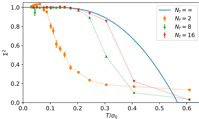
FIG. 15. \Sigma^2 as a function of T for \mu = 0 and N_f = 2, 8, 16, \infty (SLAC fermions, a \approx 0.410/\sigma_0 , N_s = 63 ).
