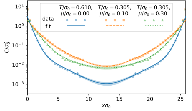
FIG. 14. The spatial correlation function C(x)/\sigma_0^2 for three different (\mu, T) in the symmetric phase and fits with A_1 \cosh(m_1(x - L/2)) + A_2 \cosh(m_2(x - L/2)) . We do not show data points in the region 9 \leq x\sigma_0 \leq 16 because of large systematic errors due to autocorrelations.
