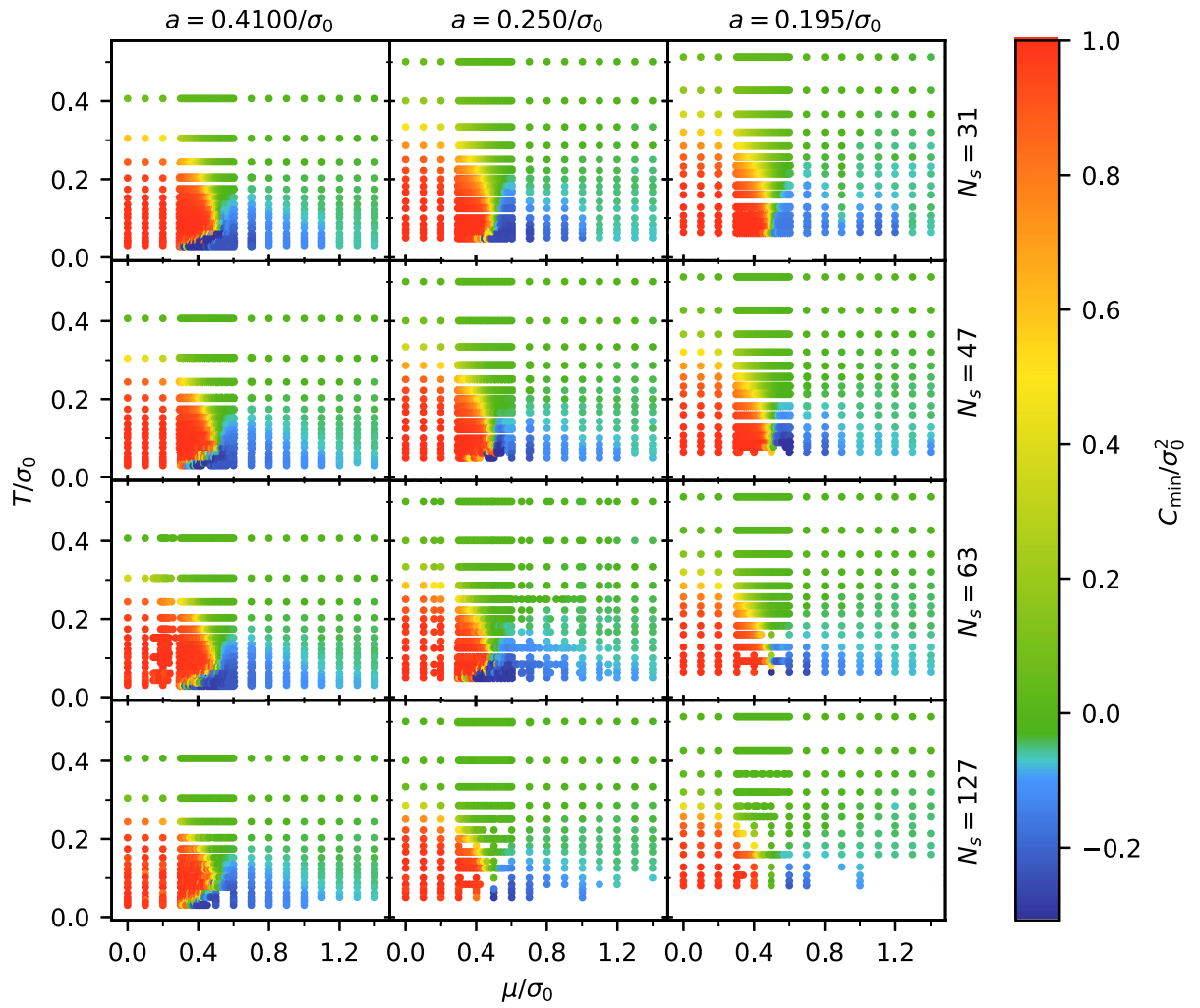
FIG. 8. C_{\min}/\sigma_0^2 in the \mu - T plane for three different values of the lattice spacing a (the columns) and four different numbers of lattice sites in spatial direction N_s (the rows) ( N_f = 8 , SLAC fermions).
