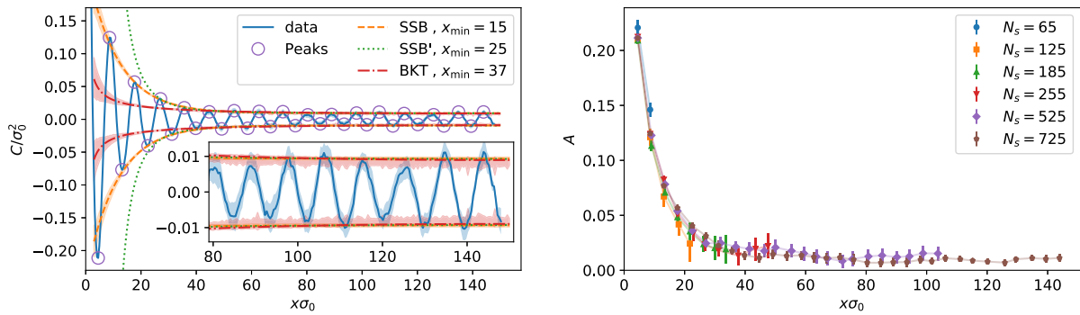
FIG. 12. The left plot shows the correlation function C(x)/\sigma_0^2 at (\mu/\sigma_0, T/\sigma) = (0.500, 0.030) for N_s = 725 , the extracted peaks and fits with the functions defined in Eqs. (65) and (66) (the parameters obtained by these fits are shown in Table II). For clarity interpolating lines are shown instead of the data points. The right plot shows the extracted peaks for N_s = 65, 125, 185, 255, 525, 725 .
