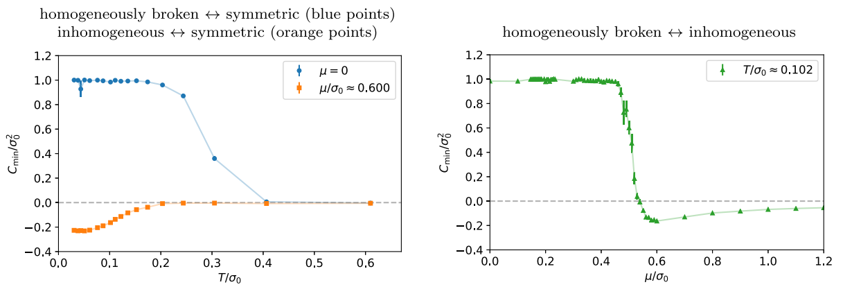
FIG. 9. C_{\min}/\sigma_0^2 as a function of T for \mu = 0 and for \mu/\sigma_0 \approx 0.600 (left plot) and C_{\min}/\sigma_0^2 as a function of \mu for T/\sigma_0 \approx 0.102 (right plot) ( N_f = 8 , SLAC fermions, a \approx 0.410/\sigma_0 , N_s = 63 ).
