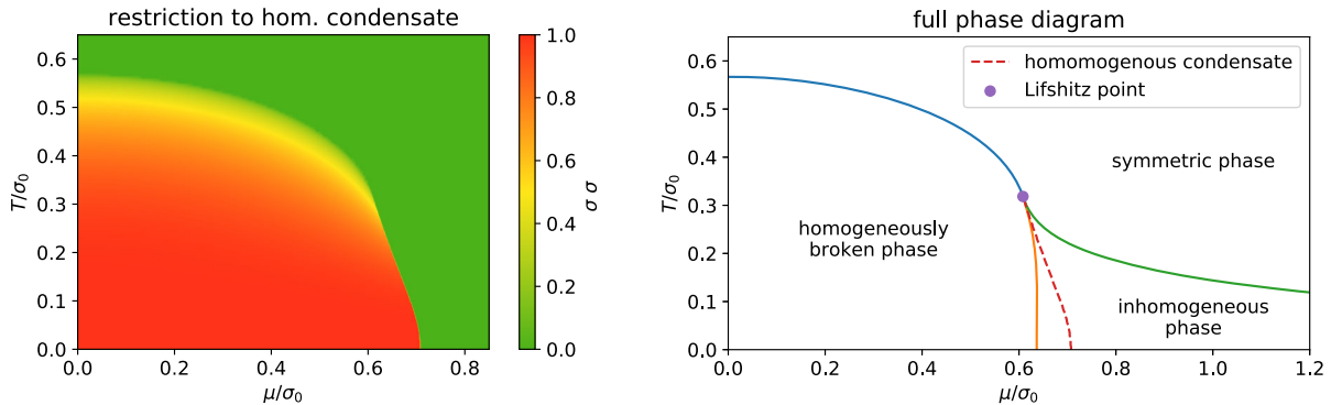
FIG. 1. (Left) The symmetric phase and the broken phase of the large- N_f GN model assuming a homogeneous condensate \sigma . The value of the condensate in units of \sigma_0 is color coded. For large temperature or large \mu chemical potential (the green region) the condensate vanishes. (Right) The corrected phase diagram of the large- N_f GN model with homogeneous and inhomogeneous condensates. The first order line from the Lifshitz point to T = 0 (red dashed line) obtained, when assuming a homogeneous condensate (see plot on the left side), turns into two second order lines (orange and green). In the region with large \mu and low T the condensate is inhomogeneous.
