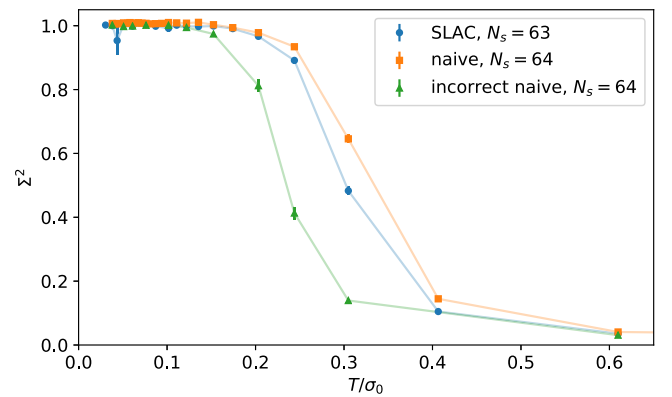
FIG. 16. \Sigma^2 as a function of T at \mu = 0 for SLAC fermions, naive fermions, and the straightforward but incorrect naive discretization (A9) ( N_f = 8 , a \approx 0.410/\sigma_0 ).
