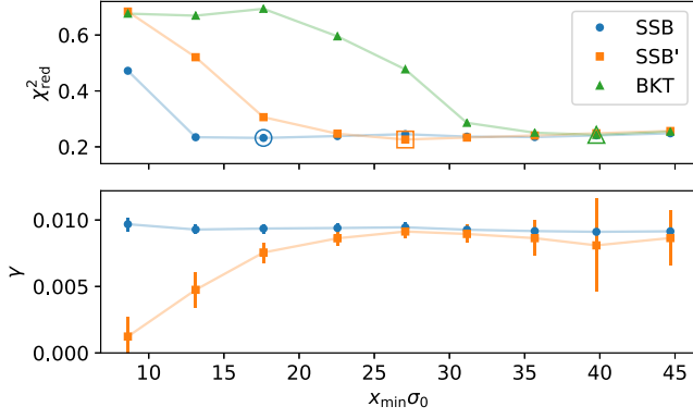
FIG. 13. Top: \chi_{\text{red}}^2 as a function of x_{\text{min}} for all three models ( N_s = 725 ). Bottom: Extracted parameters \gamma for the SSB and SSB' models as functions of x_{\text{min}} .
