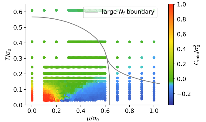
FIG. 10. C_{\text{min}}/\sigma_0^2 in the \mu - T plane for N_f = 2 . The red region corresponds to a homogeneously broken phase, the green region to a symmetric phase, and the blue region to an inhomogeneous phase. The grey lines represent the N_f \rightarrow \infty phase boundaries [8,9].
