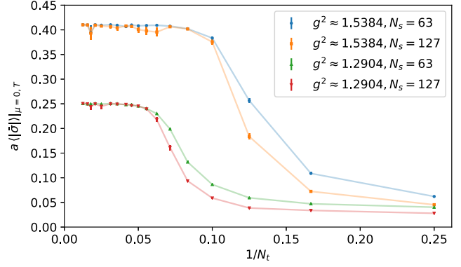
FIG. 3. a\langle|\bar{\sigma}|\rangle_{\mu=0,T} as a function of 1/N_t = Ta for \mu = 0 , N_f = 8 , SLAC fermions, two different g^2 , and two different N_s = L/a . The plateau values at small 1/N_t correspond to a\sigma_0 .
