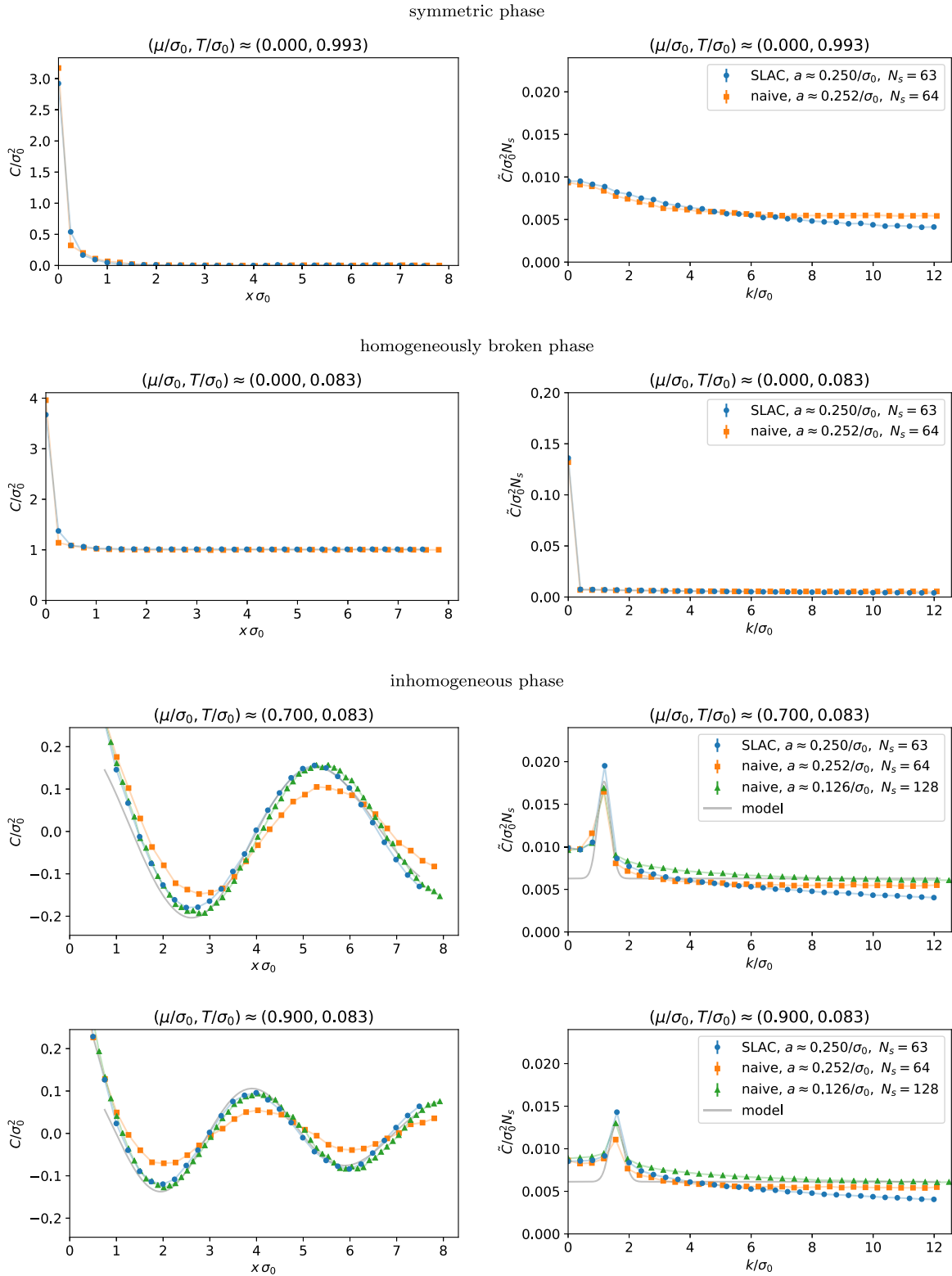
FIG. 6. The spatial correlation function C(x)/\sigma_0^2 (left column, where the x -range extends to half the box length) and its Fourier transform \tilde{C}(k)/\sigma_0^2 N_s (right column) for SLAC fermions (blue dots) and naive fermions (orange and green dots) in the symmetric, the homogeneously broken and the inhomogeneous phase ( N_f = 8 ) together with model expectations for the inhomogeneous phase [Eqs. (51) and (56); gray curves].
