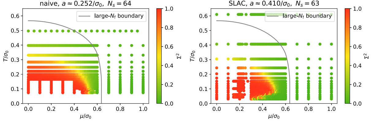
FIG. 5. \Sigma^2 in the \mu - T plane for naive fermions (left plot) and SLAC fermions (right plot) ( N_f = 8 ). The red regions correspond to a homogeneously broken phase and the green regions to a symmetric and/or an inhomogeneous phase. The gray lines represent the N_f \rightarrow \infty phase boundary of the homogeneously broken phase [8,9].
