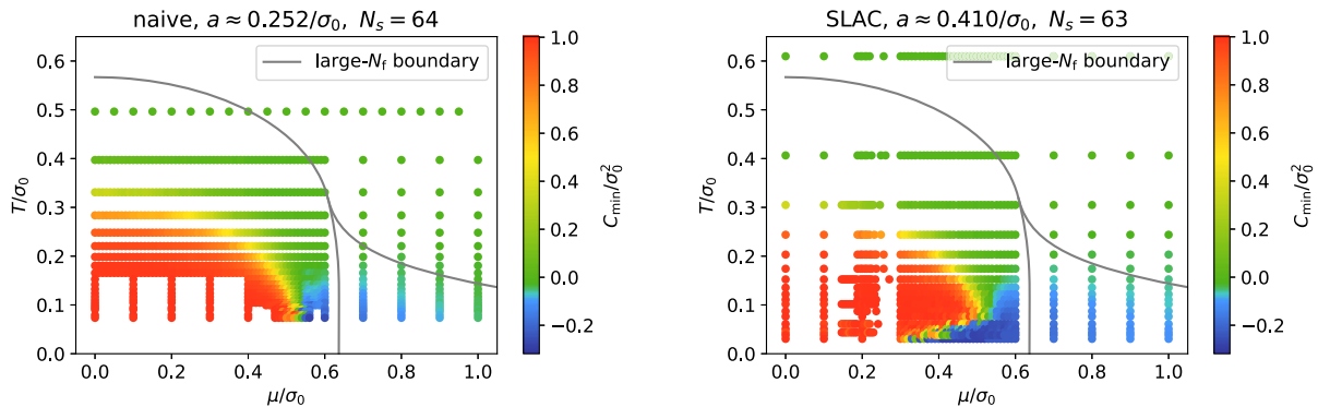
FIG. 7. C_{\min}/\sigma_0^2 in the \mu - T plane for naive fermions (left plot) and SLAC fermions (right plot) ( N_f = 8 ). The red regions correspond to a homogeneously broken phase, the green regions to a symmetric phase and the blue regions to an inhomogeneous phase. The gray lines represent the N_f \rightarrow \infty phase boundaries [8,9].
