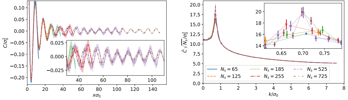
FIG. 11. The spatial correlation function C(x)/\sigma_0^2 (left) and its Fourier transform \tilde{C}(k)\sqrt{N_s}/\sigma_0^2 (right) at (\mu/\sigma_0, T/\sigma) = (0.500, 0.030) for N_f = 2 and N_s = 65, 125, 185, 255, 525, 725 . Except for the inset on the right, for clarity interpolating lines are shown instead of the data points.
