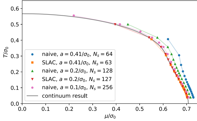
FIG. 2. N_f \rightarrow \infty phase diagram with the restriction to homogeneous condensate \sigma for naive and for SLAC fermions (three different lattice spacings, a \approx 0.41/\sigma_0, 0.20/\sigma_0, 0.10/\sigma_0 , similar spatial extent L ). The solid grey line represents the continuum result from Ref. [27].
