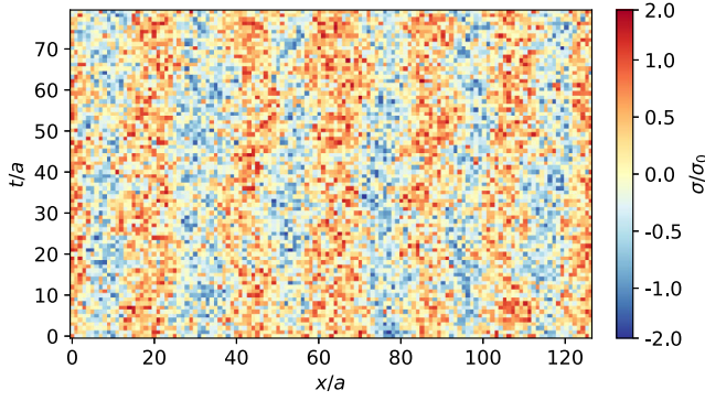
FIG. 4. A typical field configuration \sigma(\mathbf{x})/\sigma_0 generated by the HMC algorithm at large \mu/\sigma_0 \approx 0.450 and small T/\sigma_0 \approx 0.030 , where an inhomogeneous phase is expected ( N_f = 8 , SLAC fermions, a \approx 0.410/\sigma_0 , N_s = 127 ). The clearly visible vertical stripes indicate six oscillations in a spatial direction.
