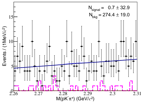
Figure 3. (color online) Fit to the M(pK^-\pi^+) distribution for the candidate events from \psi(3686) \rightarrow \Lambda_c^+\bar{\Sigma}^- . Points with error bars are data. The red (black) dashed line is the signal (background), and the blue solid curve is the total fit. The pink dashed line is the inclusive
