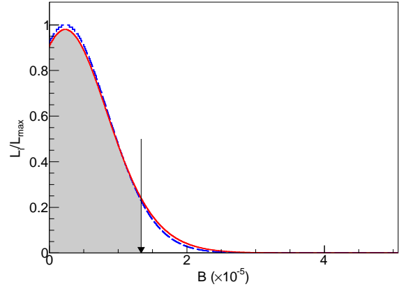
Figure 4. (color online) Distributions of the likelihoods versus the branching fraction of \psi(3686) \rightarrow \Lambda_c^+\bar{\Sigma}^- . The results obtained with and without incorporating the systematic uncertainties are shown in the red solid and blue dashed curves, respectively. The black arrow shows the result corresponding to the 90% confidence level.
