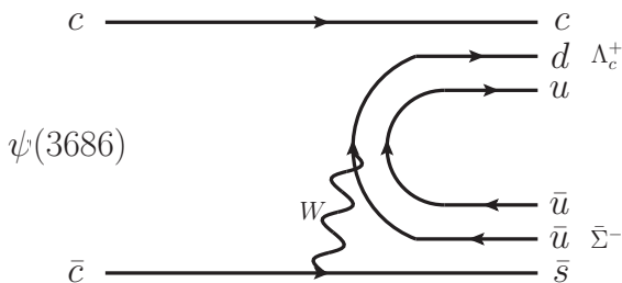
Figure 1. Feynman diagram for the process \psi(3686) \rightarrow \Lambda_c^+ \bar{\Sigma}^- in the SM[7].
