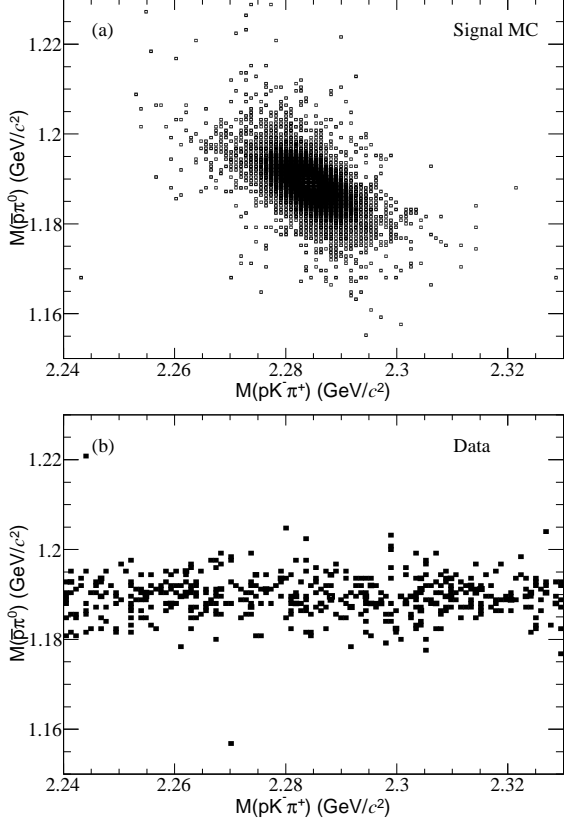
Figure 2. Distribution of M(\bar{p}\pi^0) versus M(pK^-\pi^+) for the accepted candidate events in the signal MC sample and data.
