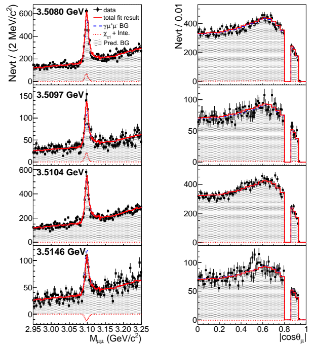
FIG. 2. One-dimensional projections of the two-dimensional fit to the M_{\mu^+\mu^-} and |\cos\theta_{\mu}| distributions from the \chi_{c1} scan samples. The black dots with error bars are the distributions from data, the gray histograms are the irreducible background predicted by the corrected MC simulation. The red curve is the best fit result, the red dotted (blue dashed) curve is the signal (background) contribution.
