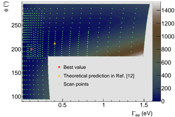
FIG. 1. The distribution of -\ln(L) in a larger parameter space region.
