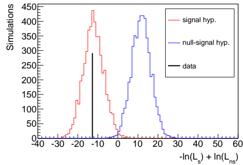
FIG. 8. Distribution of the test variable t from the toy MC samples using all four \chi_{c1} scan samples.
