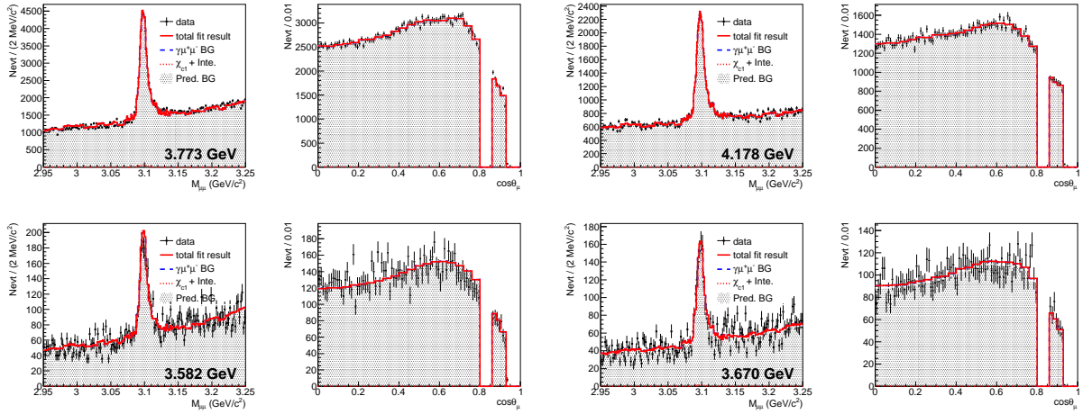
FIG. 5. One-dimensional projections of the two-dimensional fit to the M_{\mu^+\mu^-} and |\cos\theta_\mu| distributions from the control data samples. The two-dimensional correction factor is determined from \sqrt{s} = 4.178 GeV sample.
