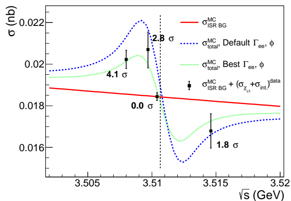
FIG. 1. Energy dependence of the cross section of the process e^+e^- \rightarrow \gamma J/\psi \rightarrow \gamma\mu^+\mu^- including (blue and green dashed lines) and not including (red solid line) the direct production of the \chi_{c1} and its interference with the irreducible background processes. The blue and green dashed lines show results from simulations in which the values of \Gamma_{ee} and \phi are set to those predicted in Ref. [13] and to those determined in this work, respectively. The location of the \chi_{c1} mass is indicated by the vertical line. The black dots with error bars represent \sigma_{\text{ISR BG}}^{\text{MC}} + (\sigma_{\chi_{c1}} + \sigma_{\text{int.}})^{\text{data}} at the \chi_{c1} scan data samples, where the background contribution \sigma_{\text{ISR BG}}^{\text{MC}} is taken from the PHOKHARA generator, and the \chi_{c1} production and interference contributions (\sigma_{\chi_{c1}} + \sigma_{\text{int.}})^{\text{data}} are determined from data. The numbers next to the four data points indicate the statistical significances of the \chi_{c1} and the contribution due to interference.
