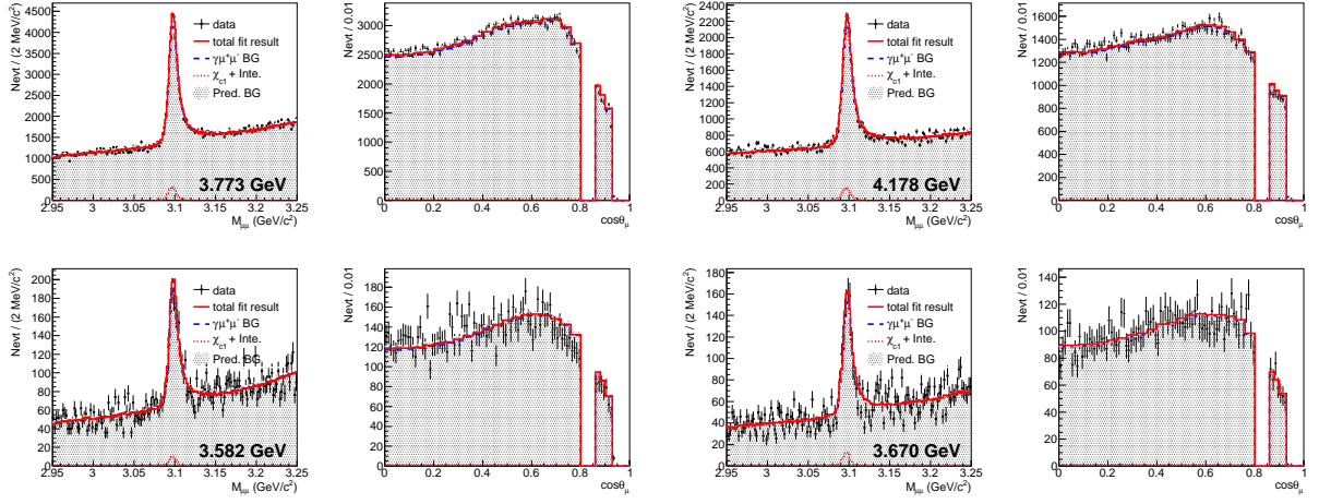
FIG. 3. One-dimensional projections of the two-dimensional fit to the M_{\mu^+\mu^-} and |\cos\theta_\mu| distributions from the control data samples. The two-dimensional correction is not applied in this fit. The black dots with error bars are the distributions from data, the gray histograms are the irreducible background predicted by the corrected MC simulation. The red curve is the best fit result, the red dotted (blue dashed) curve is the signal (background) contribution.
