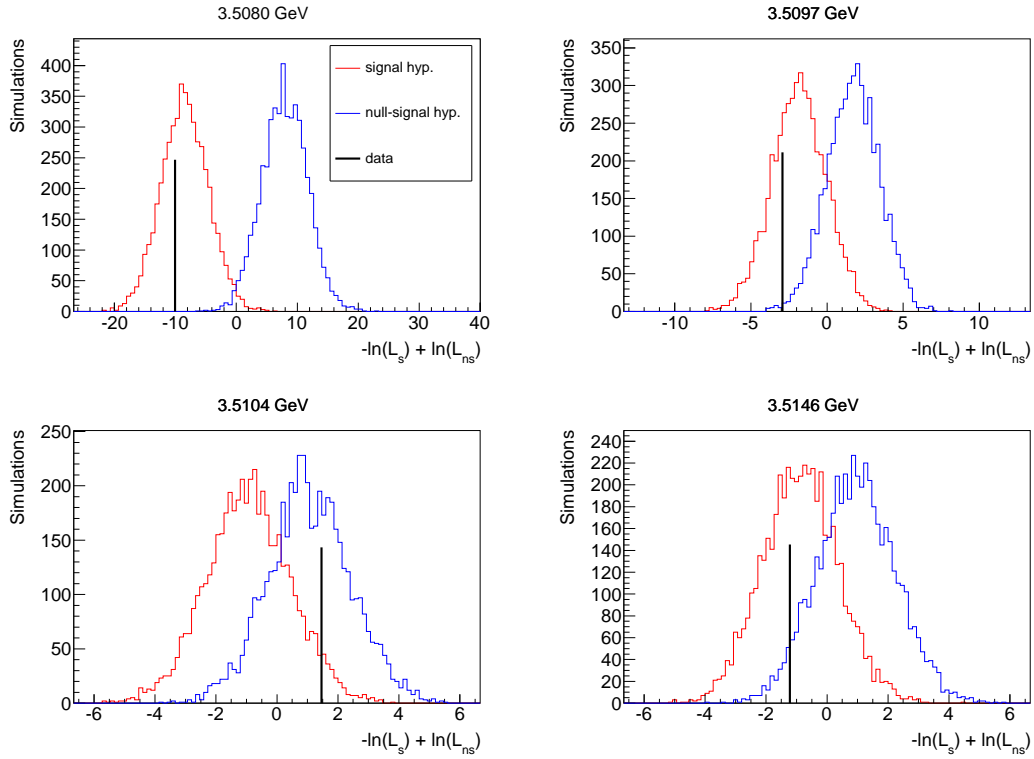
FIG. 7. Distributions of the test variable t from the toy MC samples based on the common fit result under the signal and null-signal hypotheses at \sqrt{s} = 3.5080, 3.5097, 3.5104, and 3.5146 GeV. The red and the blue histograms show the distributions under the signal and null-signal hypotheses, respectively, while the black vertical lines indicate the values from real data.
