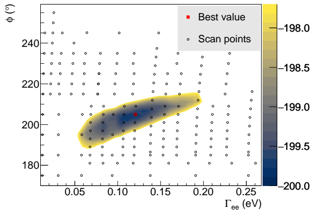
FIG. 3. The 68.3% C.L. contour of \Gamma_{ee} and \phi on a distribution of log-likelihood ( -\ln L ) values. The black open circles are the parameter points with which MC samples are produced. The red point (0.12 eV, 205.0°) represents the point where the likelihood value is maximum. The distribution of -\ln L in a larger parameter space region is shown in the supplemental material [20].
