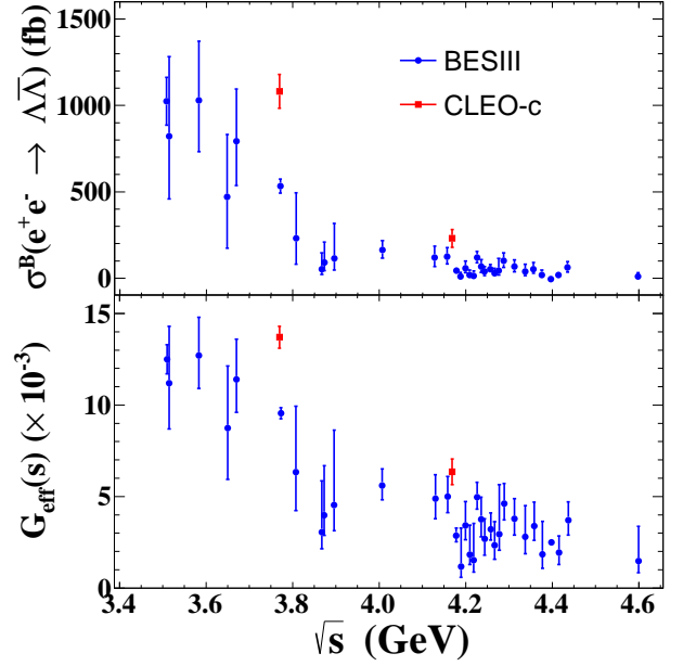
FIG. 2. The measured Born cross section (top) and \Lambda effective form factor (bottom) for e^+e^- \rightarrow \Lambda\bar{\Lambda} as a function of the c.m. energy, where the uncertainties include the statistical and systematic ones.
