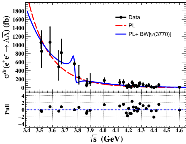
FIG. 3. The dressed cross section of the process e^+e^- \rightarrow \Lambda\bar{\Lambda} is represented by the dots with error bars, including statistical and systematic uncertainties. The red dashed line represents the fit with the power-law function only, while the solid blue line is for the fit with the power-law function and the \psi(3770) resonance. The bottom panel shows the pull distribution for the fit with the resonance.
