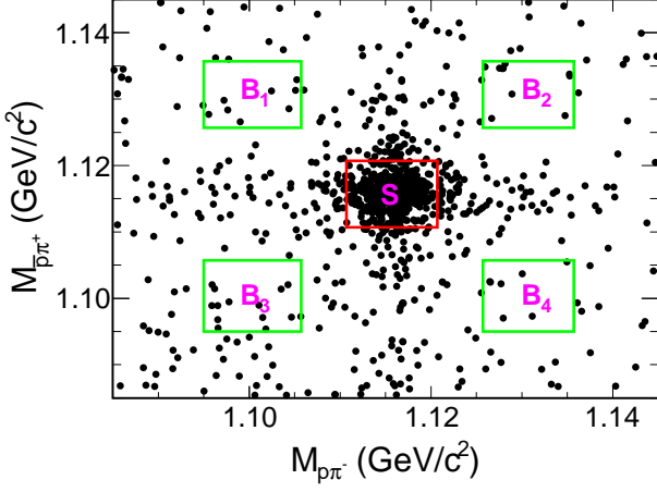
FIG. 1. Distribution of M_{p\pi^-} versus M_{p\pi^+} of the accepted candidates from all data samples, where the red box shows the signal region, the green boxes denote the selected sideband regions.
