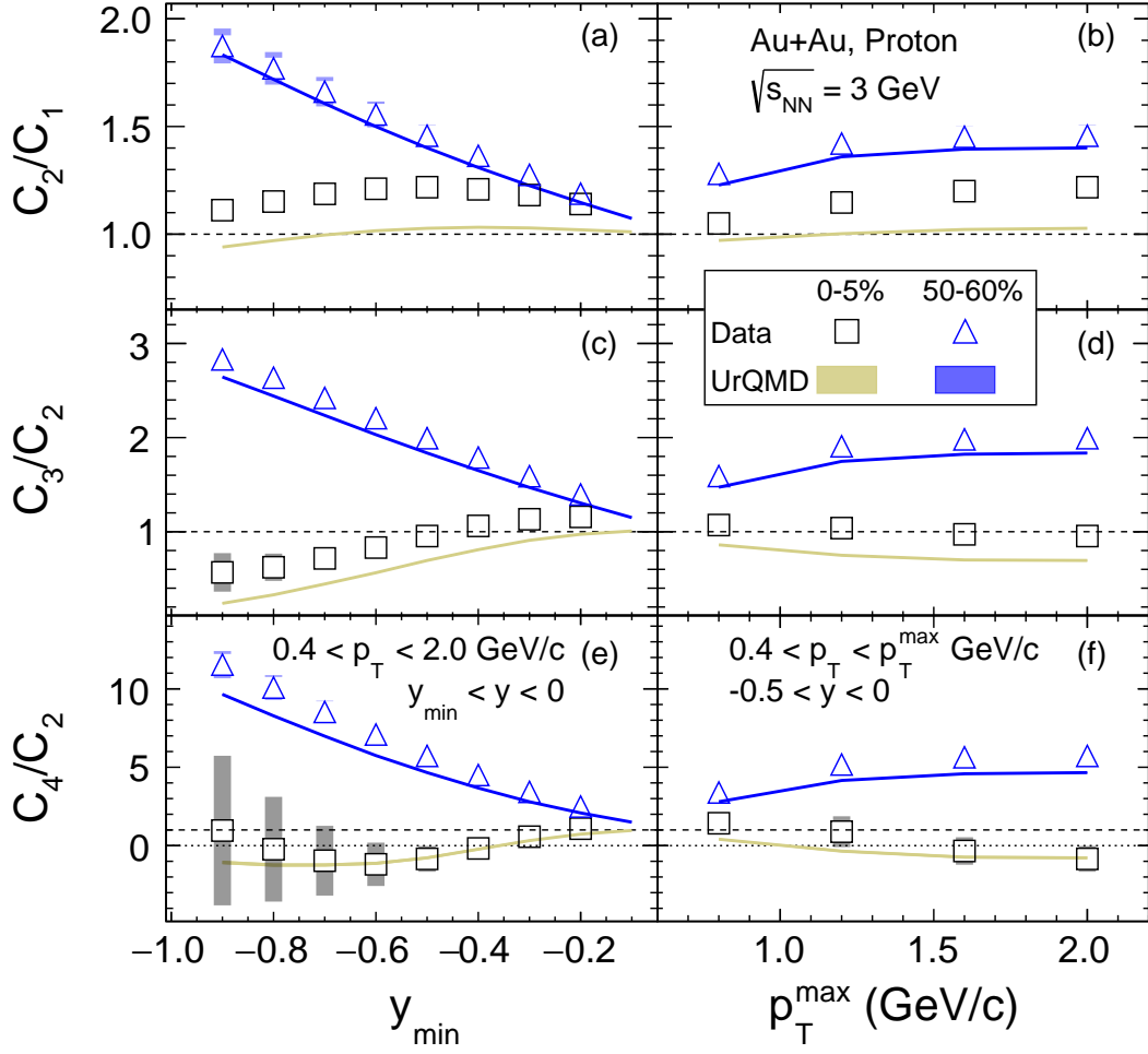
FIG. 18: The transverse-momentum and rapidity dependence of cumulant ratios of proton multiplicity distributions for Au+Au collisions at \sqrt{s_{\text{NN}}} = 3 GeV. In the left column, the p_{\text{T}} of the analysis window is 0.4 < p_{\text{T}} < 2.0 GeV/c while the rapidity window is varied in the range y_{\text{min}} < y < 0 . In the right column, the rapidity of the analysis window is -0.5 < y < 0 while the p_{\text{T}} is varied in the range 0.4 < p_{\text{T}} < p_{\text{T}}^{\text{max}} GeV/c. The most central (0-5%) and peripheral (50-60%) events are depicted by black squares and blue triangles, respectively. Statistical and systematic uncertainties are represented by black and gray bars, respectively. UrQMD simulations for the top 0-5% and 50-60% are shown by gold and blue bands, respectively.
