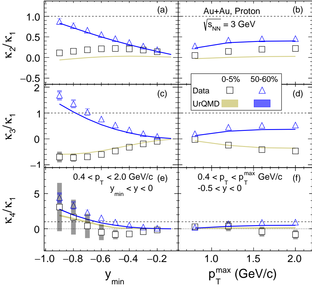
FIG. 19: As Fig. 18 but for transverse-momentum and rapidity dependence of correlation function ratios of proton multiplicity distributions for Au+Au collisions at \sqrt{s_{NN}} = 3 GeV.
