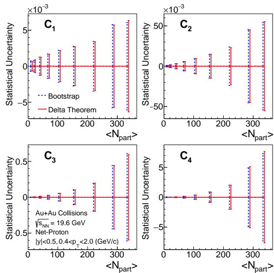
FIG. 10. (Color online) Comparison of the statistical uncertainties on C_n of net-proton distributions in Au+Au collisions at \sqrt{s_{\text{NN}}} = 19.6 GeV from the delta theorem and bootstrap methods. The results are presented as a function of \langle N_{\text{part}} \rangle .
