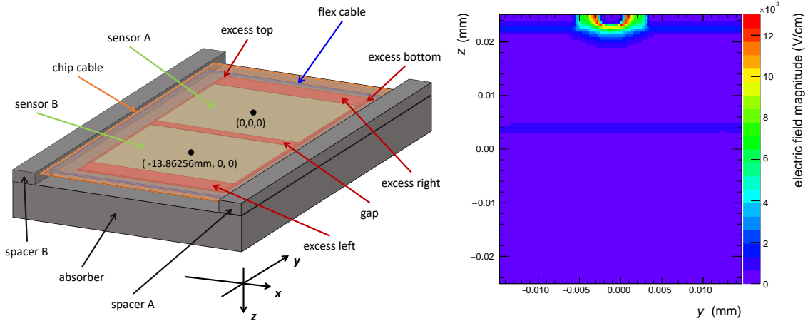
Figure 5: (left) Implementation of an EPICAL-2 layer in the Allpix 2 simulation. (right) Electric field magnitude in the sensor region corresponding to a single pixel as a function of y - and z -position relative to the simulation-internal origin.
