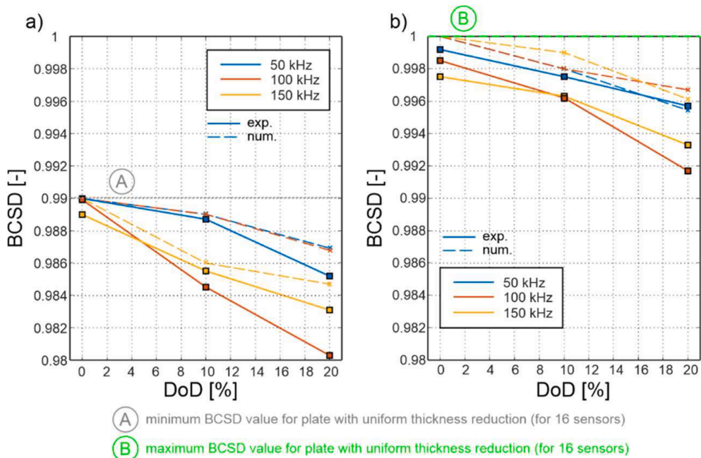
Fig. 28. Minimal and maximal values of BCSD functions determined for plates varying in DoD: a) minimum values of BCSD and b) maximum values of BCSD for variable frequencies.
