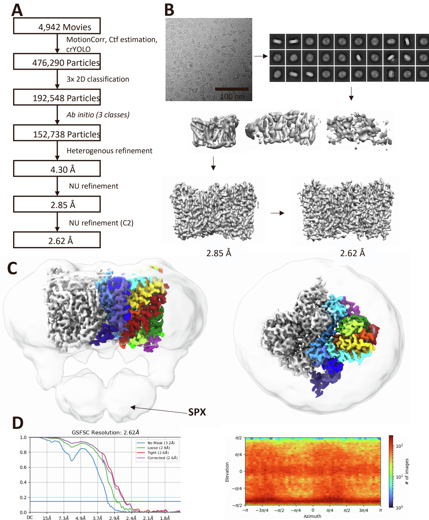
Figure S2: Cryo-EM processing of ScPho90 in the presence of phosphate, related to Figure 1
