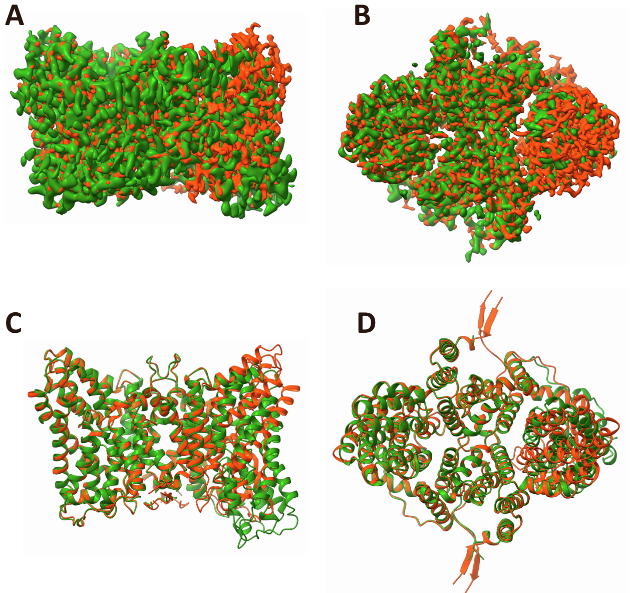
Figure S7: Comparison of phosphate-free ScPho90 maps and models, related to Figure 2
