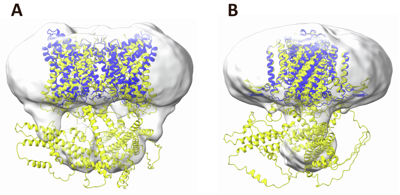
Figure S9: AlphaFold model of the SPX domain, related to Figure 5
