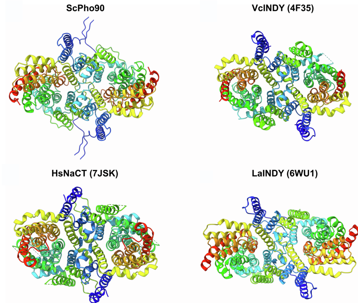
Figure S10: Structures of the DASS family, related to Figure 4
