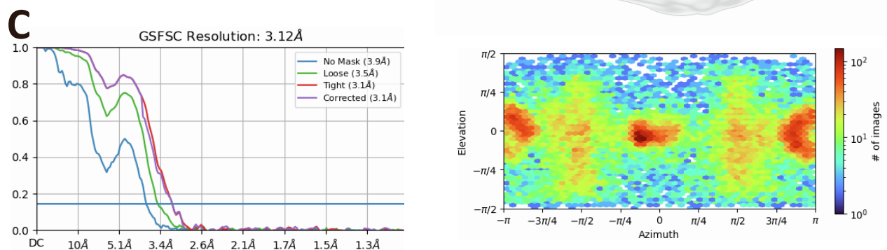
Figure S4: Cryo-EM processing of ScPho90 in the absence of phosphate (Part 2), related to Figure 1
