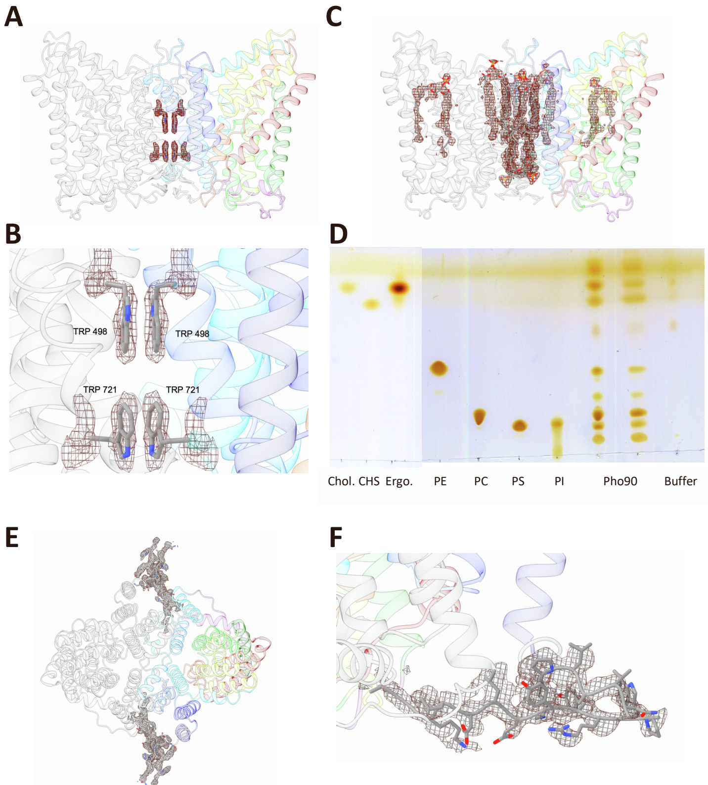
Figure S6: Details of the ScPho90 structure, related to Figure 3
