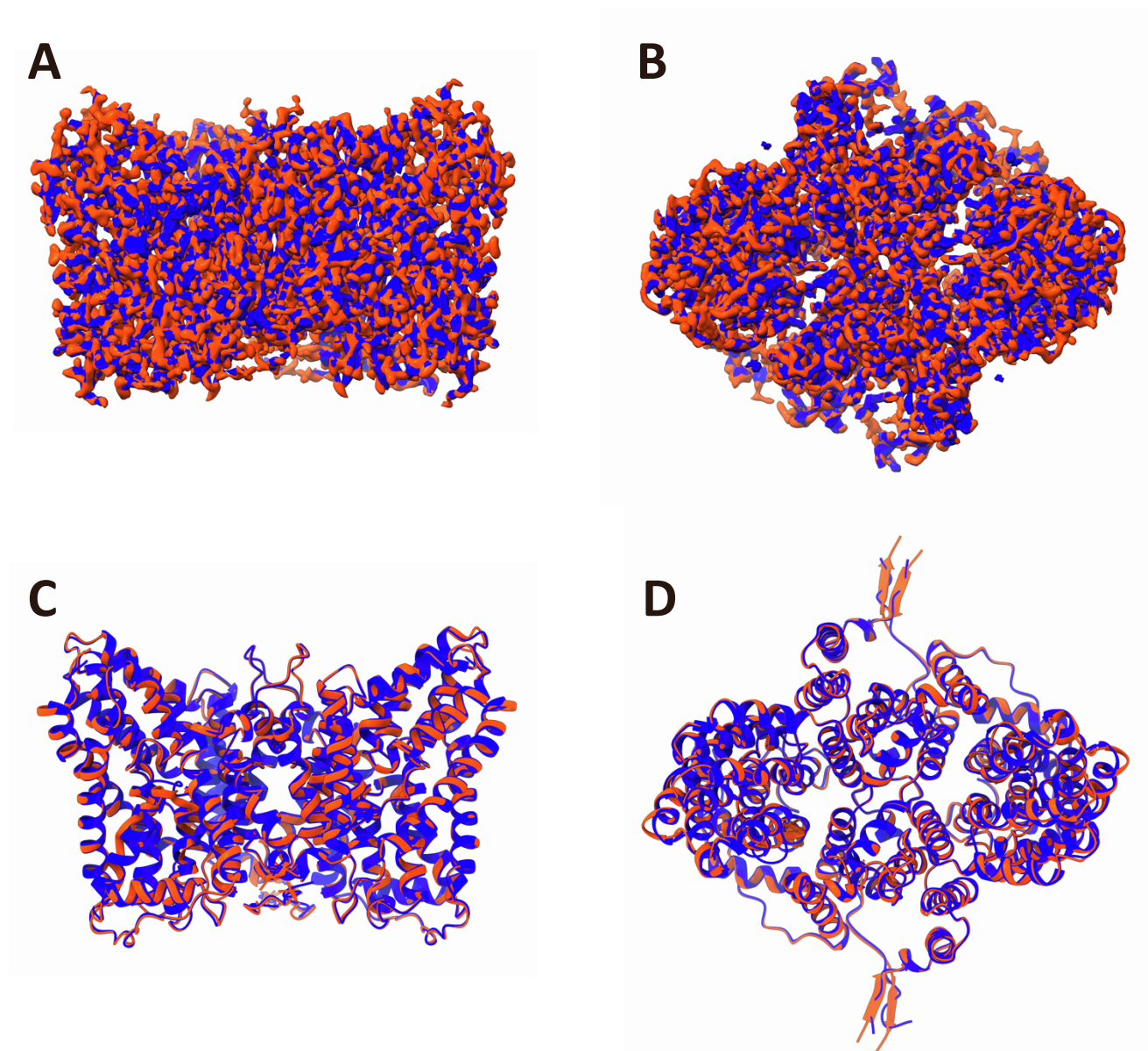
Figure S5: Comparison of symmetric ScPho90 maps and models, related to Figure 3
