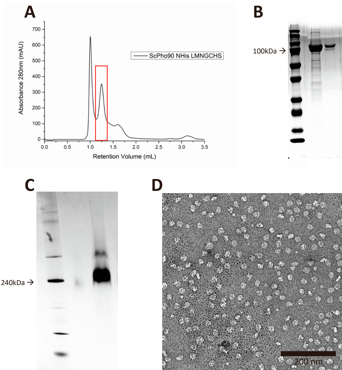
Figure S1: Purification and analysis of ScPho90, related to STAR Methods
