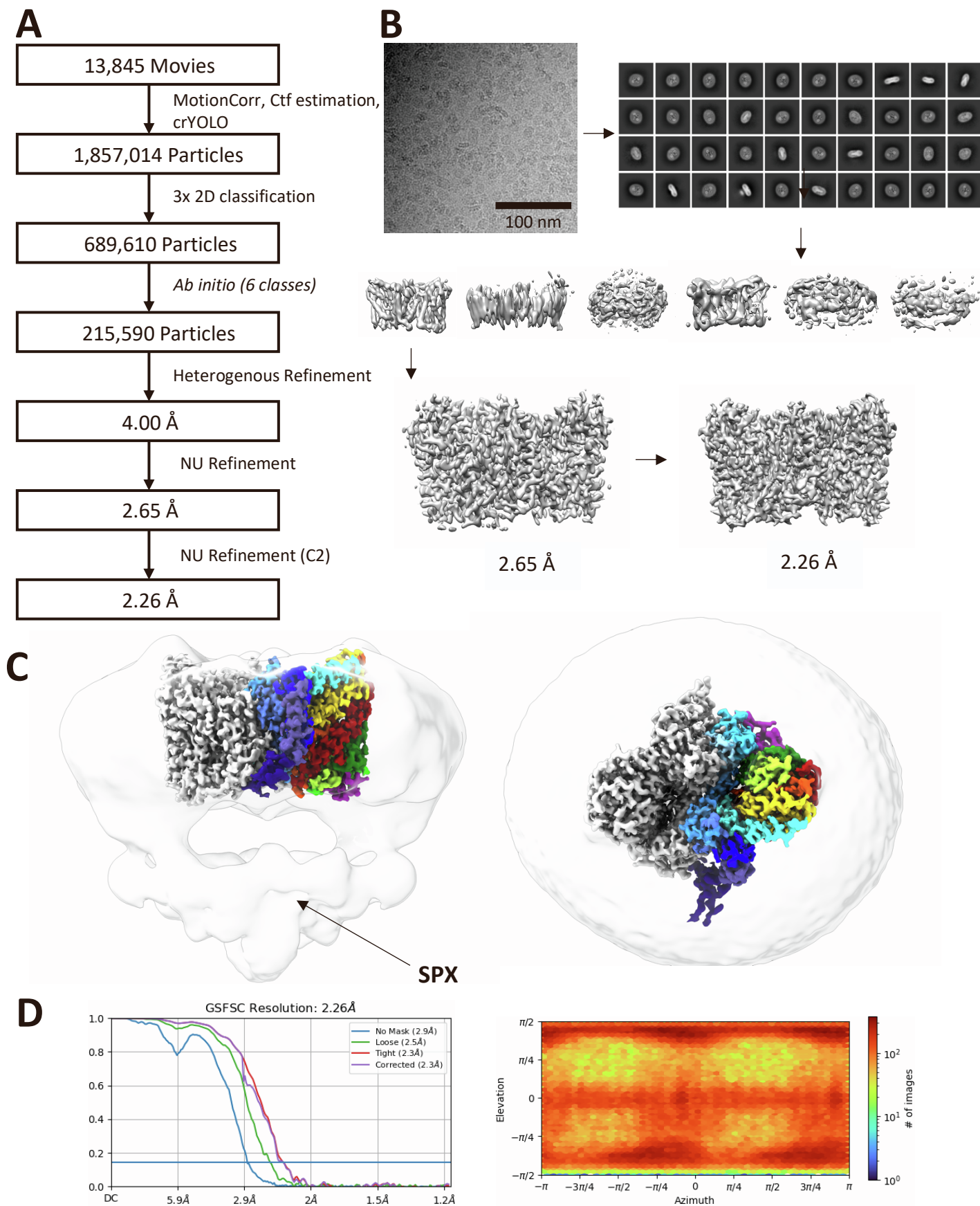
Figure S3: Cryo-EM processing of ScPho90 in the absence of phosphate (Part 1), related to Figure 1
